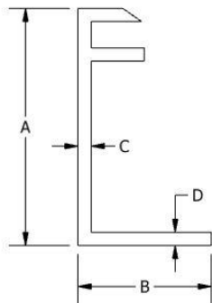
C-Shape Construction Minimum Requirements
