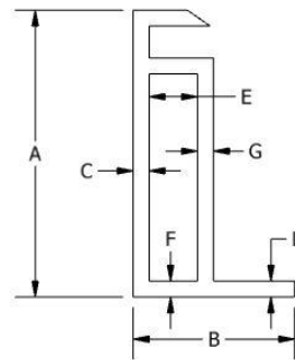
Box Shape Construction Minimum Requirements
