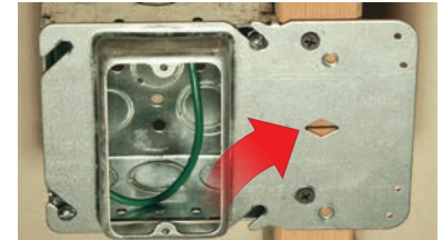
Center window for accurate positioning
