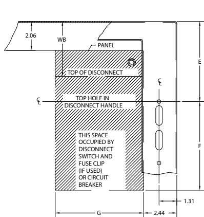
“WAX-SSN4” Style Enclosures
