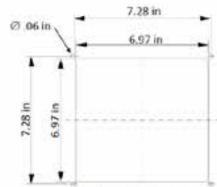
Mounting Cutout
