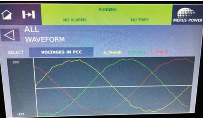
Figure 7: HMI showing voltages at 2AHF-2A panel
