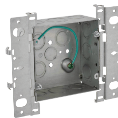
Ultimate Mounting Bracket with 4-11/16" Box 257GHF
