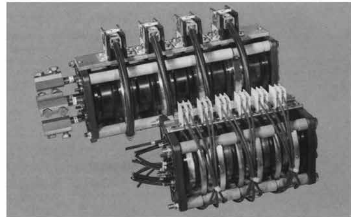
BRUSH AND FINGER ASSEMBLY
