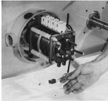
BRUSH AND FINGER ASSEMBLY
