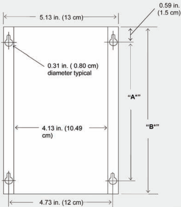
Figure 4. Fiber service unit top view
