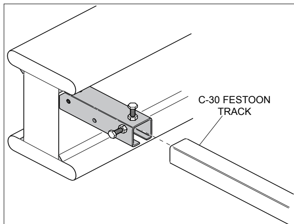
AFFIXING TRACK TO CRANE BOX
