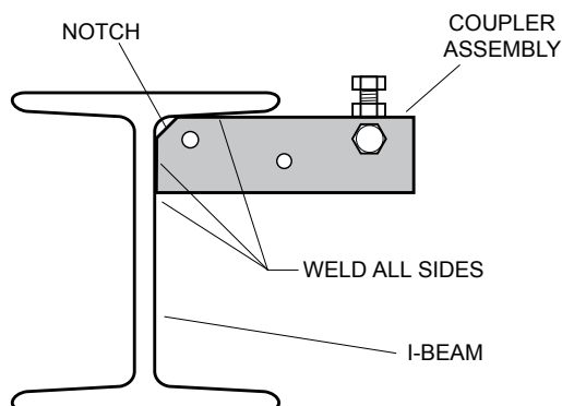
AFFIXING TRACK TO I-BEAM
