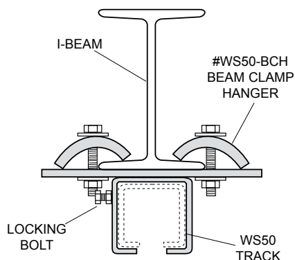
Figure 1 TOOL RAIL BENEATH I-BEAM, PARALLEL TO BEAM
