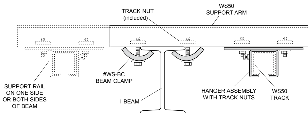
Figure 1 TOOL RAIL BENEATH I-BEAM, PARALLEL TO BEAM
