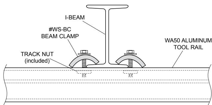
Figure 2 ALUMINUM TOOL RAIL BENEATH I-BEAM, PERPENDICULAR (BEAM-TO-BEAM)
