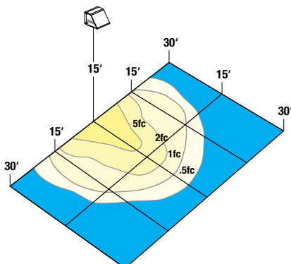
WGM PHOTOMETRIC PERFORMANCE
