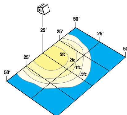
WGL PHOTOMETRIC PERFORMANCE
