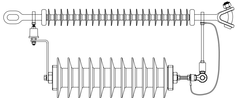
607 Series Protecta*Lite mounted on a Quadri*Sil Suspension Insulator
