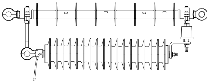
602 Series Protecta*Lite mounted on a PDI Insulator
