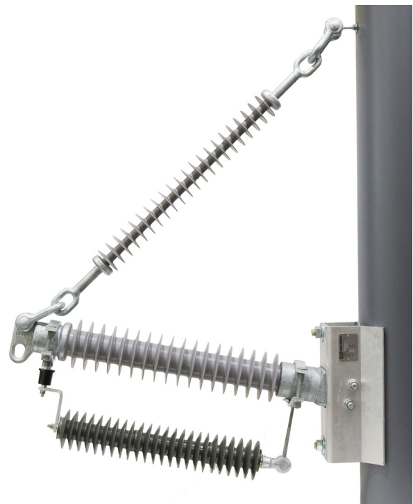
Insulator Mount
