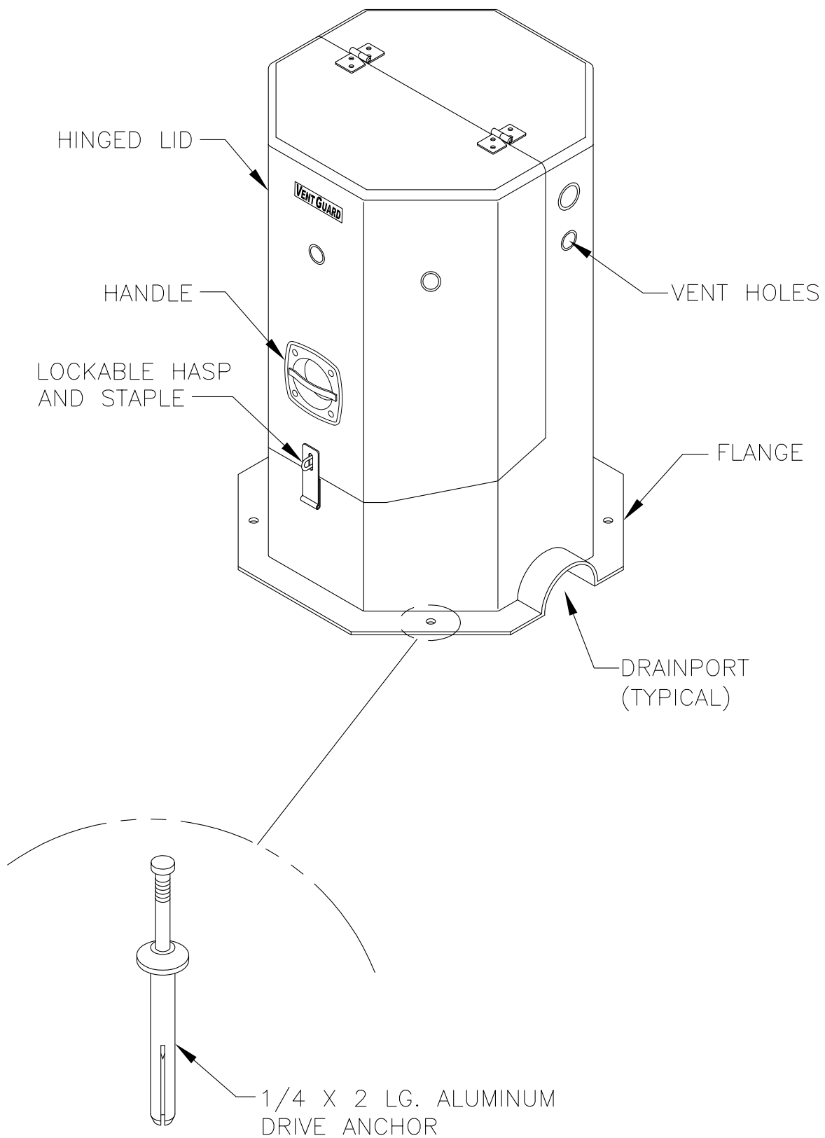
LOCKING DETAIL 4 PLACES
