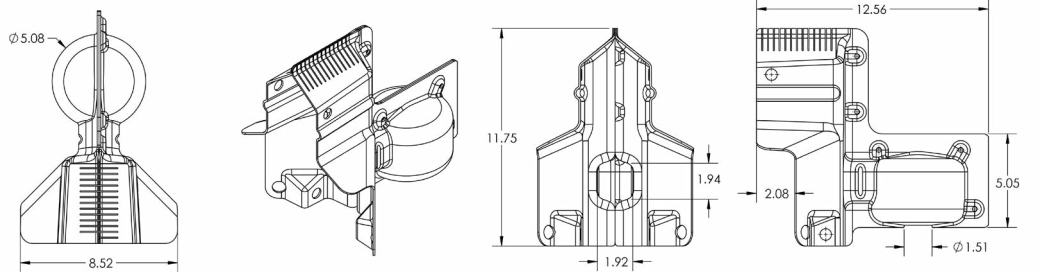
Technical Drawing for Solid Blade Disconnect Guard 900 amp
