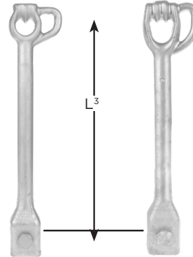
Twineye® & Tripleye® Guy Adapters WITH Pulling Eye
