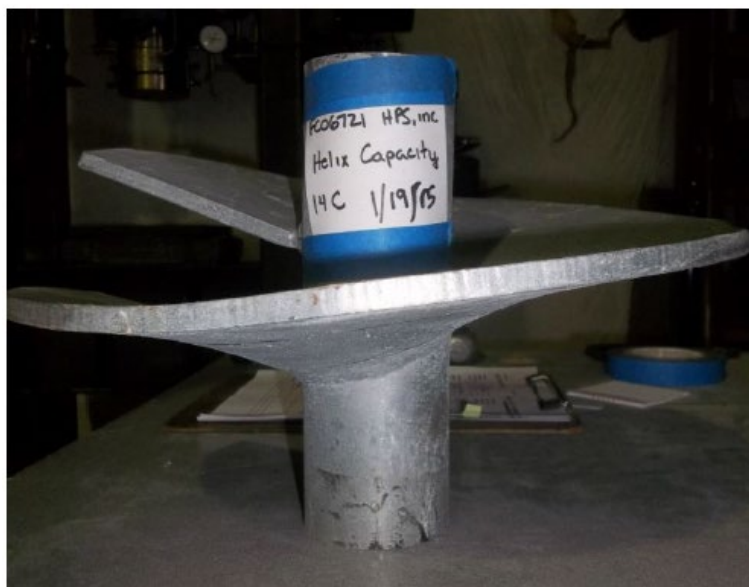
FIG. C-2 – RS2875 14" DIA. HELIX - TEST RESULTS
