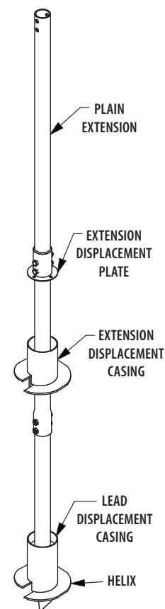
GROUTFORCE PILE ASSEMBLY, FIGURE 7-54
