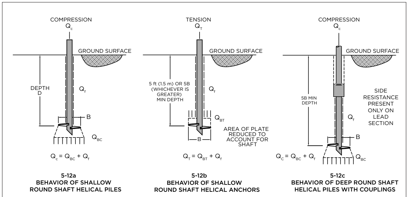
INDIVIDUAL BEARING AND SIDE RESISTANCE MODELS FOR HELICAL PILES AND ANCHORS WITH ROUND (PIPE) SHAFTS FIGURE 5-12
