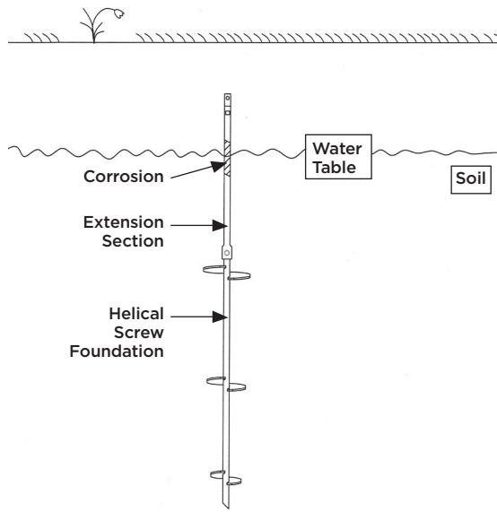
CORROSION OF HELICAL PILE/ANCHOR AT THE WATERLINE FIGURE A-8
