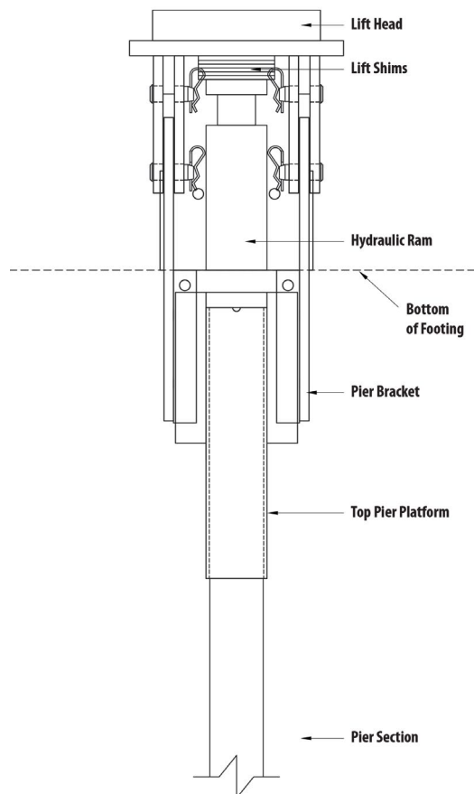
RESTORATION USING LIFT HEAD AND HYDRAULIC RAM FIGURE 6-2
