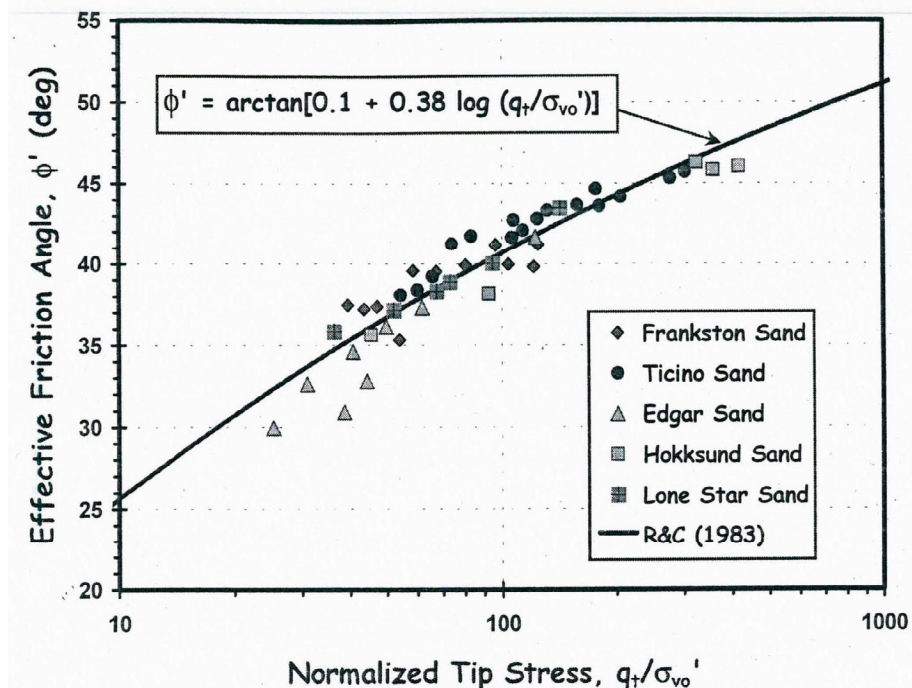
RELATIONSHIP BETWEEN FRICTION ANGLE AND CPTU EFFECTIVE TIP RESISTANCE FIGURE 5-17
