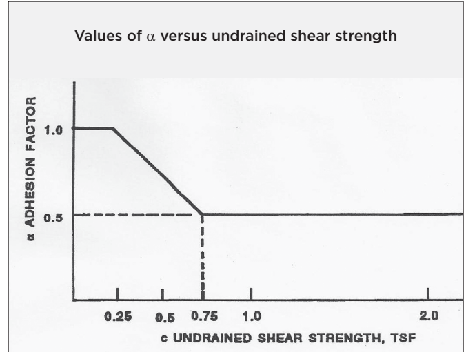
VARIATION IN ADHESION FACTOR FROM AMERICAN PETROLEUM INSTITUTE [ASCE (1993B)] FIGURE 5-11
