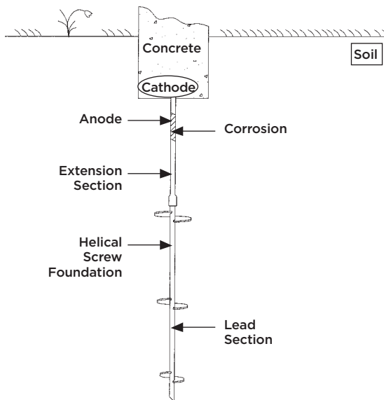
CORROSION OF HELICAL PILE/ANCHOR FOUNDATION WITH A CONCRETE CAP FIGURE A-9
