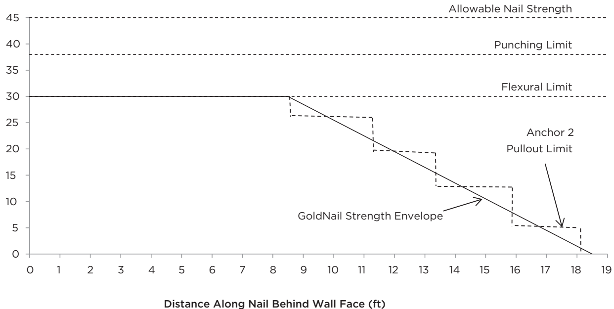
GOLDNAIL STRENGTH ENVELOPE FIGURE 8-17
