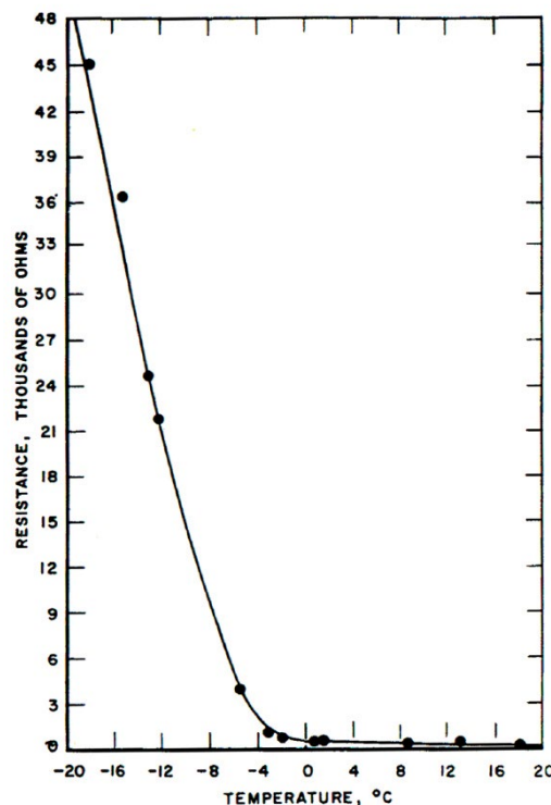
EFFECT OF TEMPERATURE ON EARTH RESISTANCE (ROMANOFF, 1957) FIGURE A-2
