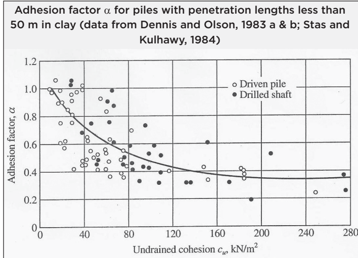
VARIATION IN ADHESION FACTOR WITH UNDRAINED SHEAR STRENGTH OF CLAYS [MURTHY (2003)] FIGURE 5-10
