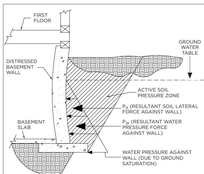
DISTRESSED BASEMENT WALL WITH ACTIVE SOIL PRESSURE AND WATER PRESSURE ACTING AGAINST THE WALL
