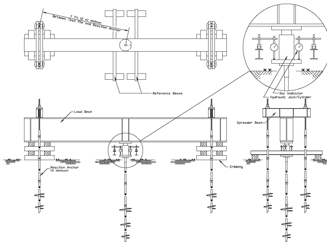
BASIC COMPRESSION FIELD TEST SET-UP FIGURE B-3
