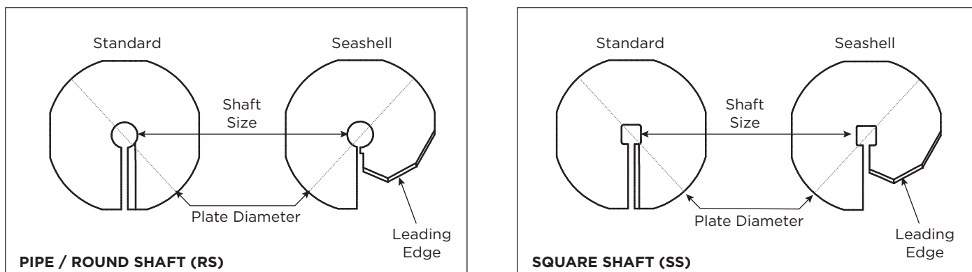
PROJECTED VIEWS OF ROUND SHAFT AND SQUARE SHAFT HELIX PLATES FIGURE 7-2
