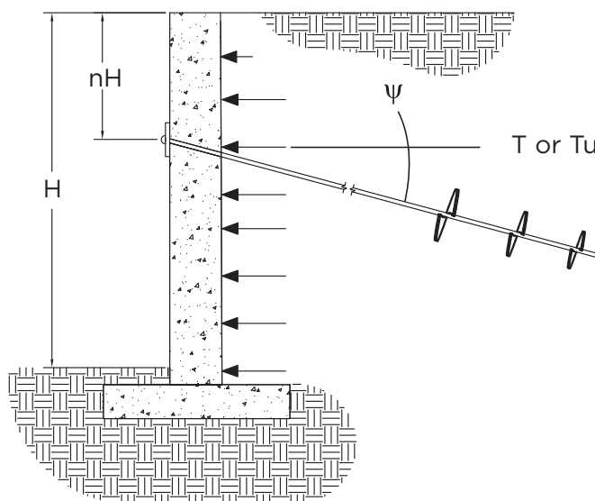
ESTIMATED TIEBACK FORCE REQUIRED FOR RETAINING WALLS 15 FEET HIGH OR LESS FIGURE 4-5
