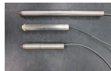
CPT/CPTU FIGURE 2-10
