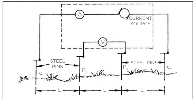
Wenner 4-Pin Method for Measuring Soil Resistivity Figure A-4
