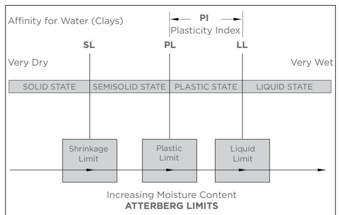
Plasticity and Atterberg Limits Figure 2-4
