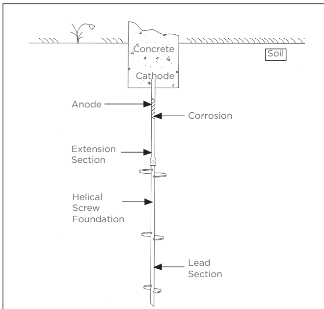
Corrosion of Helical Pile/Anchor Foundation With a Concrete Cap Figure A-9
