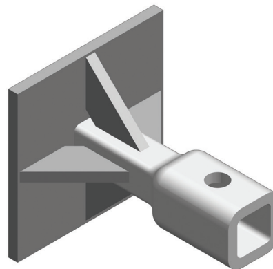
New Construction Cap for Type SS Shafts, Equal Compression and Uplift Capacity Figure 6-51
