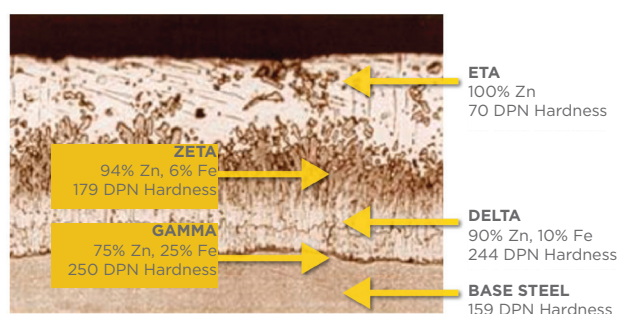
HDG Cross-Section from: American Galvanizer's Association
