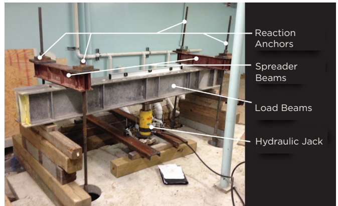
Compression Test Figure B-2
