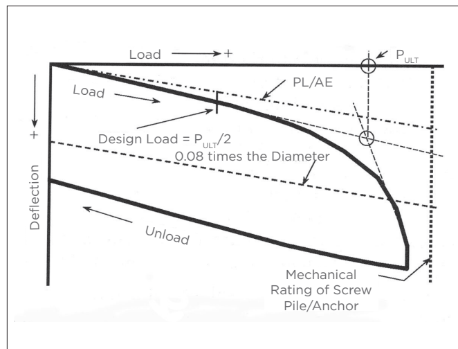
Sample Compression Test Load-Deflection Curve Figure B-5
