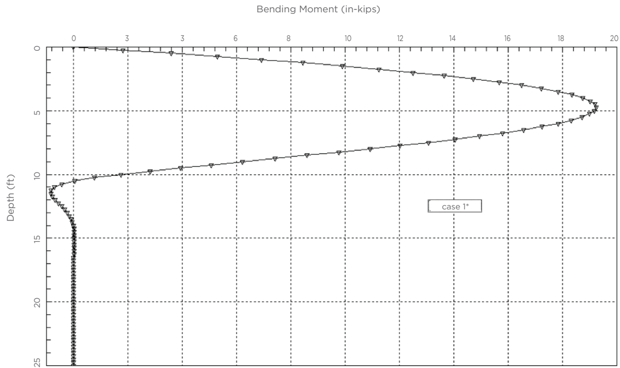
Lateral Deflection vs Depth Figure 7-21
