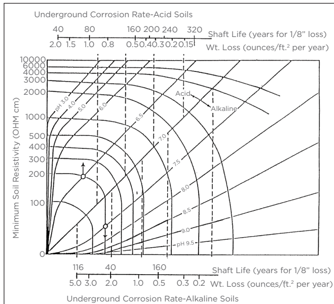
Nomograph for Estimating the Corrosion Rate of Pile/Anchor Shafts Figure A-6
