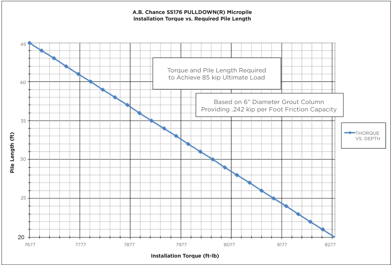
Torque vs. Required Length Figure 7 -13
