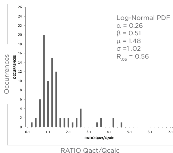
Torque correlation model Figure 5-7
