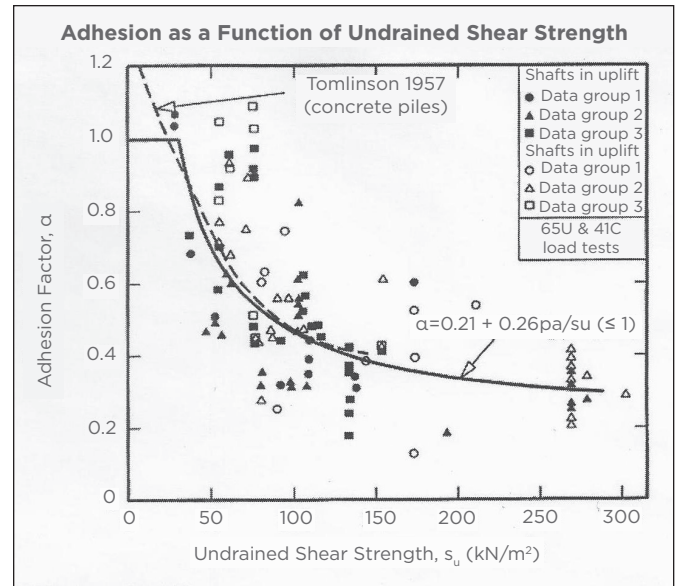
Variation in Adhesion Factor with Undrained Shear Strength of Clays [Canadian Foundation Manual (2006)] Figure 4-7
