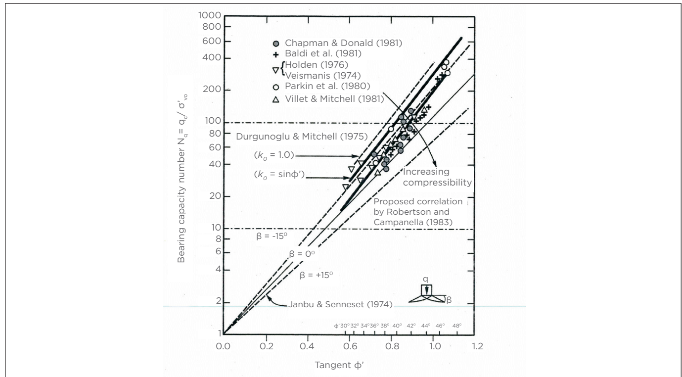
Relationship between Bearing Capacity Number and Friction Angle from Normalized CPT Tip Resistance [Robertson and Campanella (1983)] Figure 4-13
