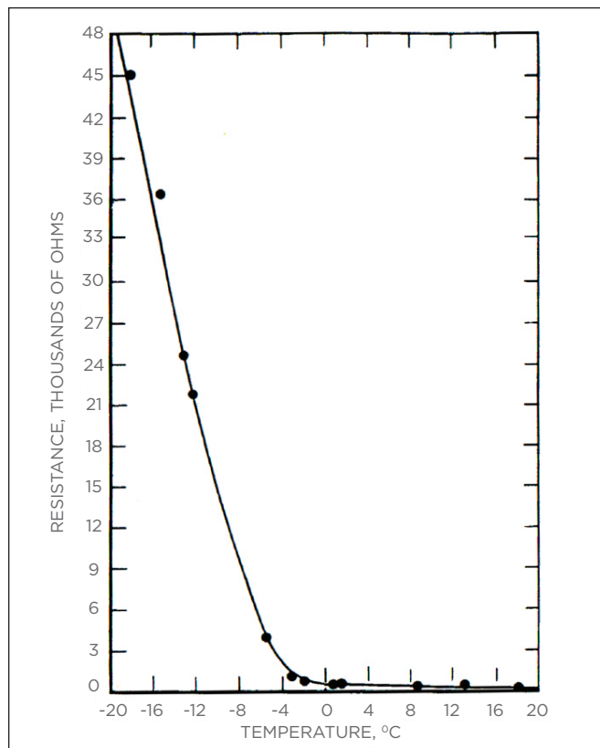
Effect of Temperature on Earth Resistance (Romanoff, 1957) Figure A-2
