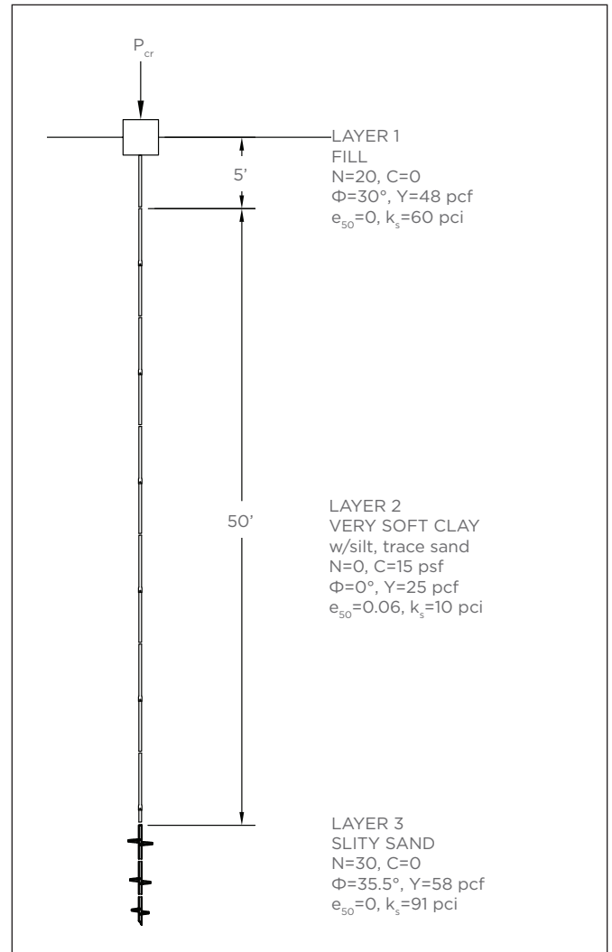
Foundation Details Figure 7-36
