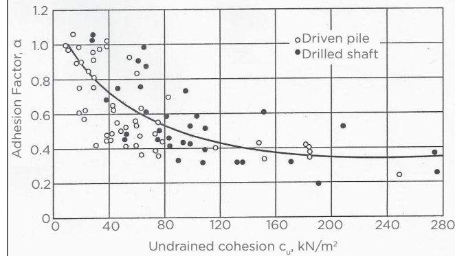
Variation in Adhesion Factor with Undrained Shear Strength of Clays [Murthy (2003)] Figure 4-8
