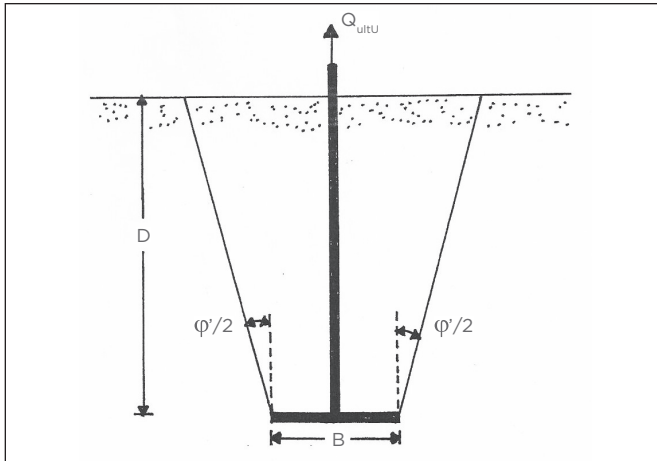
Proposed Failure Mechanism for Shallow Single-Helix Anchors in Dense Sand Figure 4-3
