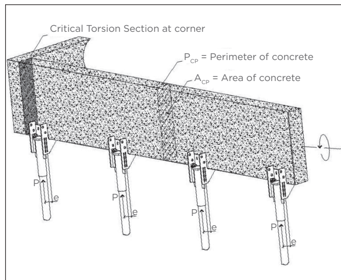
Pier Bracing near Grade Beam Corner Figure 4-23
