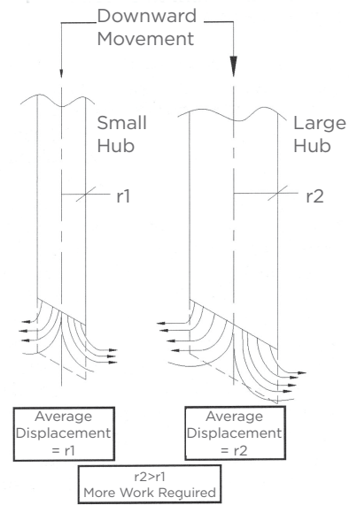
Shaft/Pilot Point with Flow Lines Figure 5-5
