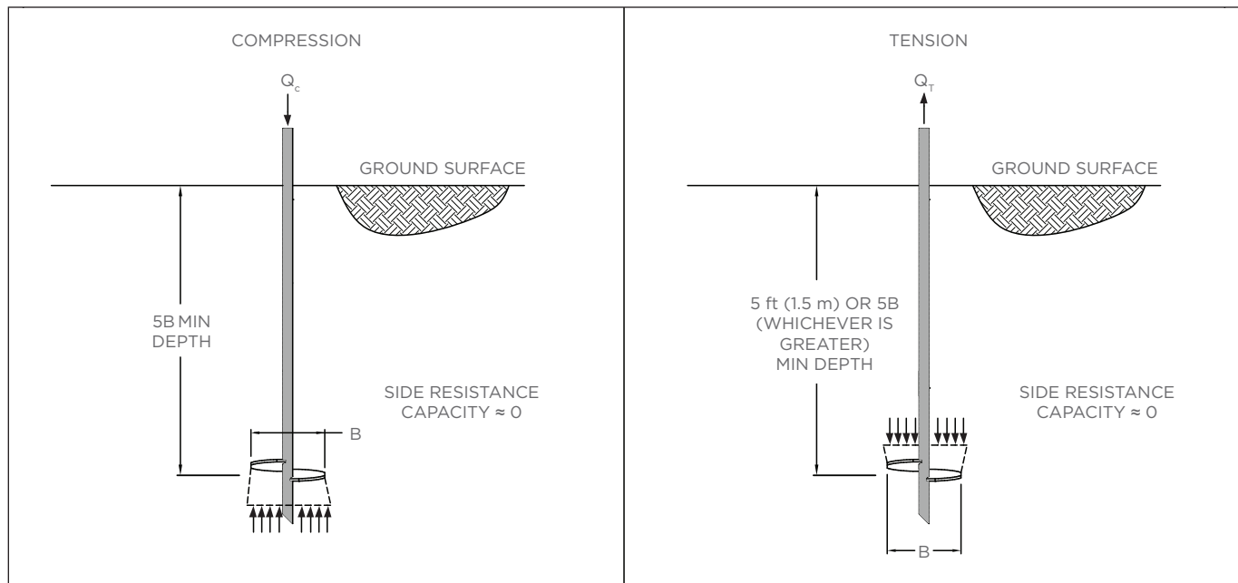
Single-Helix Plate Bearing Capacity Model—Helical Piles with Slender Shafts Figure 4-4
