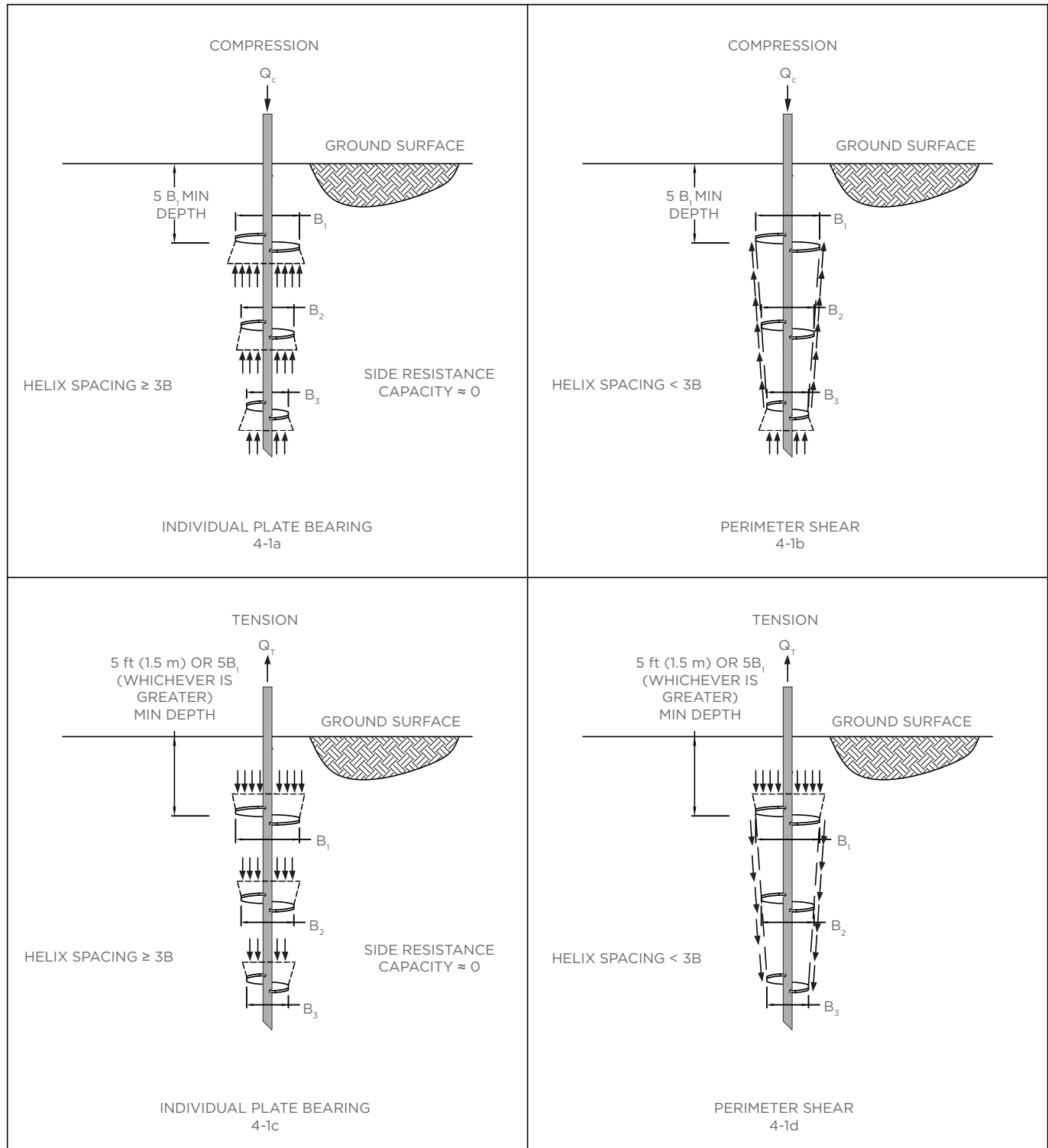
Comparison Between Individual Plate Bearing and Perimeter Shear for Compression and Tension Loading Figure 4-1
