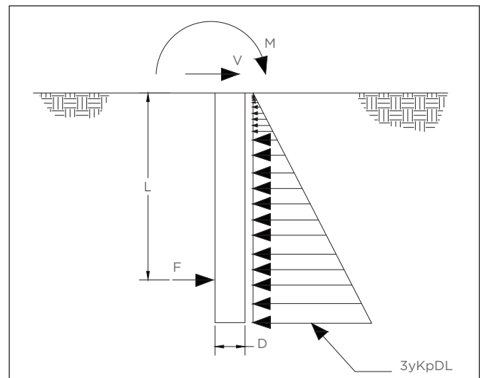
Foundation in Cohesionless Soil Figure 7-32
