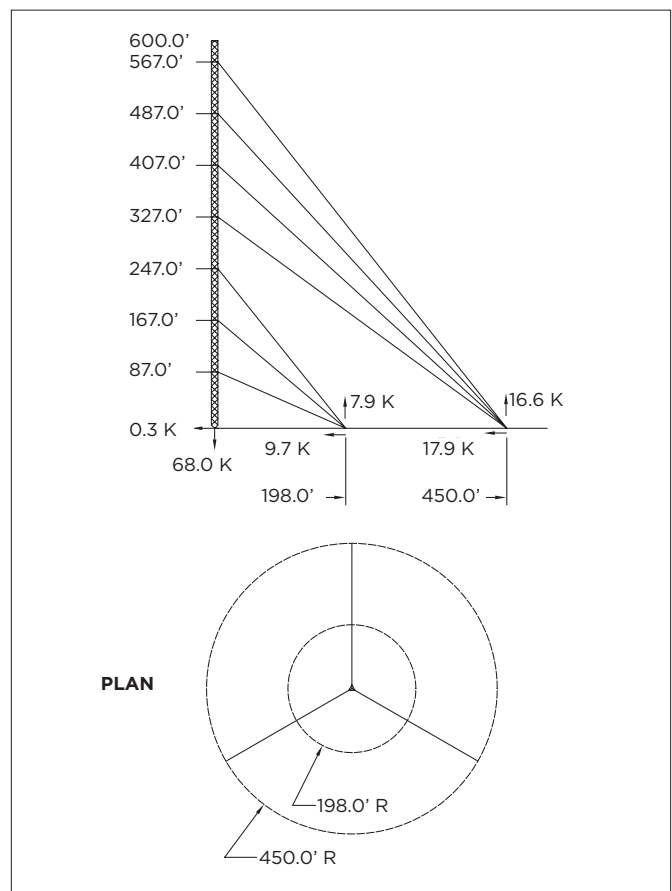
Tower Guy Anchor And Foundation Figure 7-1
