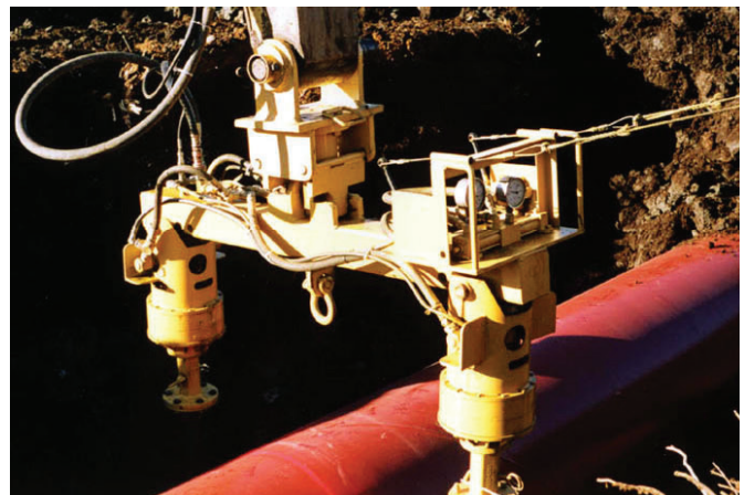
Differential Pressure Torque Indicator Figure 5-12
