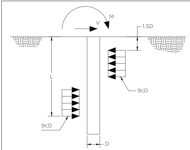
Foundation in Cohesive Soil Figure 7-31
