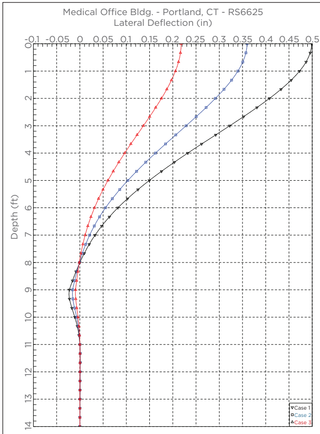
LPILE Plus Sample Plot: Deflection vs. Depth Figure 4-17
