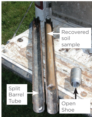
Geometry of Standard Penetration Test Split-Barrel Sampler (ASTM D 1586) Figure 2-9
