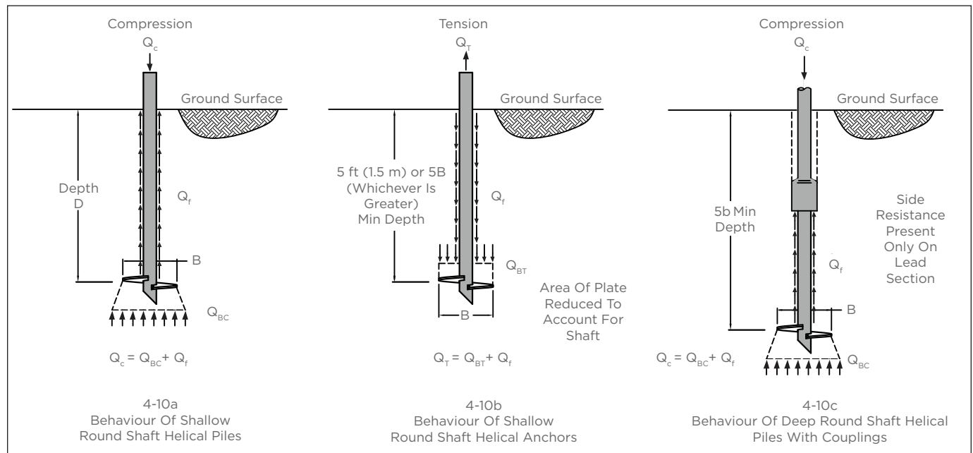
Individual Bearing and Side Resistance Models for Helical Piles and Anchors with Round (Pipe) Shafts Figure 4-10
