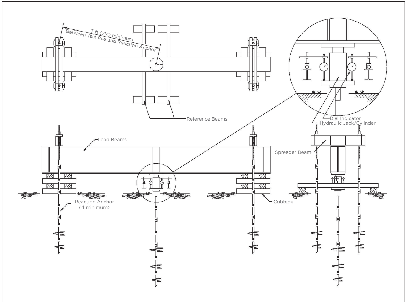
Basic Compression Field Test Set-up Figure B-1
