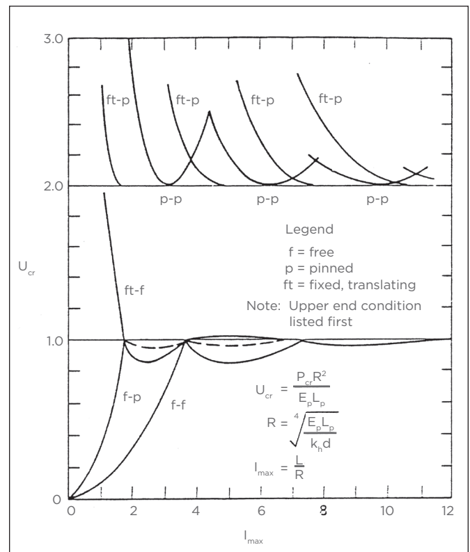
Buckling Load Ratio ( U_{cr} ) vs. Length Ratio ( l_{max} ) [Poulos and Davis (1980)] Figure 4-25
