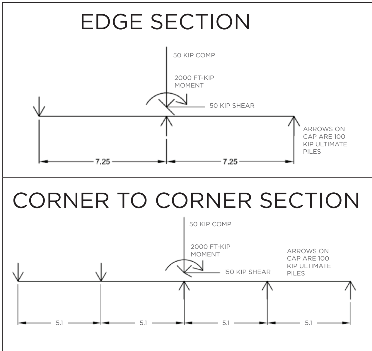
Load Scenarios Figure 7-17
