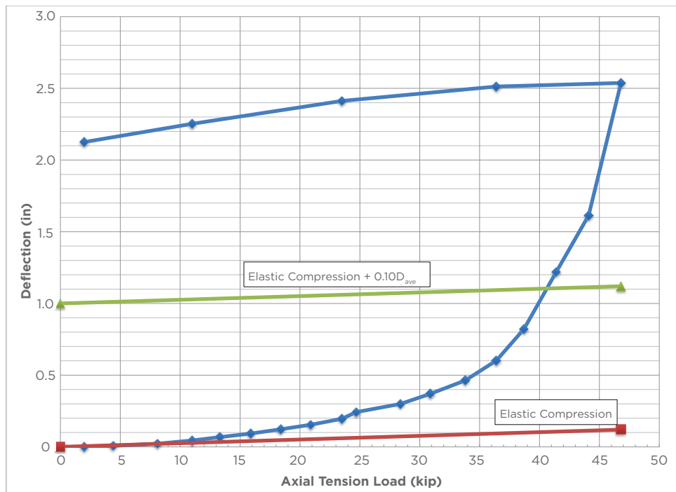
ASTM D3689 "Quick Test" Tension Plot, Figure B-8
