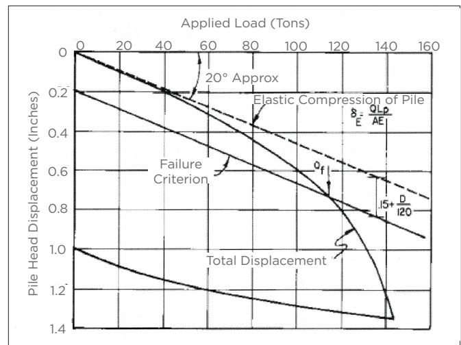
Davisson Method for Determining Net Displacement Figure B-6
