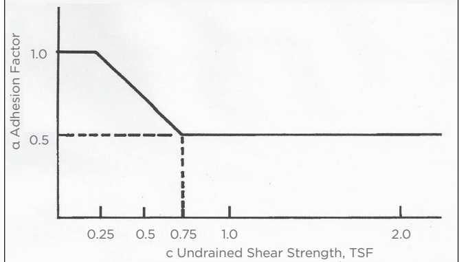
Variation in Adhesion Factor from American Petroleum Institute [ASCE (1993b)] Figure 4-9
