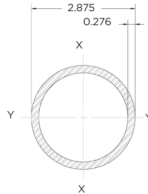
CHANCE Type RS2875.276 HCP Helical Pile Shaft Cross-Section Figure 6-22
