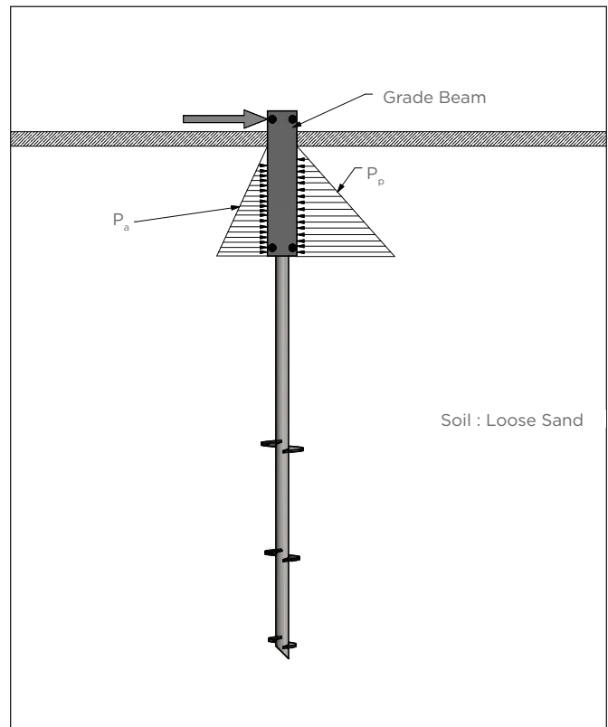
Earth Pressure on a Grade Beam
