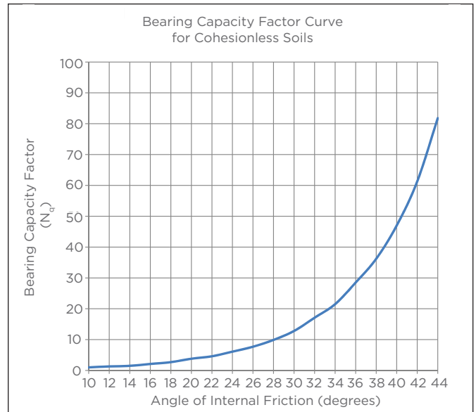
Recommended Bearing Capacity Factor ( N_q ) for Deep Helical Piles/Anchors in Sand Figure 4-6
