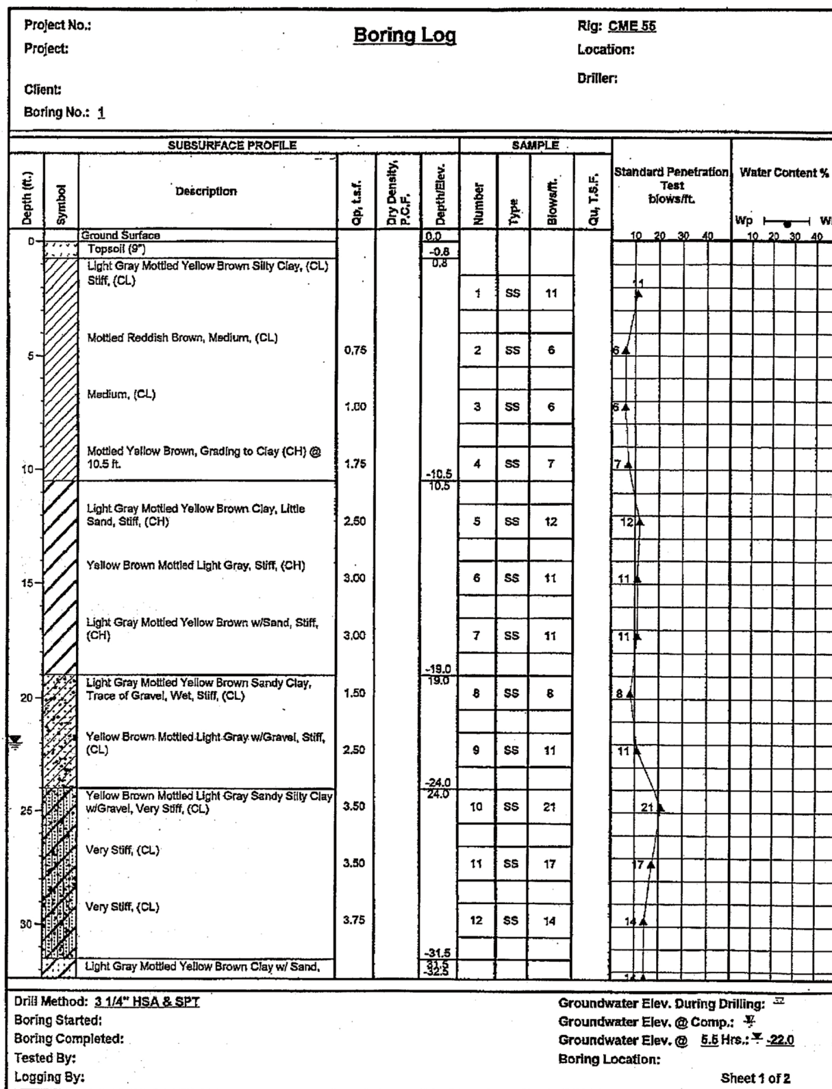
Sample Boring Log Figure 7-2
