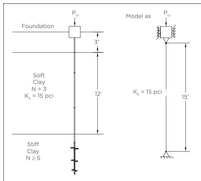
Foundation Details Figure 7-35
