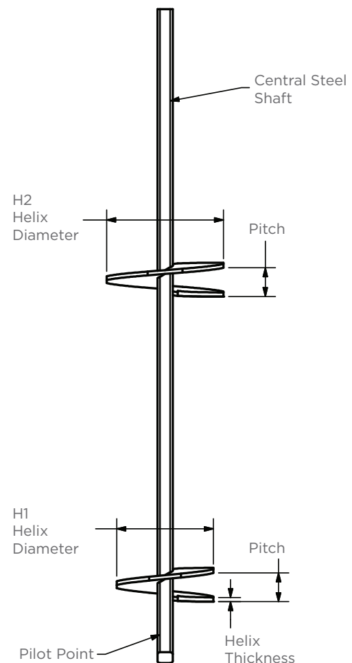
Helical Pile/Anchor Figure 5-1
