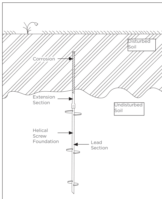
Corrosion of Helical Pile/Anchor in Disturbed Soil Figure A-7
