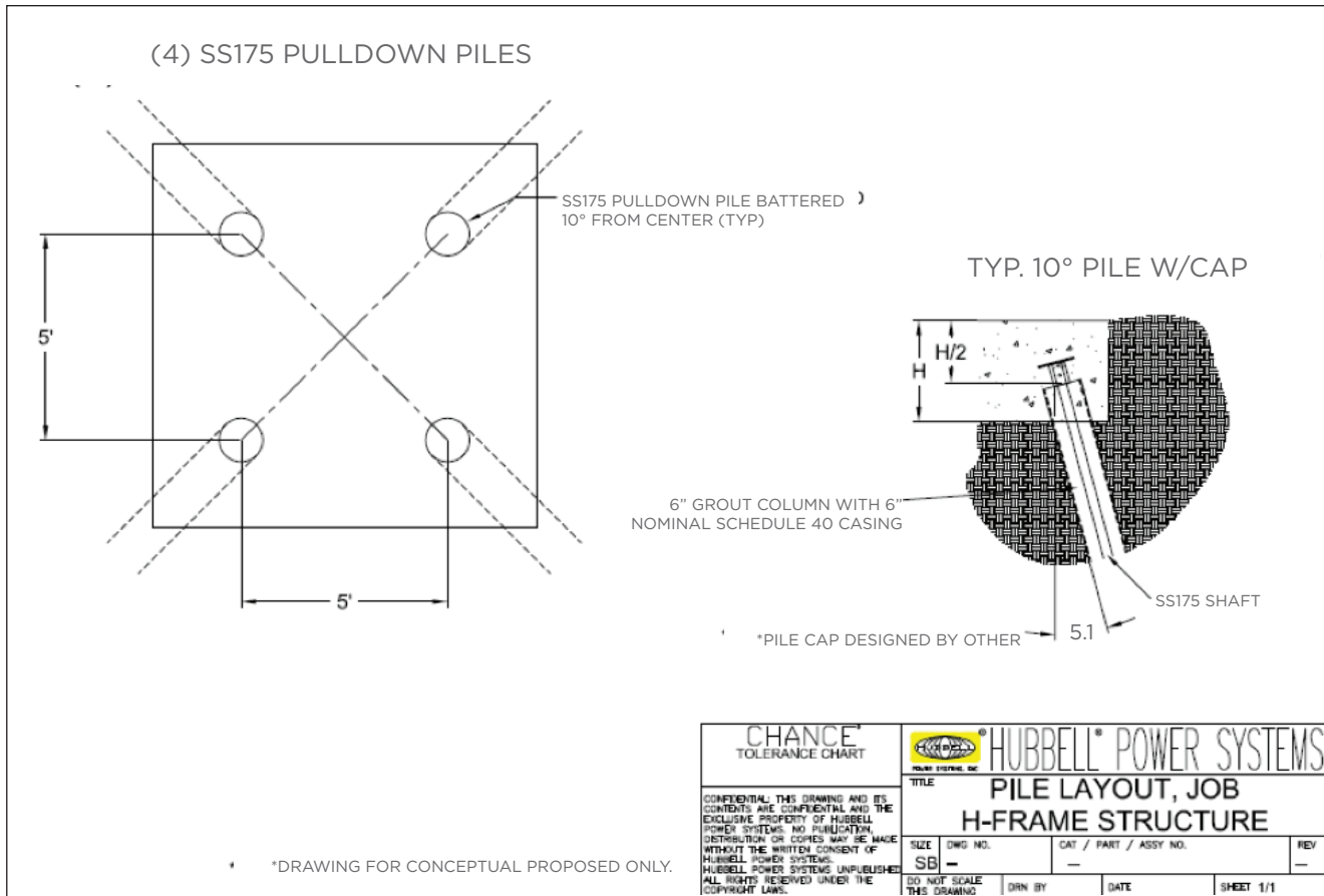
Figure 7 -14: Pile Layout
