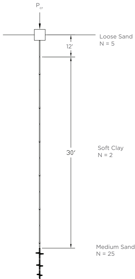
Foundation Details Figure 7-39
