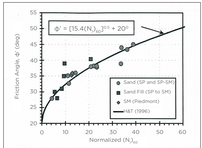
Peak Friction Angle of Sands from SPT RESISTANCE—CORRELATION of Hatanaka & Uchida (1996) [FHWA Reference Manual on Subsurface Investigations (2002)] Figure 4-11
