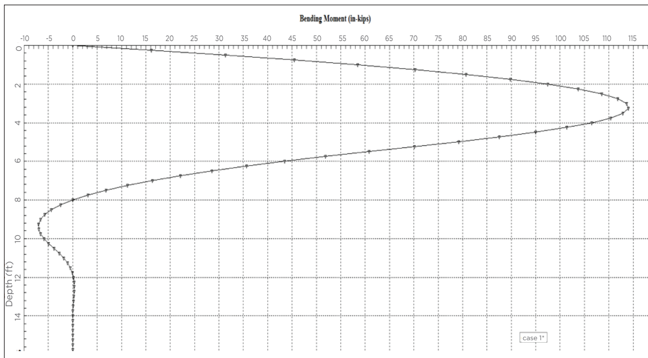
Bending Moment vs Depth Figure 7-19
