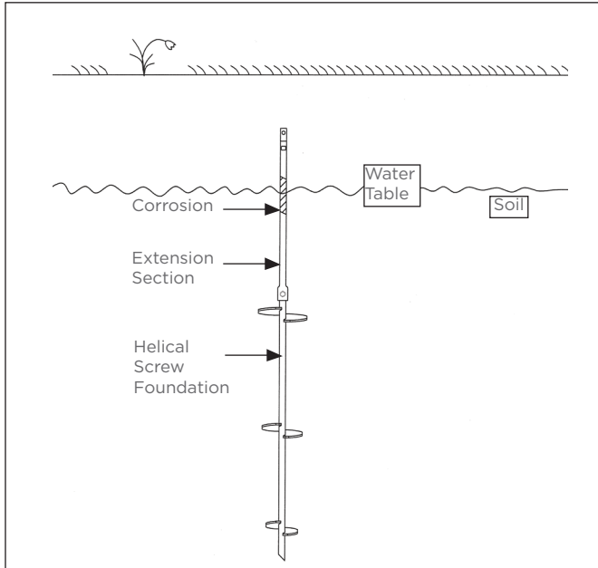
Corrosion of Helical Pile/Anchor at the Waterline Figure A-8
