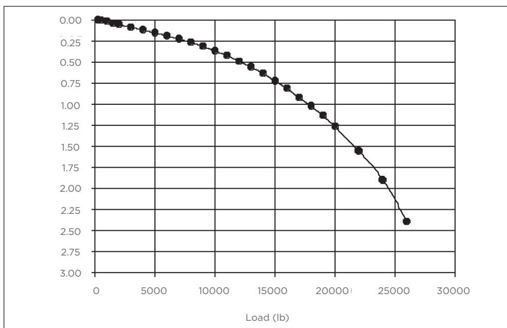
Deflection vs. Load Plot Figure 4-27
