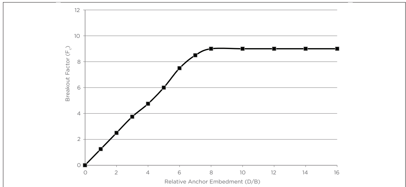
Variation in Uplift Breakout Factor for Shallow SINGLE-HELIX Anchors in Clay Figure 4-2
