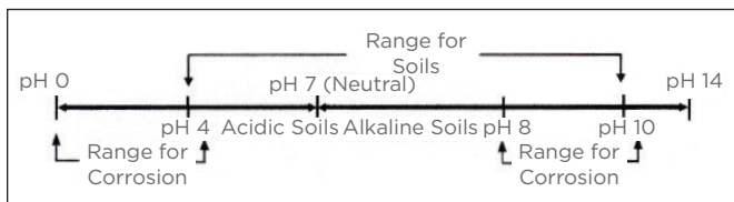
Corrosion of Metal in Soil vs pH Figure A-3
