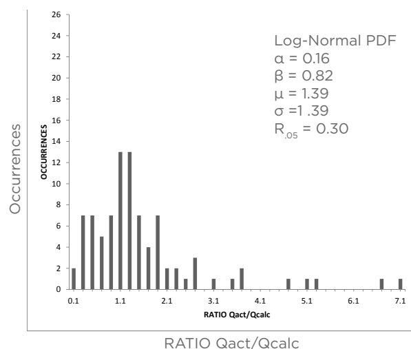
Individual Bearing Method Figure 5-6
