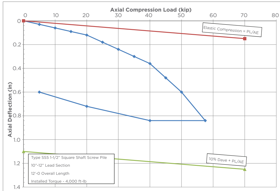
ASTM D1143 "Quick Test" Compression Plot, Figure B-7
