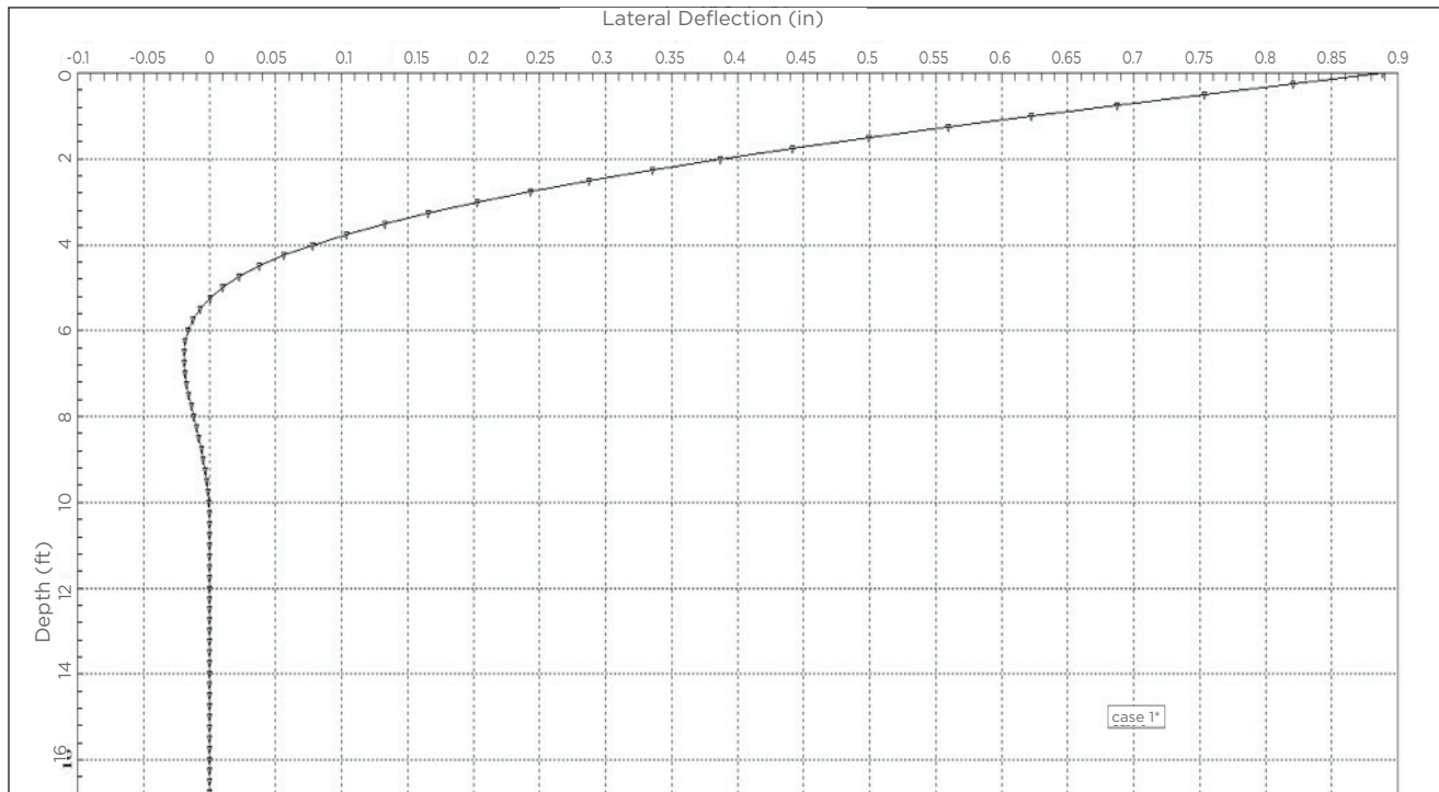
Lateral Deflection vs Depth Figure 7-18
