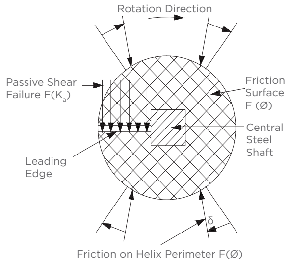
Top View of Helix Figure 5-2
