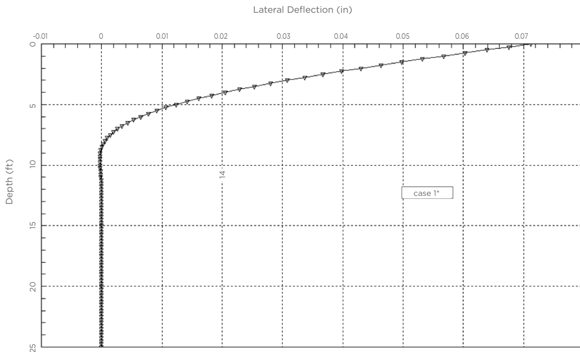
Lateral Deflection vs Depth Figure 7-20
