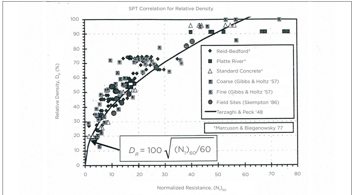
Relative Density of Clean Sands from SPT Resistance Figure 4-12
