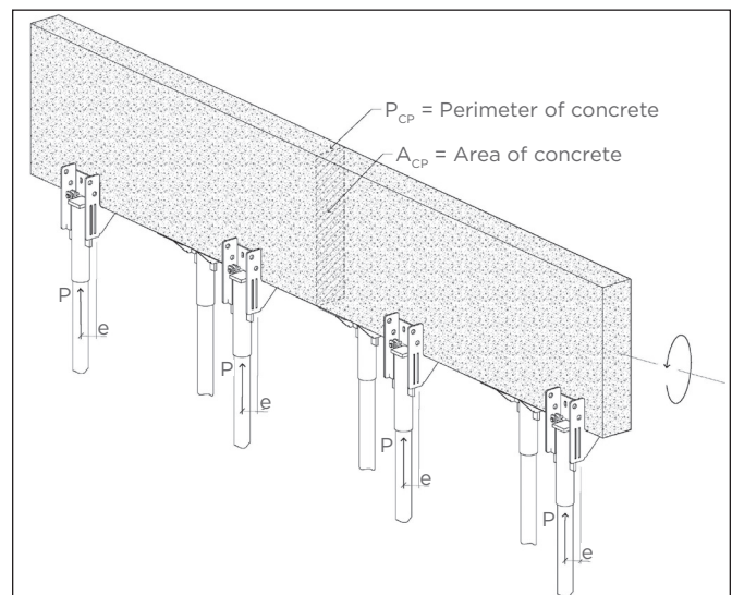
Pier Bracing on Continuous Grade Beam Figure 4-24
