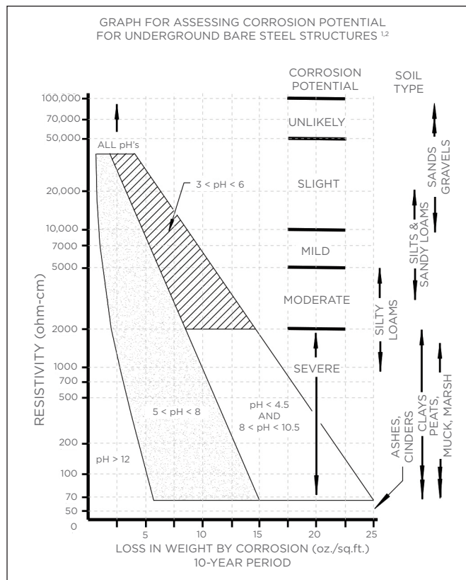
Steel Loss Due to Corrosion, Figure A-5
