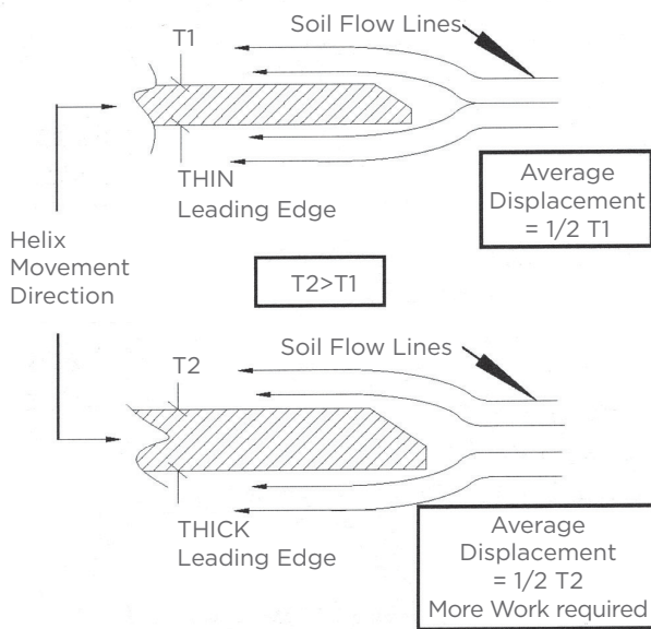
Section View of Leading Edge with Flow Lines Figure 5-4
