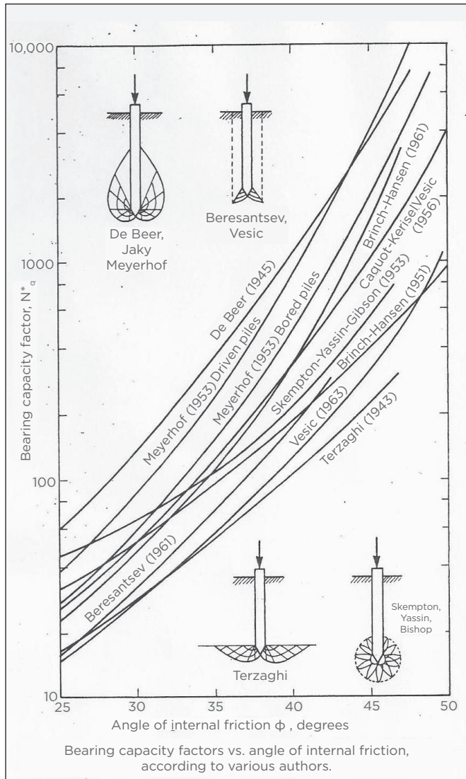
Reported Values of Bearing Capacity Factor ( N_q ) for Deep Foundations in Sands [Winterkorn & Fang (1983)] Figure 4-5
