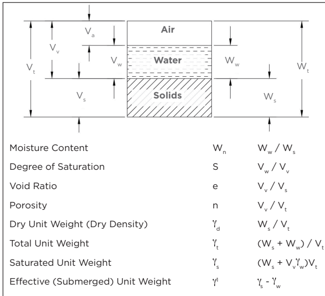
Soil Phases and Index Properties Figure 2-2
