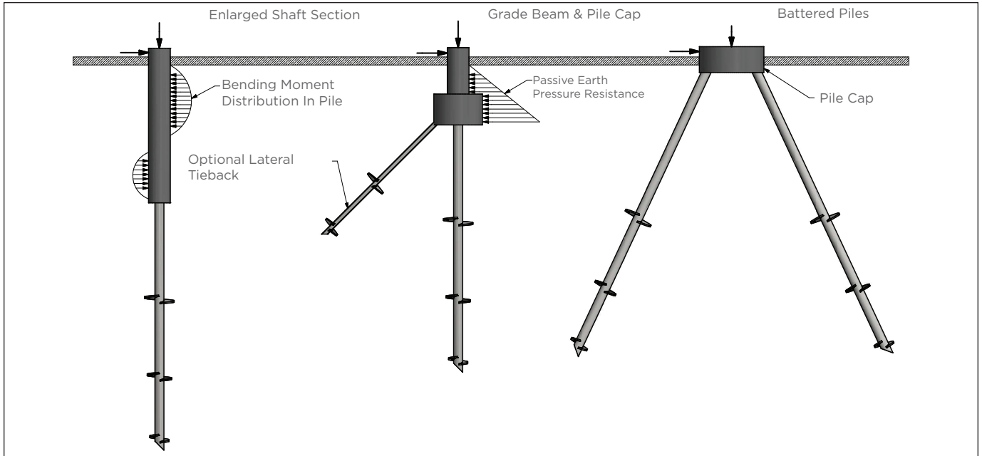
Lateral Resistance Methods Figure 4-16
