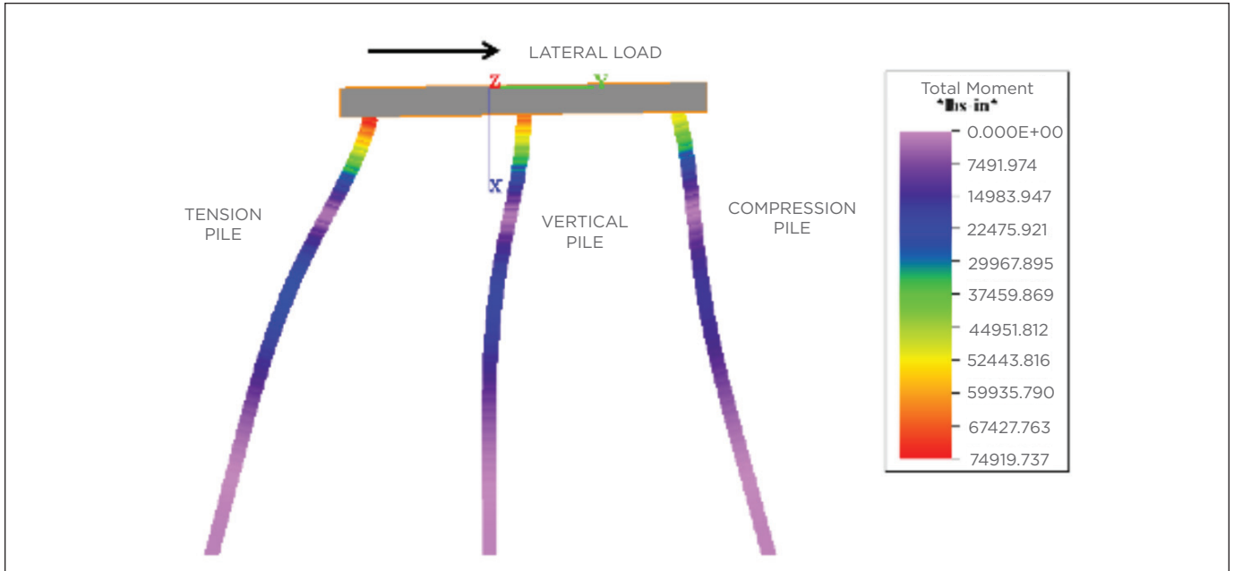
Figure 4-21. Group Box Pile Deflection
