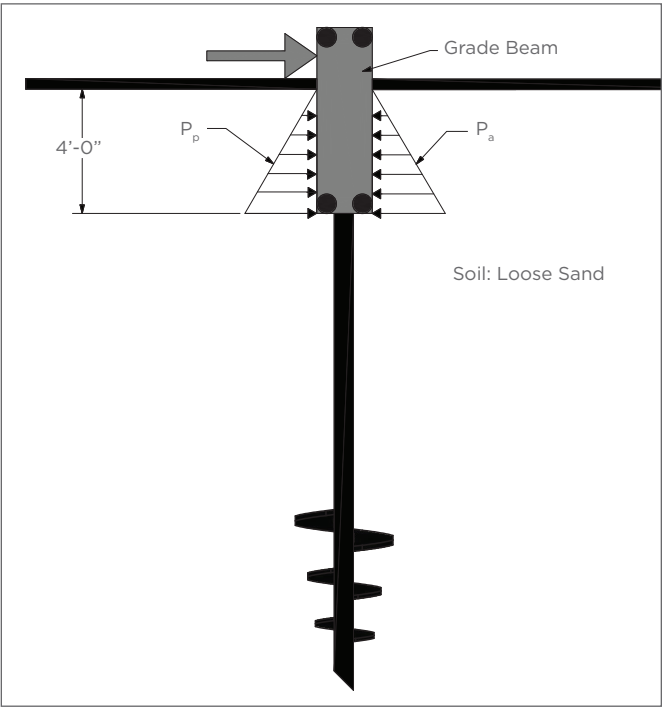
Earth Pressure on a Grade Beam Figure 7-33
