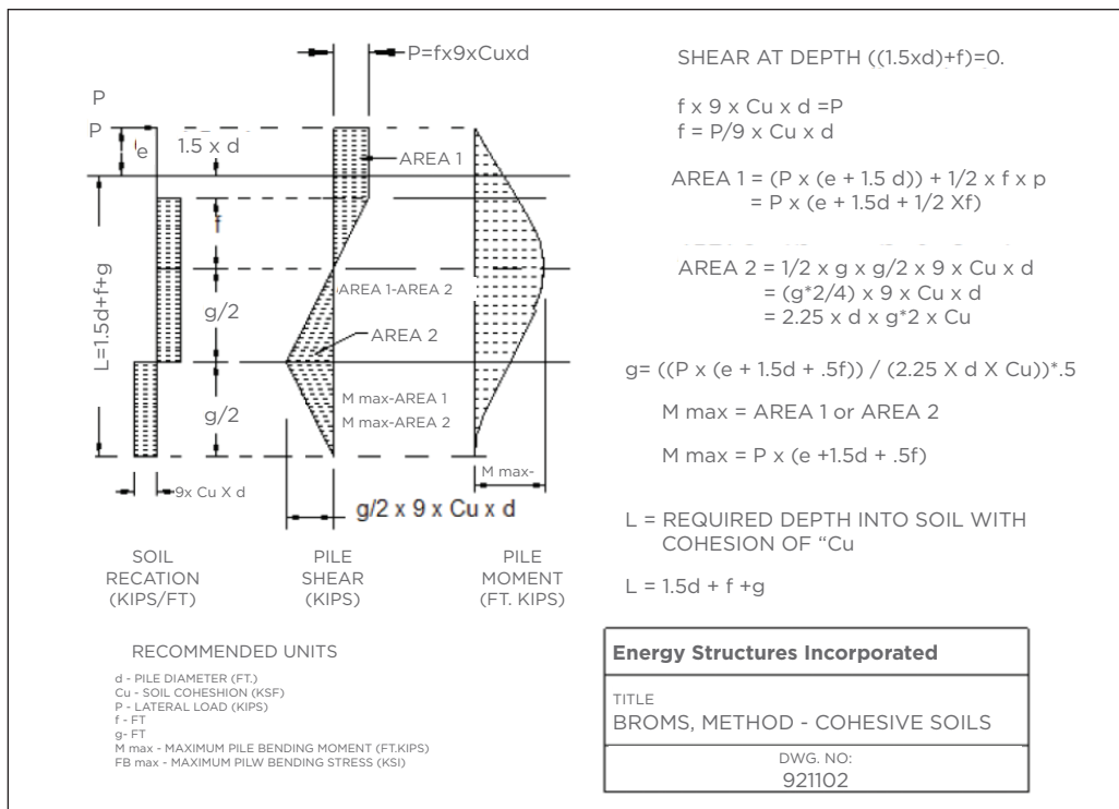
Broms' Method for Laterally Loaded Short Piles Figure 7-27
