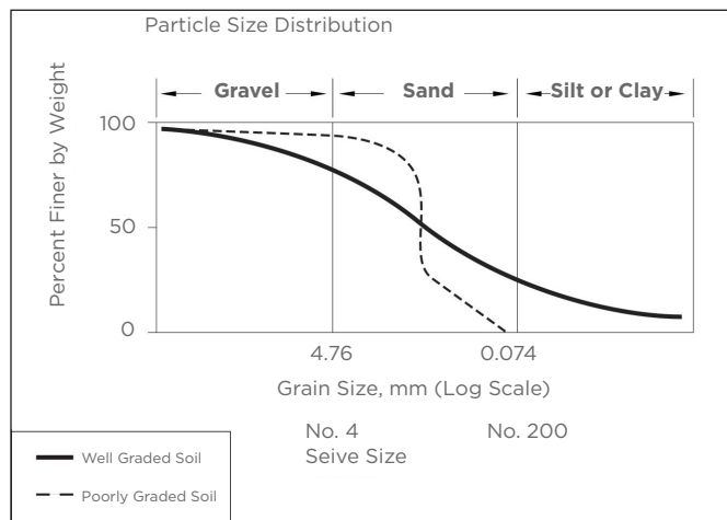
Typical Grain Size Distribution Curves Figure 2-3
