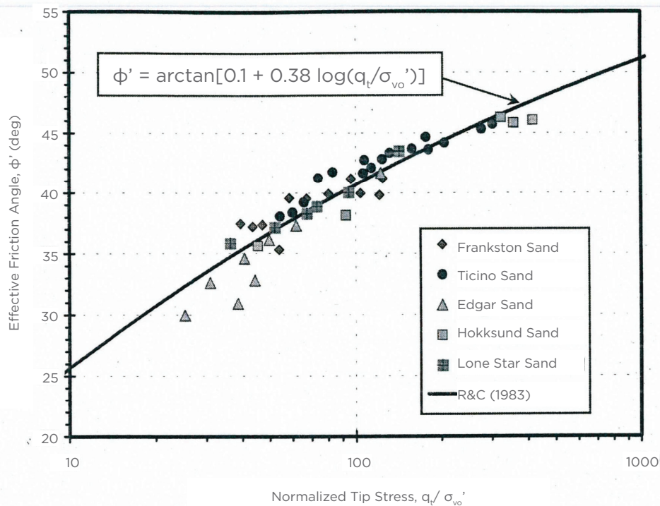
Relationship Between Friction Angle and CPTU Effective Tip Resistance Figure 4-15
