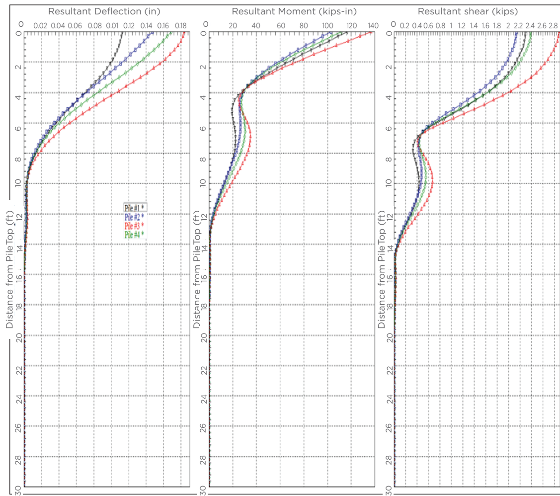
Resultant Deflection, Moment, and Shear Figure 7-10
