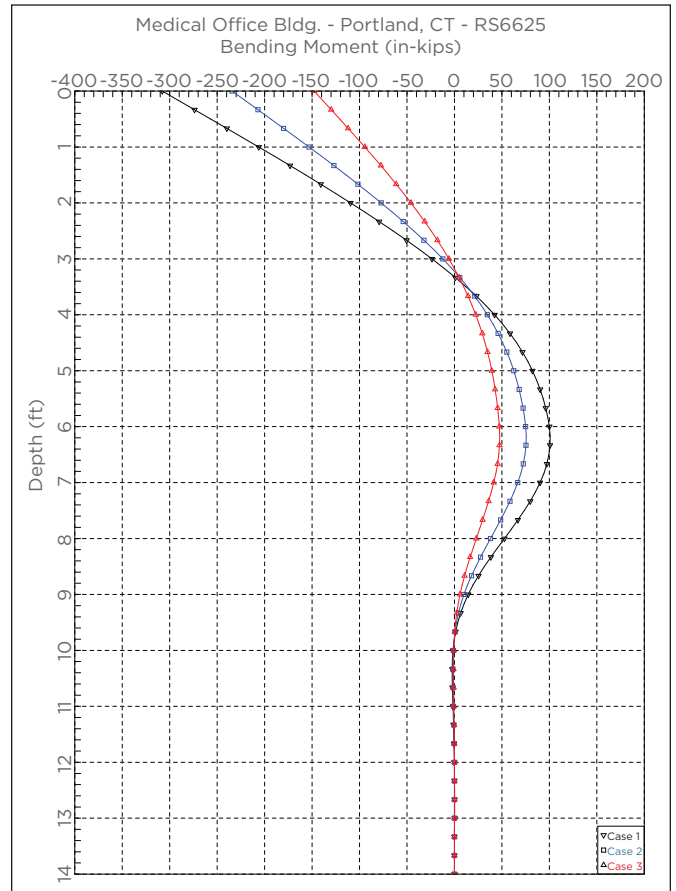
LPILE Plus Sample Plot: Bending Moment vs. Depth Figure 4-18
