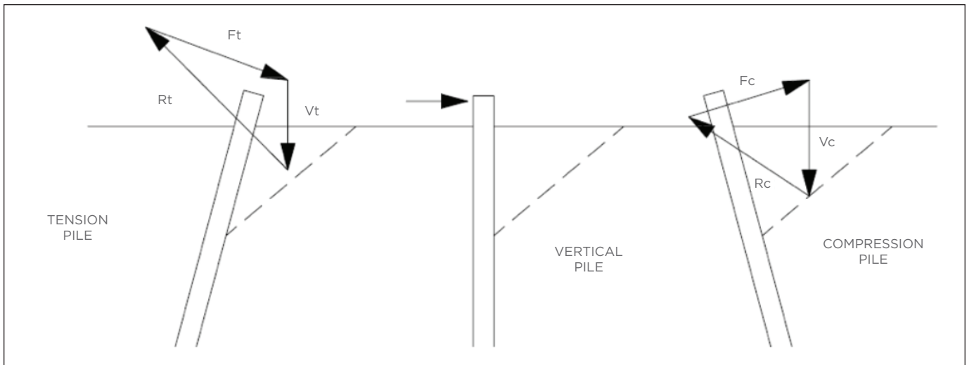
Figure 4-22 Behavior of Battered Piles
