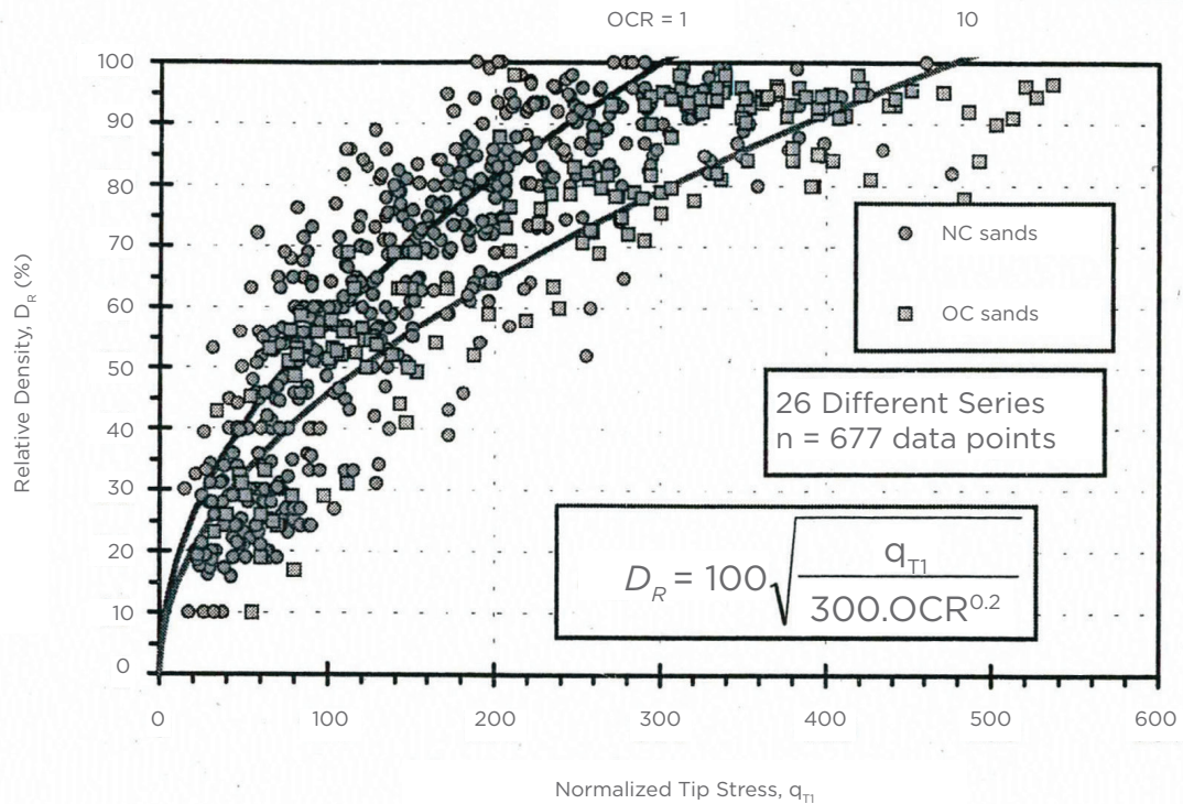
Relationship Between Relative Density and CPT Normalized Tip Stress for Normally Consolidated (NC) and Overconsolidated (OC) Sands Figure 4-14
