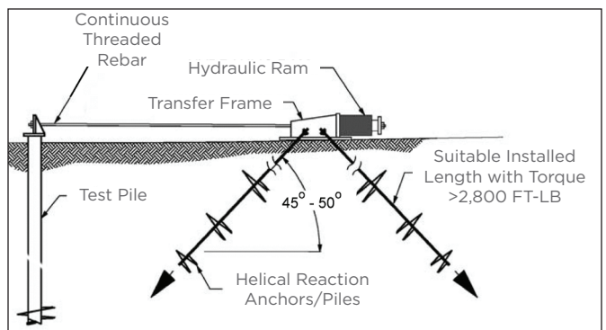
Lateral Load Test Equipment Configuration Figure B-3
