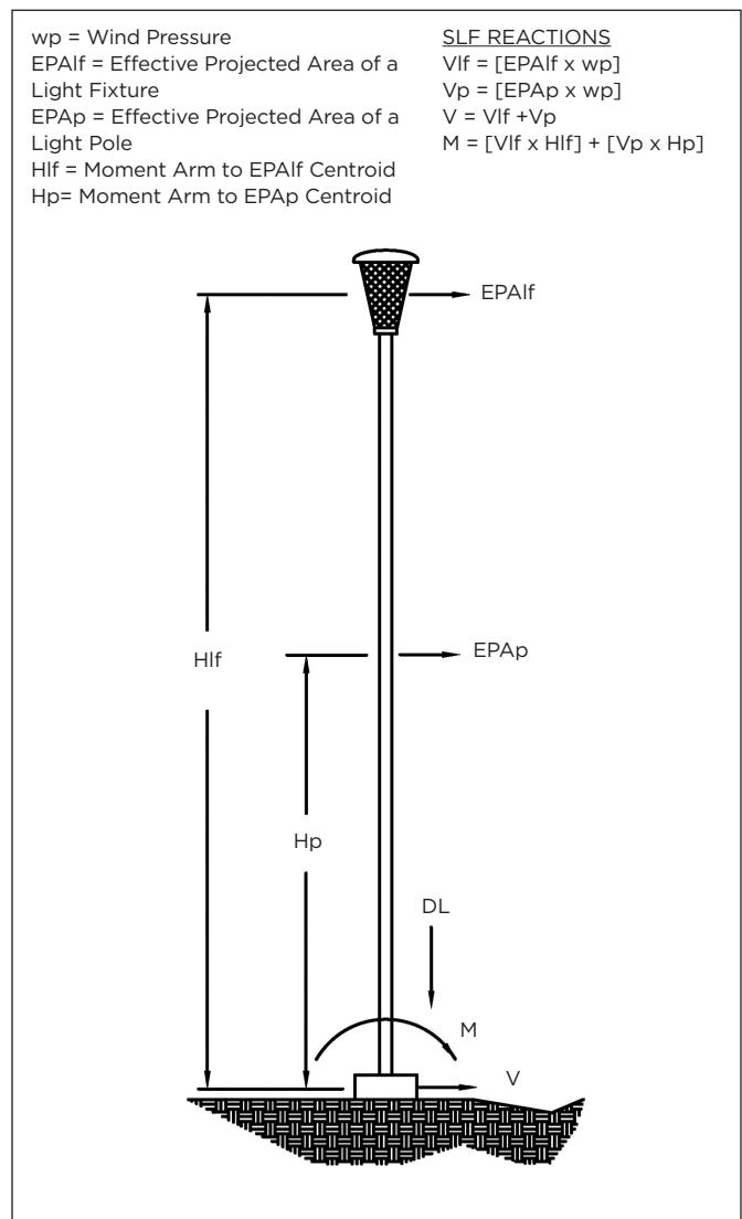
Pole Load Diagram Figure 7-30
