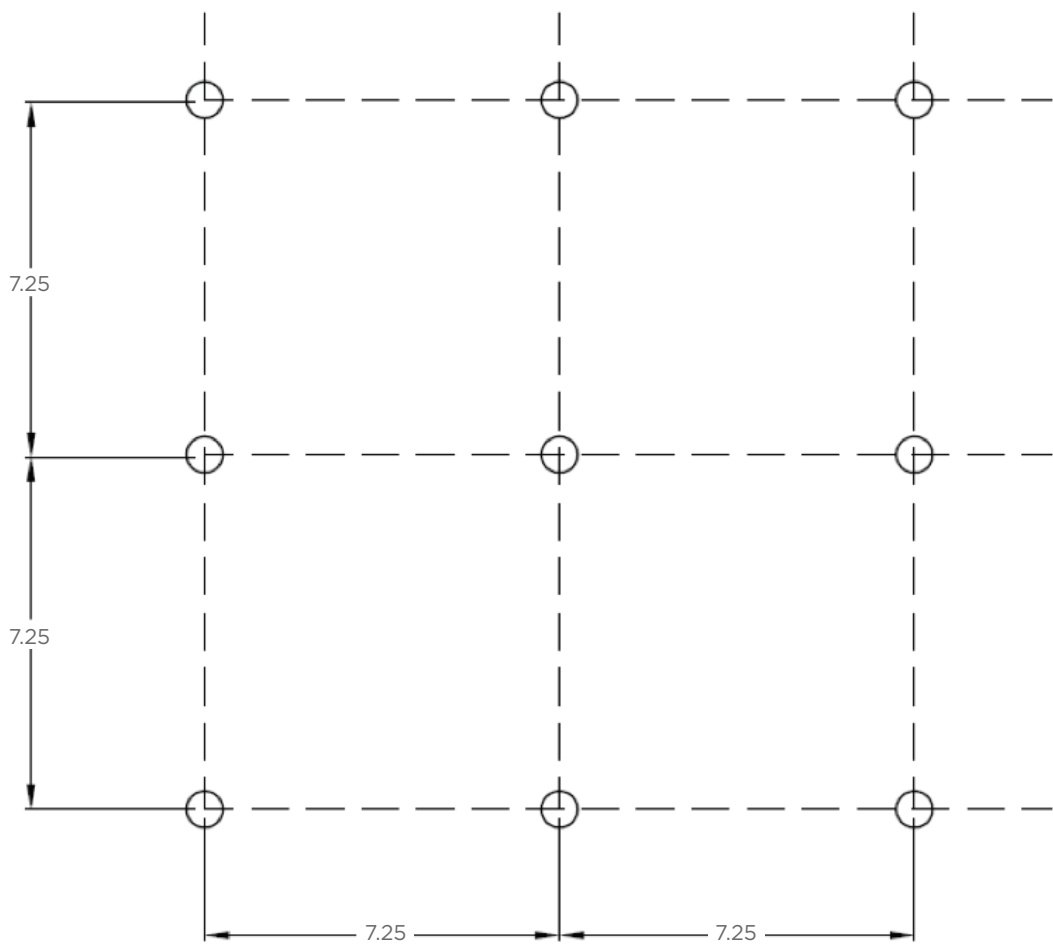
Anticipated Pile Layout Figure 7-16
