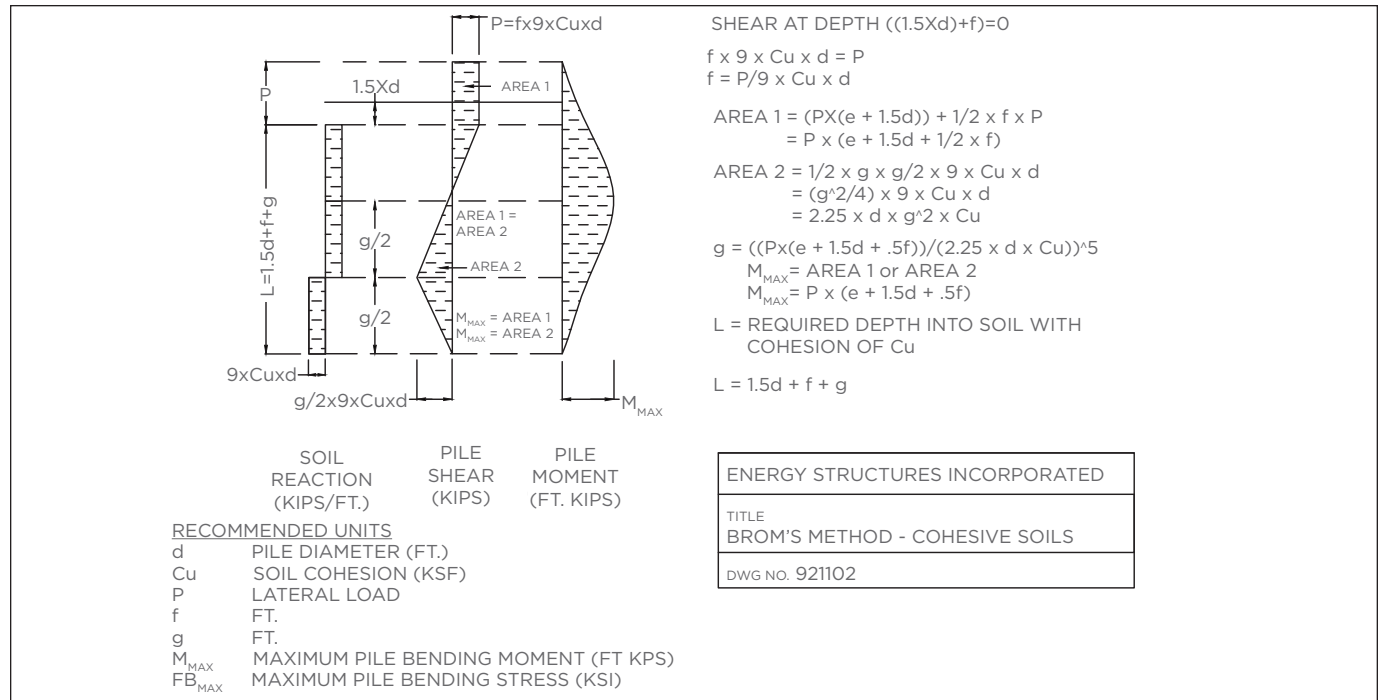
Broms' Method for Short Piles in Clay (Energy Structures, Inc., 1994)
