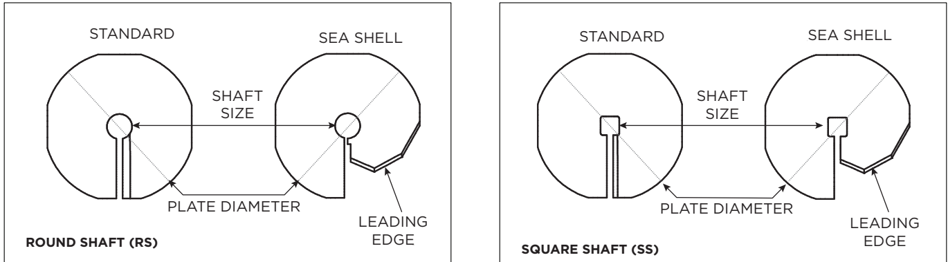
Projected Views Of Round Shaft And Square Shaft Helix Plates Figure 6-1
