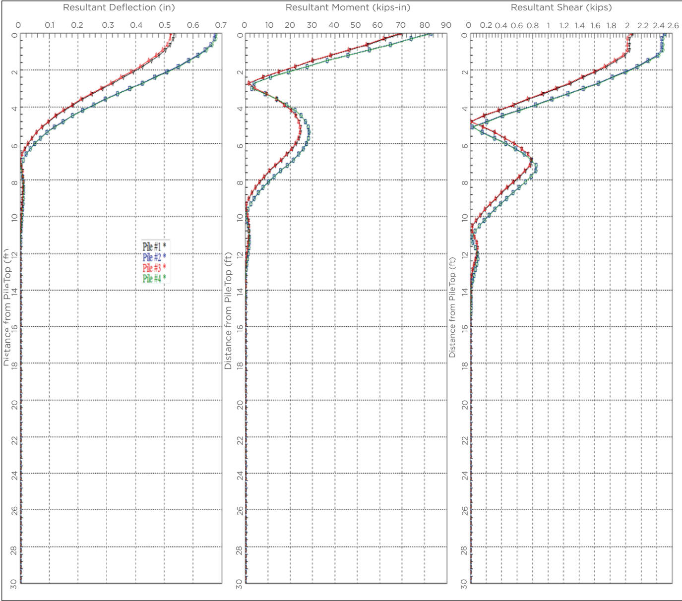
Resultant Deflection, Moment, and Shear Figure 7-7
