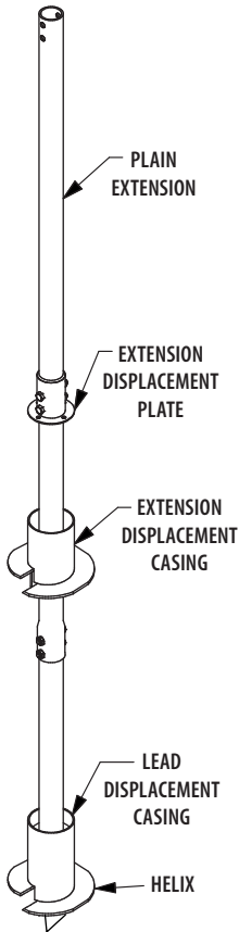
GROUTFORCE PILE ASSEMBLY, FIGURE 7-54
