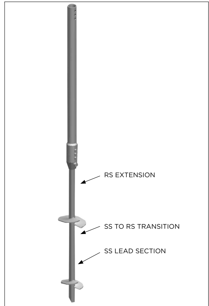
SS TO RS COMBINATION PILE FIGURE 5-26
