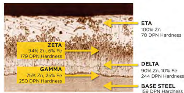
HDG Cross-Section
