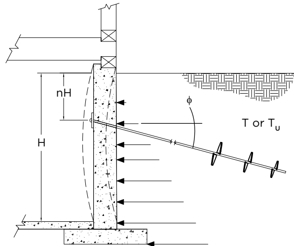
ESTIMATED TIEBACK FORCE REQUIRED FOR BASEMENT APPLICATIONS FIGURE 4-4
