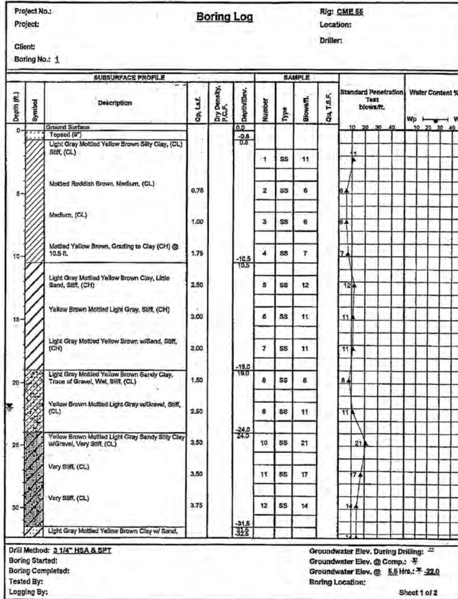
SAMPLE BORING LOG FIGURE 8-19
