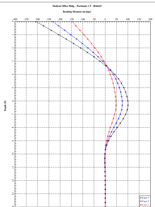
LPILE PLUS SAMPLE PLOT—BENDING MOMENT VS. DEPTH FIGURE 5-20
