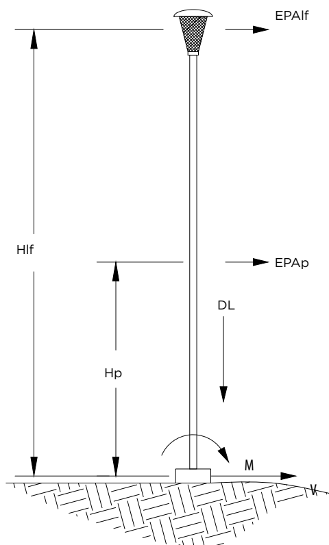
RESULTANT PILE FOUNDATION LOADS FIGURE 10-4
