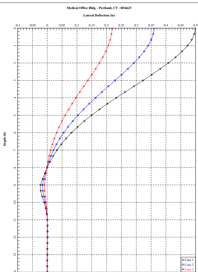
LPILE PLUS SAMPLE PLOT—DEFLECTION VS. DEPTH FIGURE 5-19
