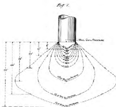
ASSUMED STRESS BULB UNDER PILE TIP FIGURE 6-3
