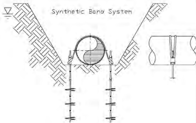
BAND SYSTEMS FIGURE 8-26
