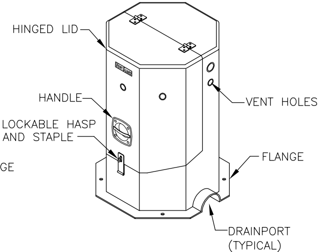
VENT GUARD
