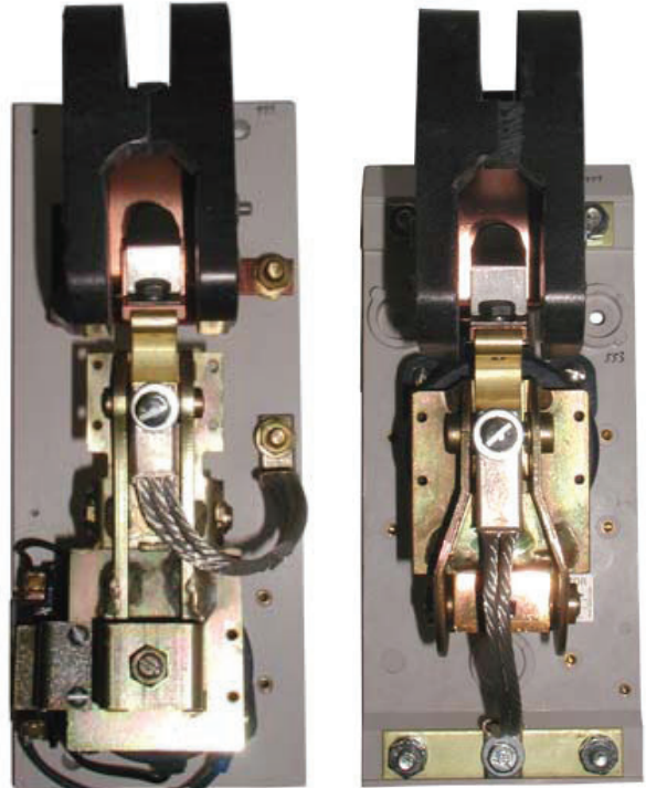
NEMA Size 3 Normally Closed
