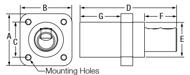
Bus Bar Type (Male Shown)
