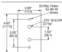
Configuration 456 Dual .375" (9.5) Round (Box Mount)
