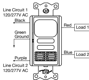
Two Circuit Sensor, Wired for Two Loads
