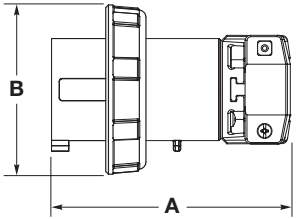
Short Housing Plug
