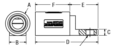
Angled Style
