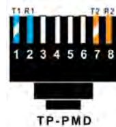
8 Position / 4 Wire
