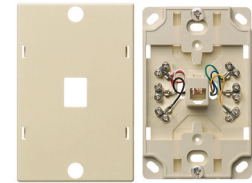
Wall Phone Jack, 6-Position, 6-Conductor, Screw Terminations
