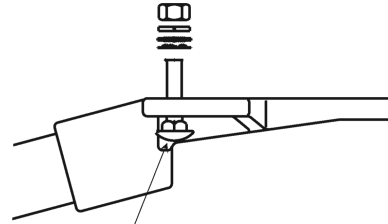
1/2" - 13 x 2" Captive Carriage Bolt
