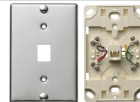
Wall Phone Jack 6-Position 4-Conductor Screw Termination
