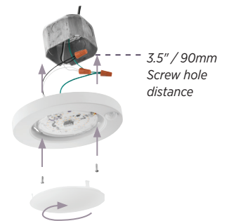
Installation Sequence
