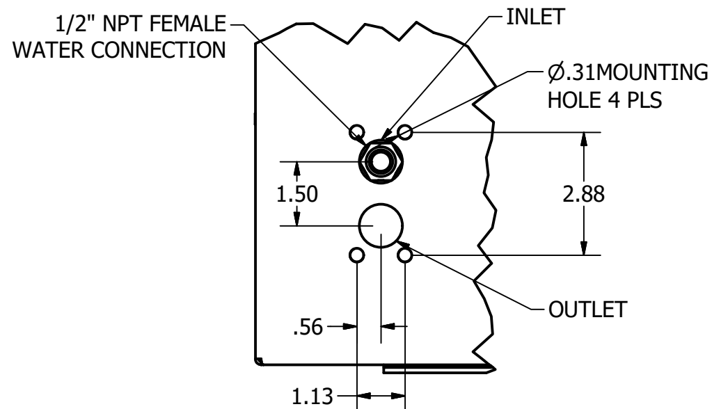
DETAIL A STANDARD PLUMBING
