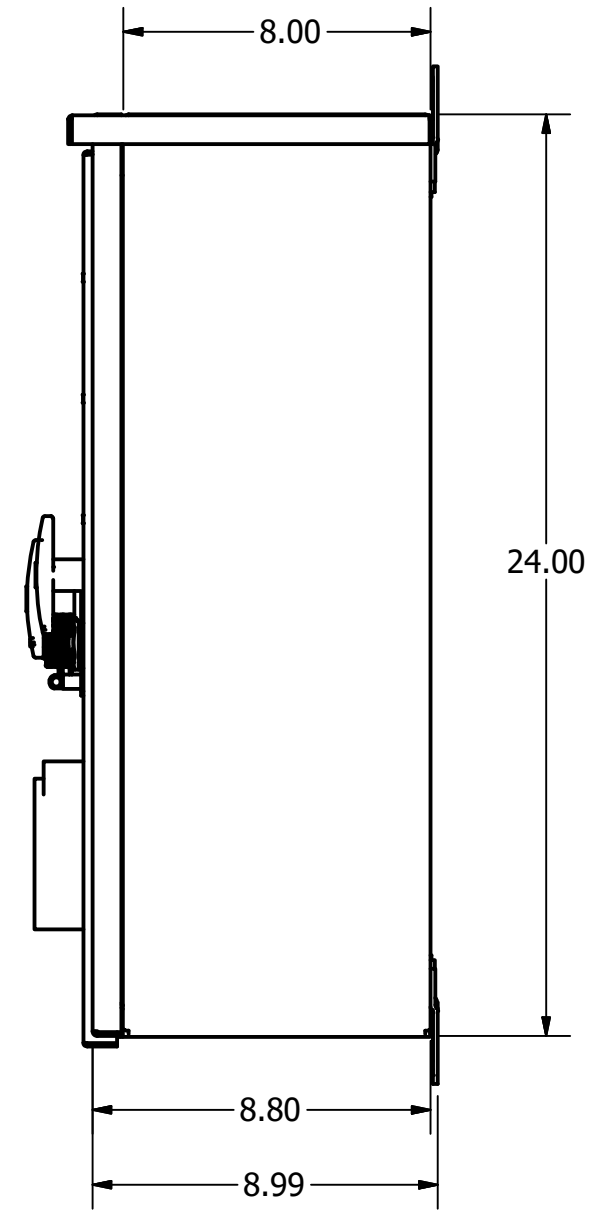
SIDE VIEW
