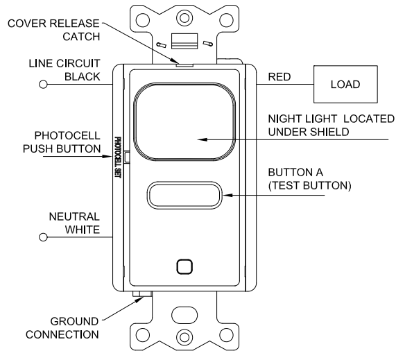
FIGURE 1 - WIRING DIAGRAM
