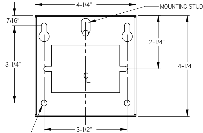
WALL BRACKET DETAIL
