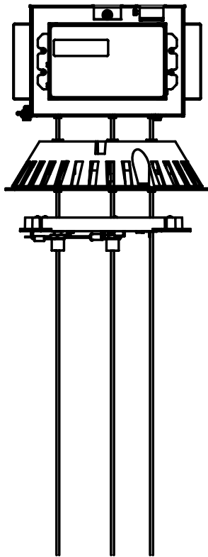
J-box/Cable Kit Assembly with mounting hardware SCALE 1 : 5
