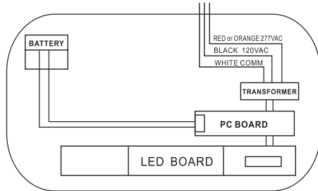
BATTERY BACKUP WIRING DIAGRAM:
