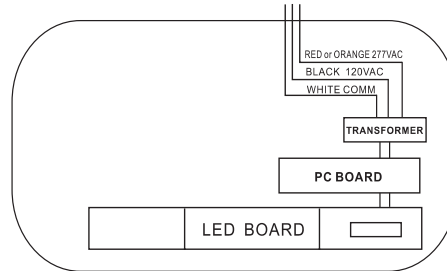
AC ONLY WIRING DIAGRAM:
