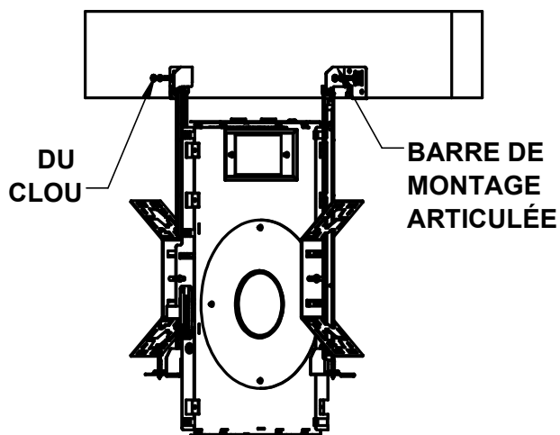
FIGURE 4 SOLIVE EN BOIS
