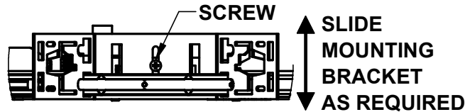
FIGURE 5 MOUNTING BRACKET ADJUSTMENT
