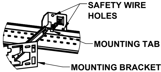
FIGURE 3 SUSPENDED CEILING
