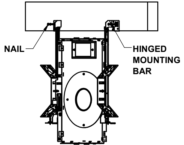
FIGURE 4 WOOD JOIST
