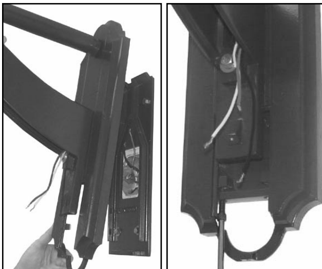
6. Attach wall mount cover plate with arm and fixture head attached, to wall plate with two (2) \frac{5}{16} -18 x 1\frac{1}{4} " socket head cap screws. Connect fixture wires to supply wires observing polarity, i.e.; green-to-ground, white-to-common, and black-to-voltage. (See fixture installation instructions.)
