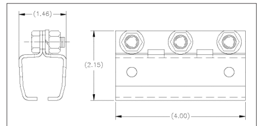
TRACK SPLICE C35-TSA Wgt: 1.00 lbs
