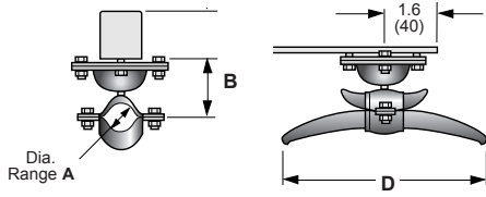
ROUND CABLE FIXED CLAMP
