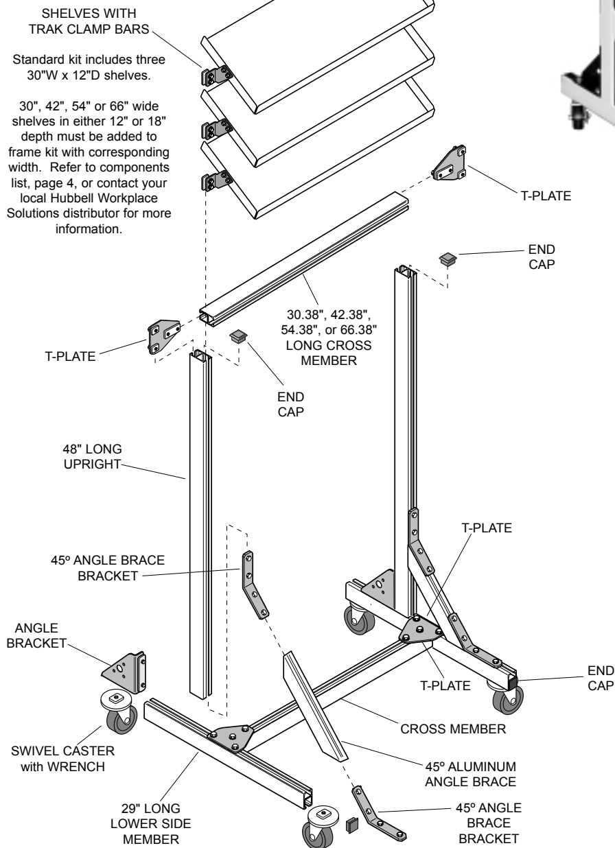
Figure 1. COMPONENTS
