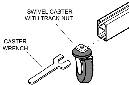
Figure 9 INSTALLING CASTERS
