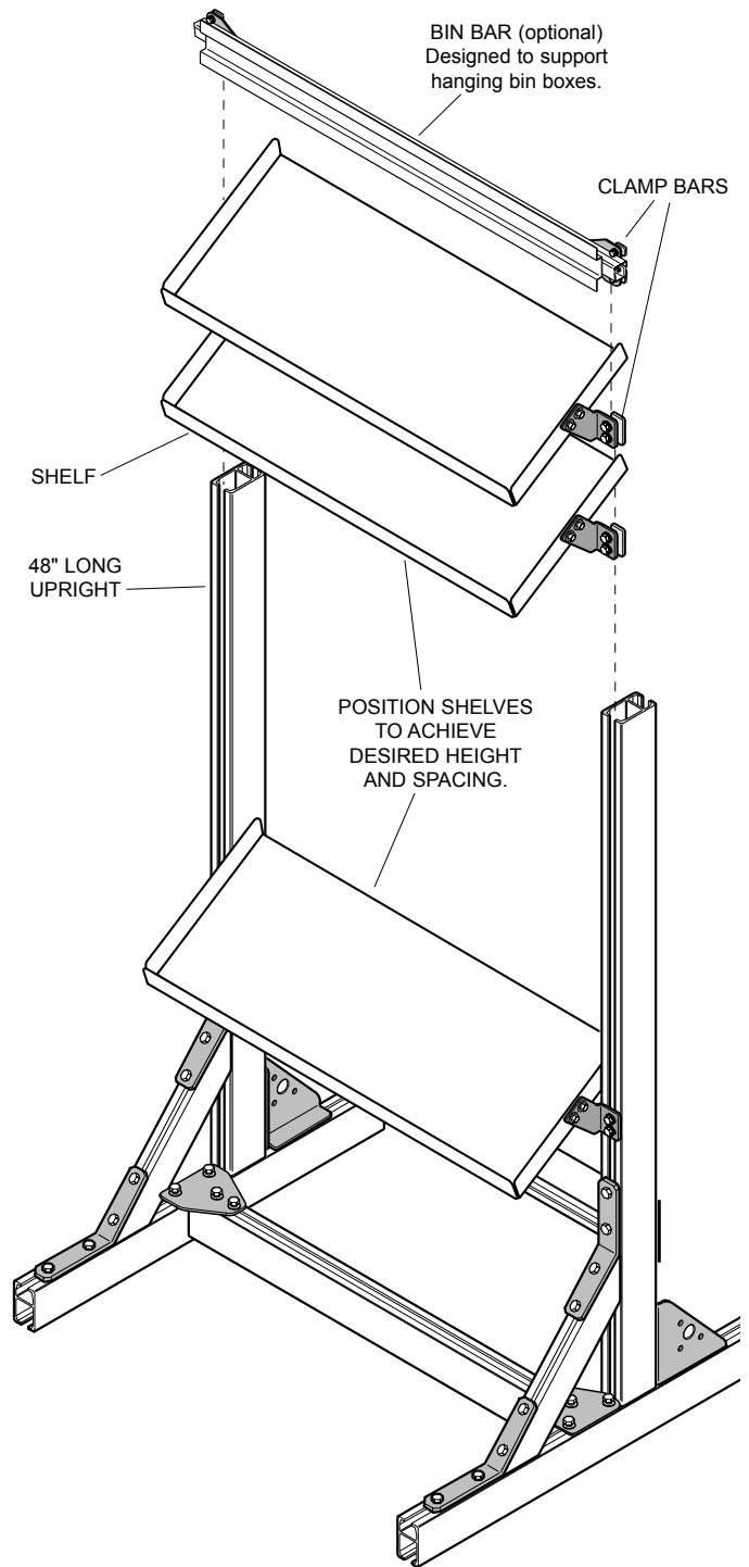
Figure 8. ATTACHING SHELVES
