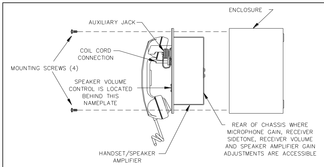
Figure 1. Installation and Adjustment Details
