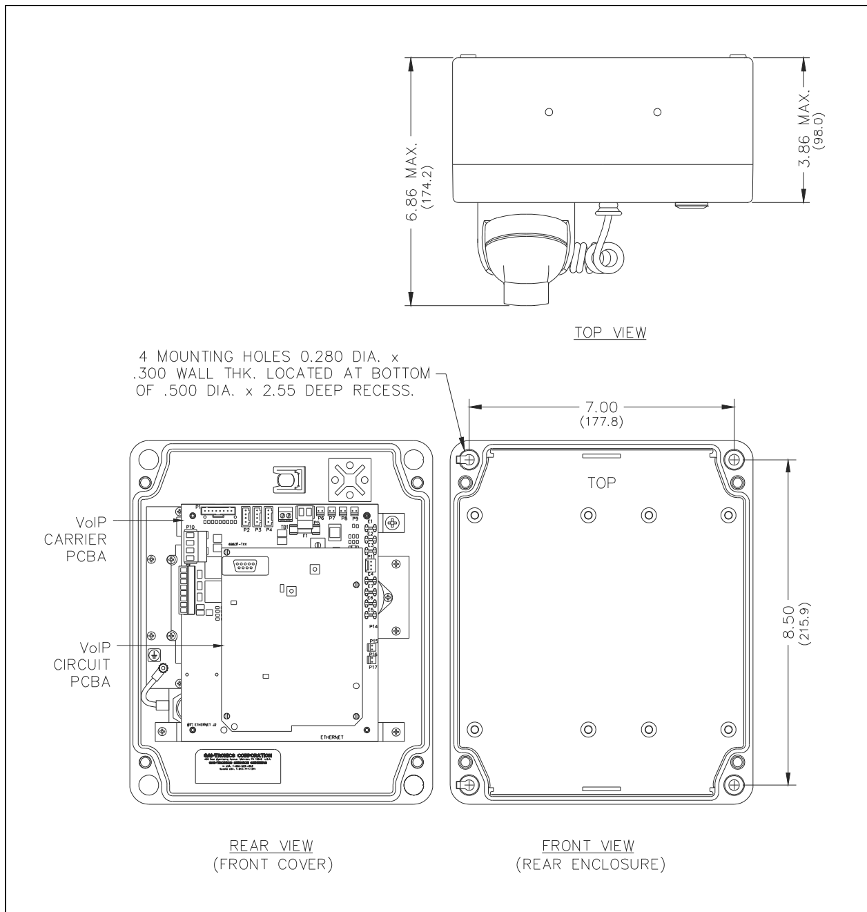
Figure 10. Model 247-700 Mounting Detail
