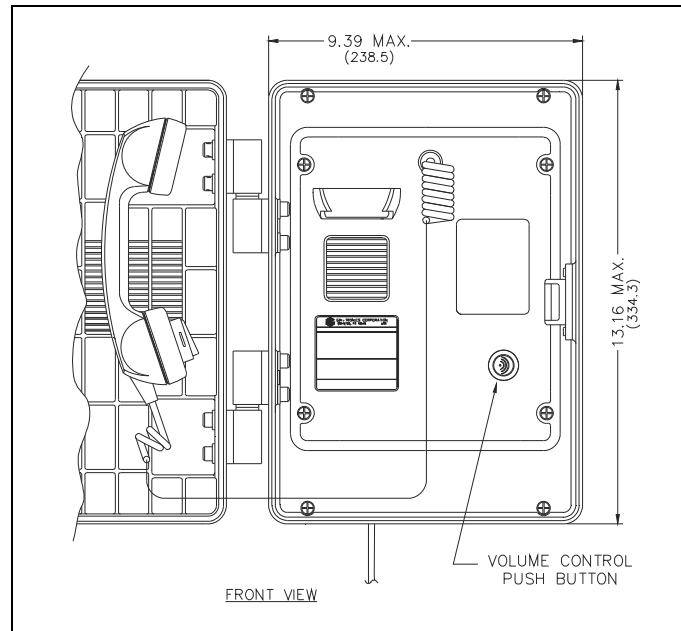
Figure 11. Model 257-700 VoIP Autodial Telephone (Front door open)
