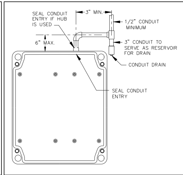
Figure 2. Model 247-700 & 257-700—Top entry conduit installation details— (NOT RECOMMENDED)
