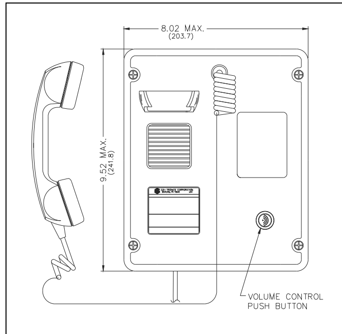
Figure 9. Model 247-700 VoIP Autodial Telephone
