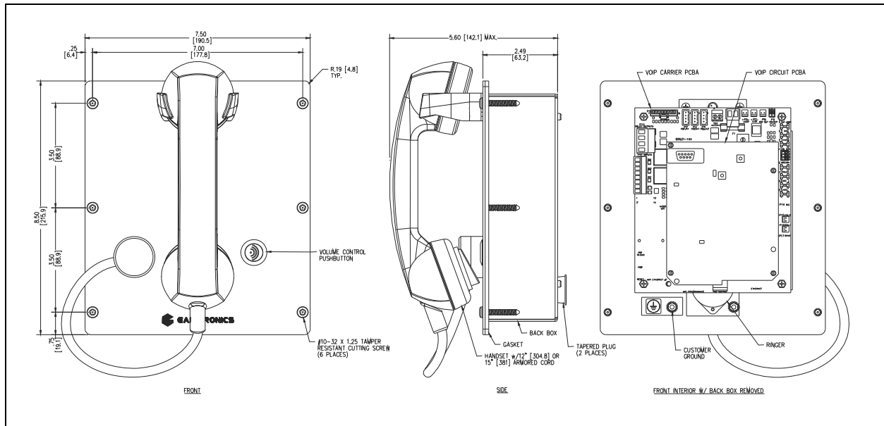
Figure 15. Models 277-702BH/-702BHAC Behavioral Health Telephone
