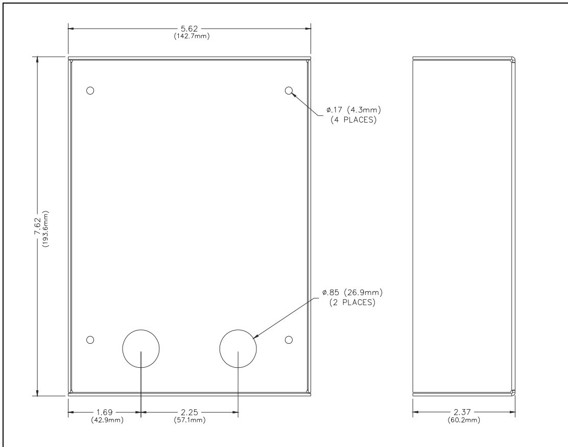
Figure 16. Models 277-702BH/-702BHAC Dust Cover Detail
