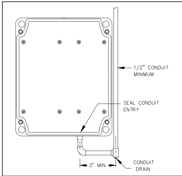
Figure 1. Model 247-700 & 257-700—Bottom entry conduit installation details
