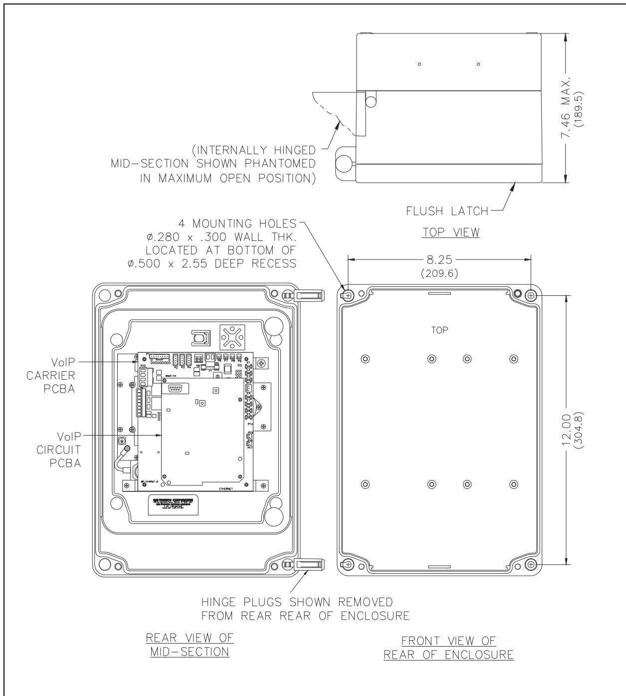
Figure 12. Model 257-700 Mounting Detail
