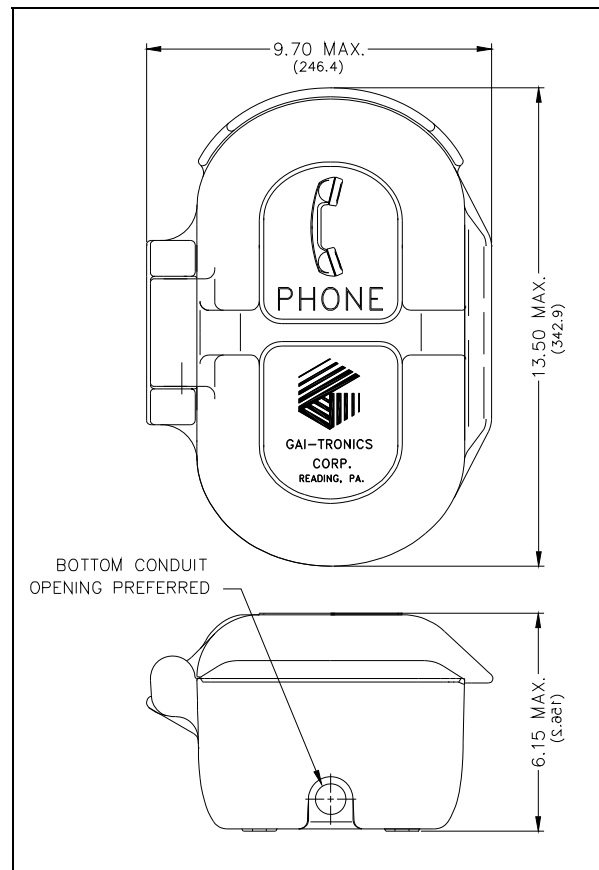
Figure 7. Model 227-700 Outline
