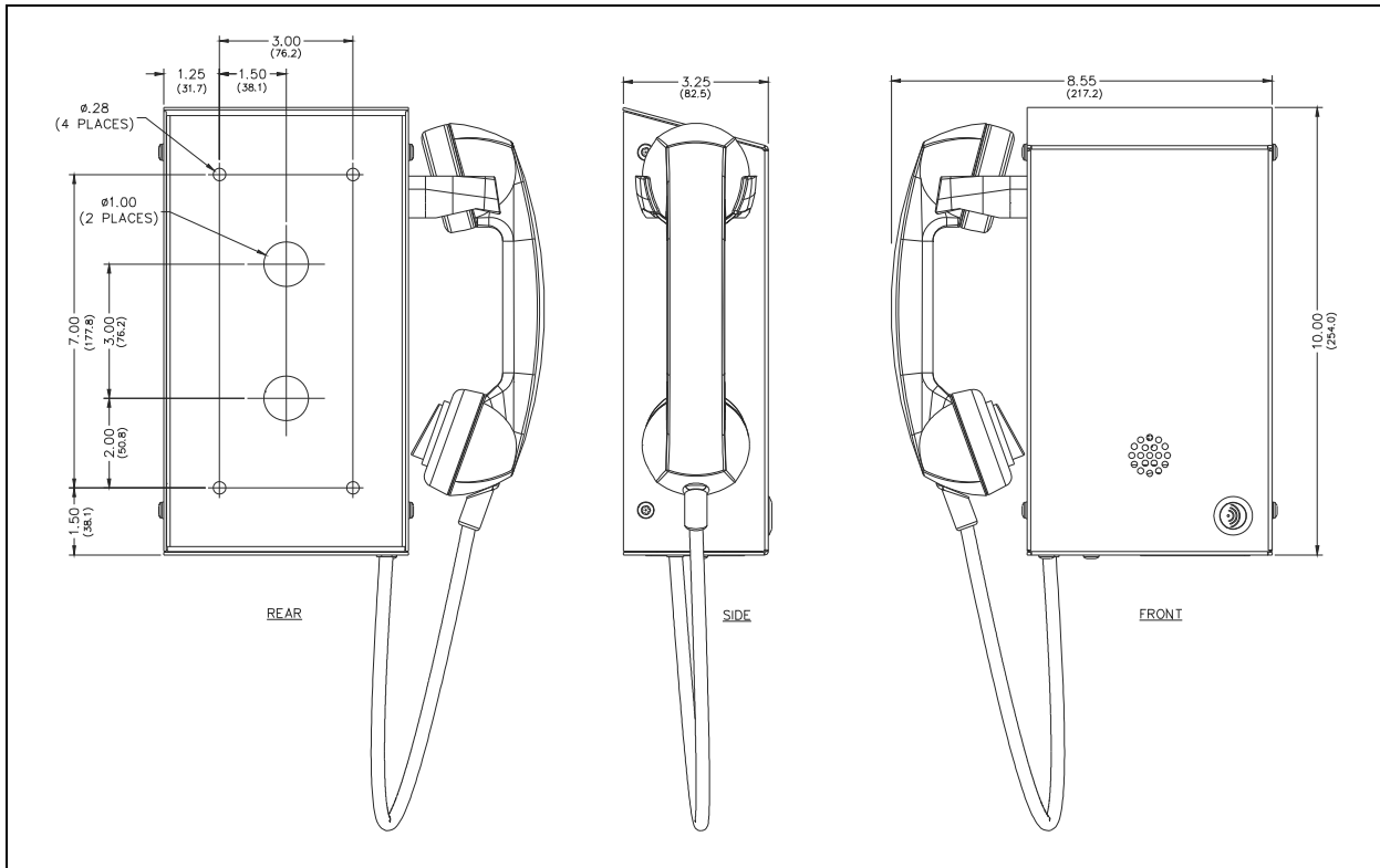
Figure 3. Models 210-702/-702BH/-702BHAC VoIP Autodial Behavioral Telephones Outline and Mounting Detail
