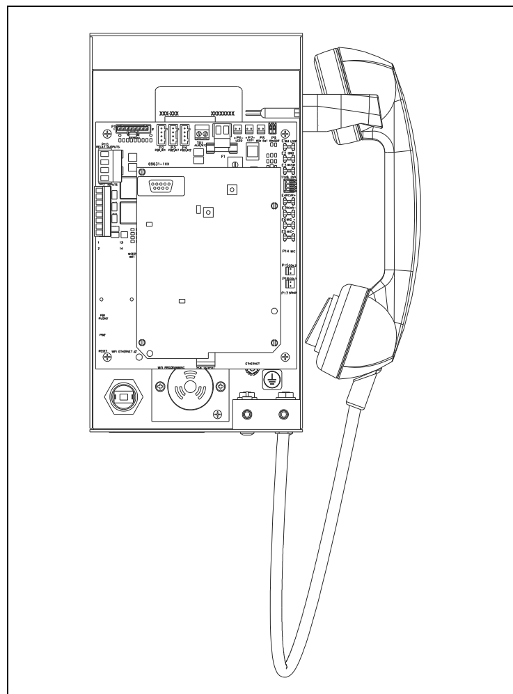
Figure 5. Models 210-702/-702BH/-702BHAC Internal View
