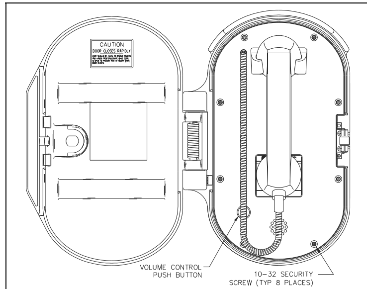
Figure 6. Model 227-700 VoIP Autodial Telephone with spring loaded door in the open position
