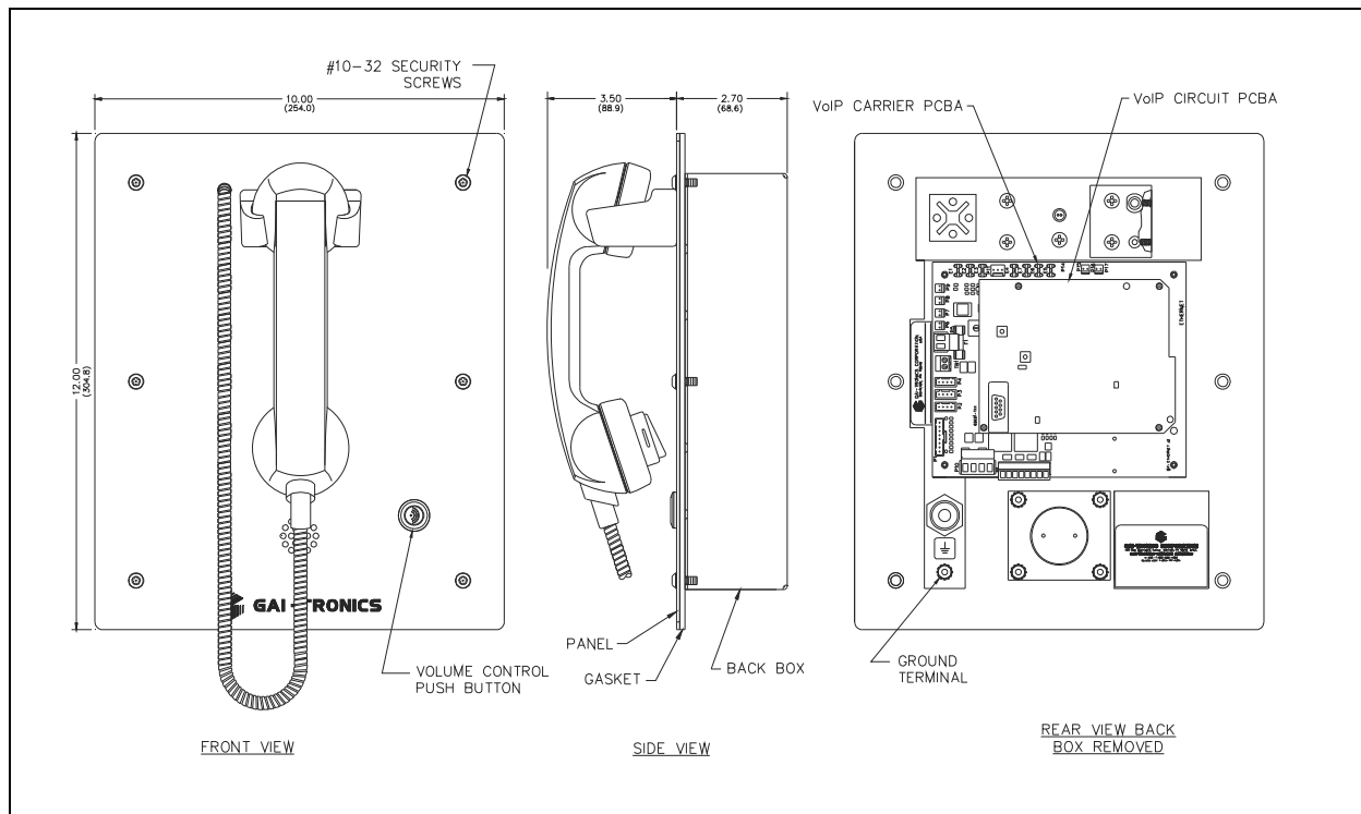
Figure 13. Model 277-700 Outline Drawing
