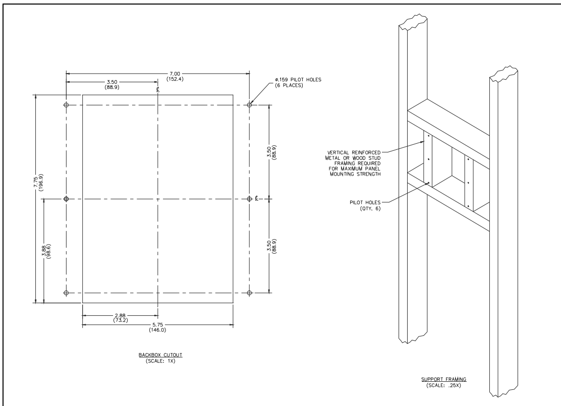
Figure 17. Models 277-702BH/-702BHAC Cutout and Support Framing Detail
