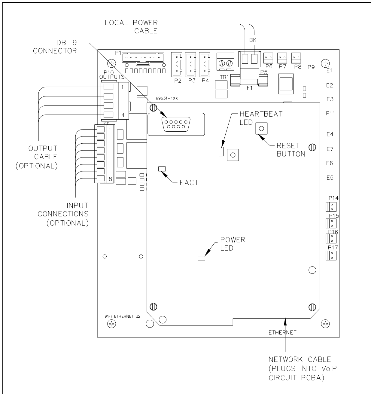
Figure 18. VoIP Telephone PCB Assembly
