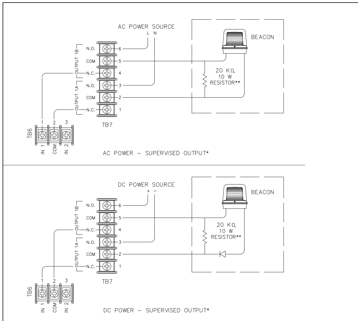
Figure 14. Supervised Output Wiring with SmartSeries® Option
