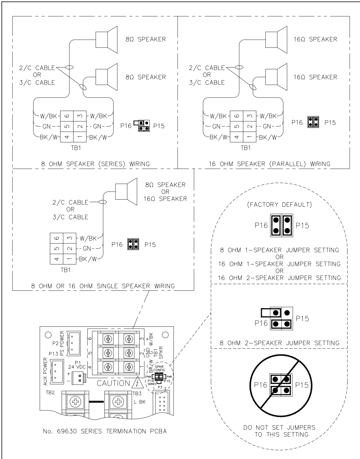
Figure 5. Jumper Configuration for 8-ohm or 16-ohm Speaker Impedance
