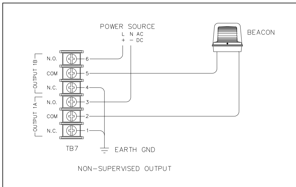
Figure 13. Non-supervised Output with the VLC or SmartSeries® Option
