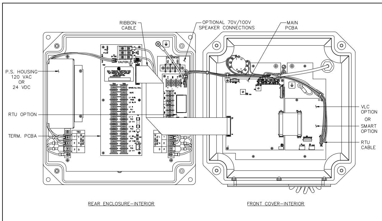
Figure 2. ICS Zone 2/22 Weatherproof Page/Party® Station Interior View (AC Version shown)
