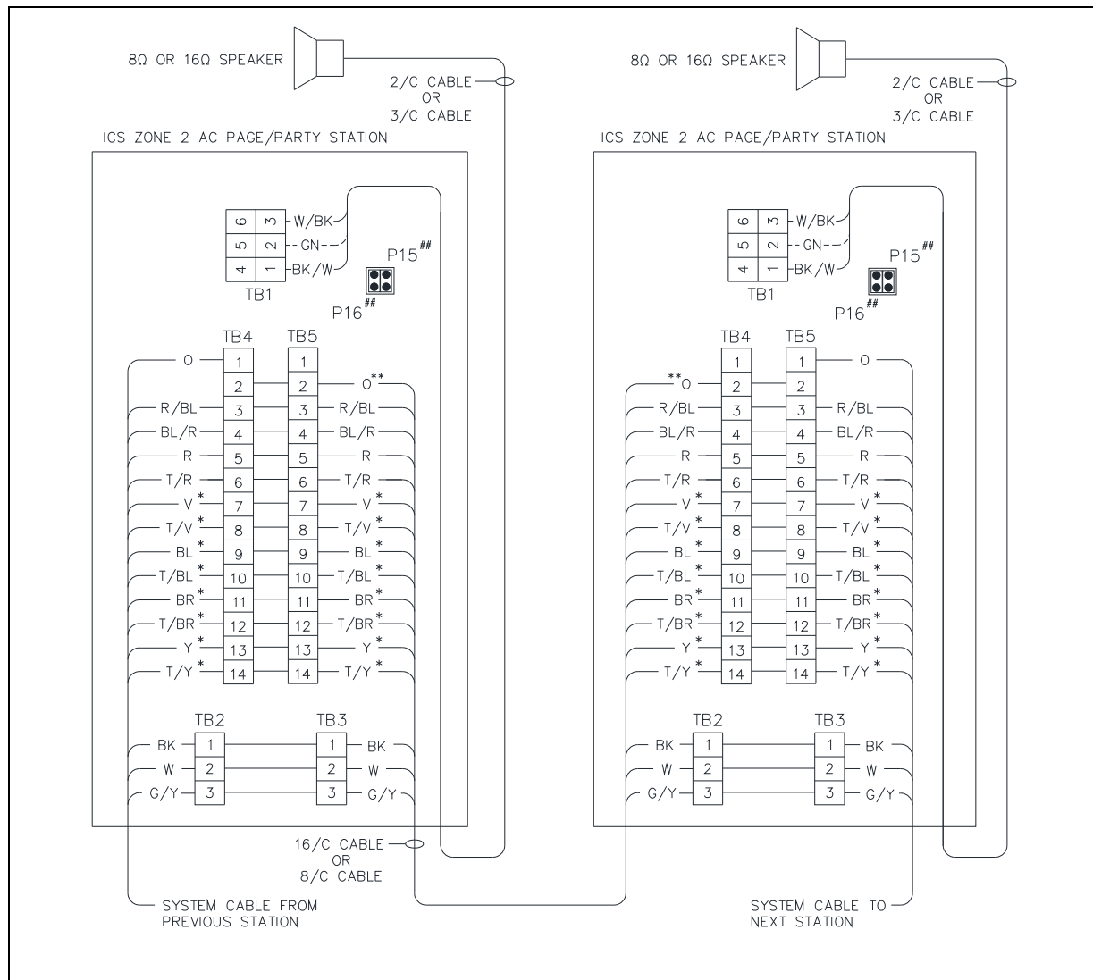
Figure 4. Typical Page/Party® ICS Station Wiring Diagram
