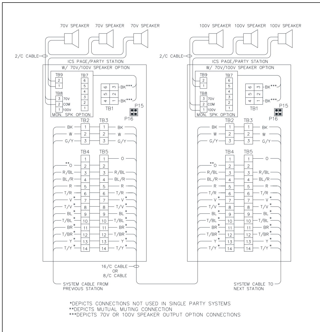
Figure 20. 70V/100V Monitored Speaker Connections
