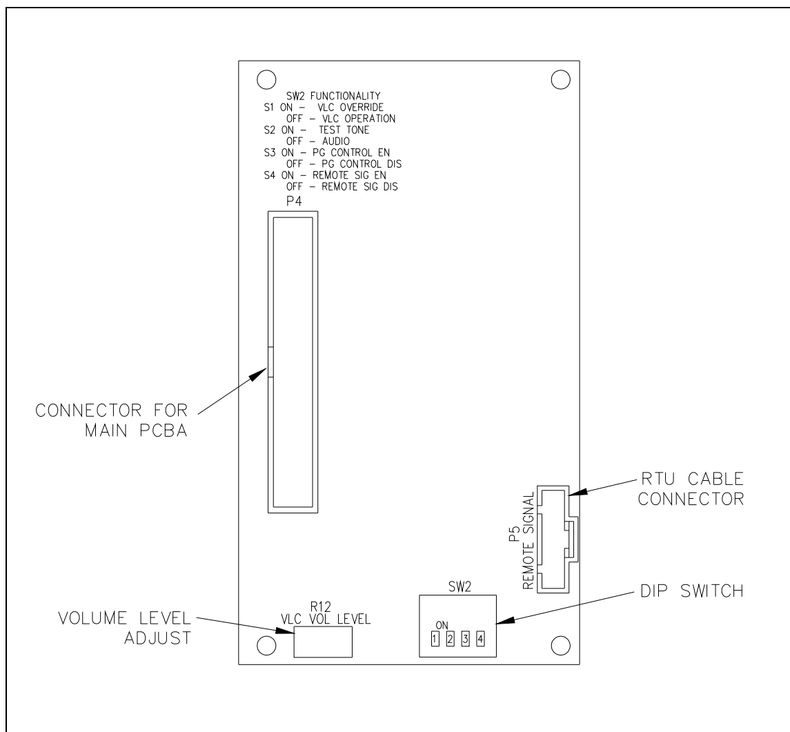
Figure 10. 69553 Series VLC PCBA
