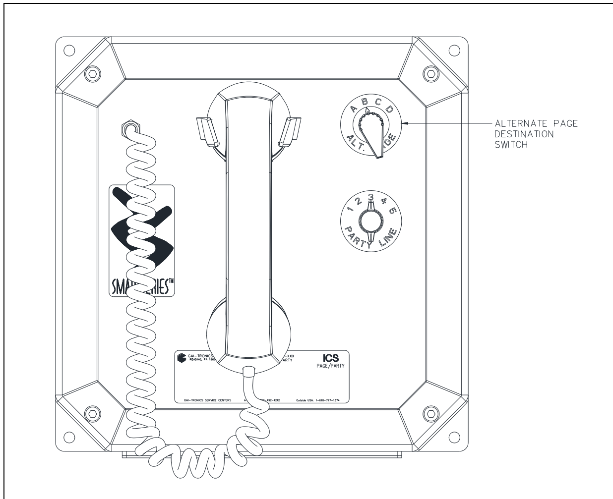
Figure 9. Alternate Page Selection Switch Location
