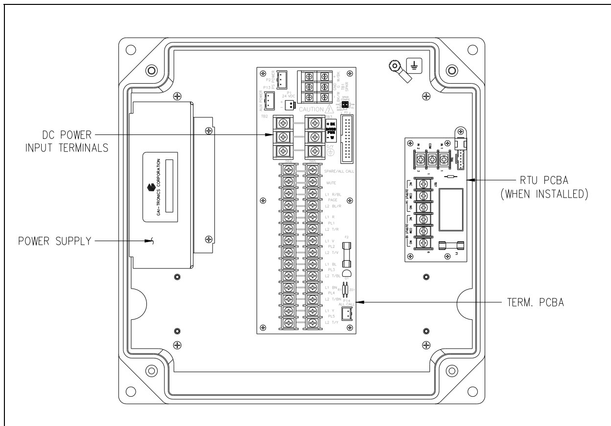
Figure 16. DC Option—Interior View
