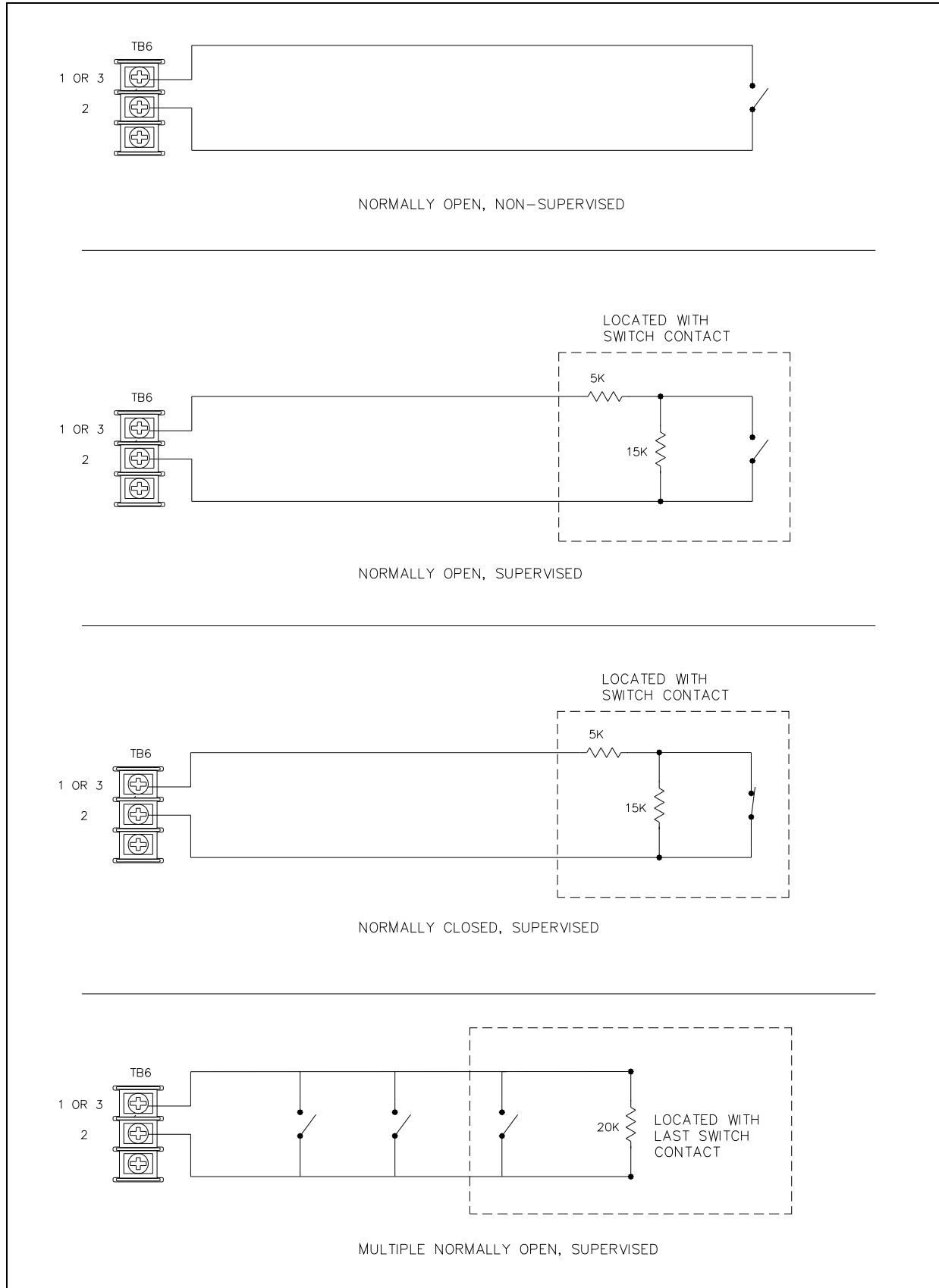
Figure 15. Input 1 or 2 Wiring Configuration with the SmartSeries® Option
