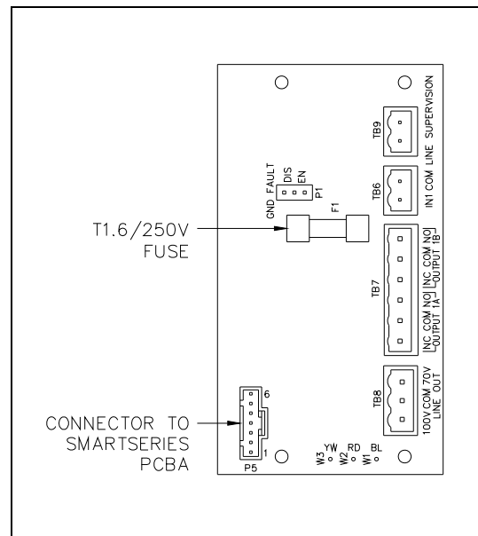
Figure 12. 69628 Series RTU & SmartSeries® 70V/100V Speaker Line Monitor PCBA
