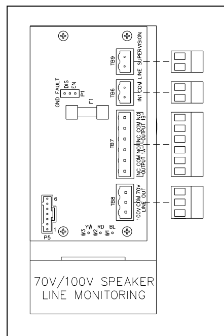
Figure 18. SmartSeries® Station 70V/100V Speaker Line Monitor Assembly
