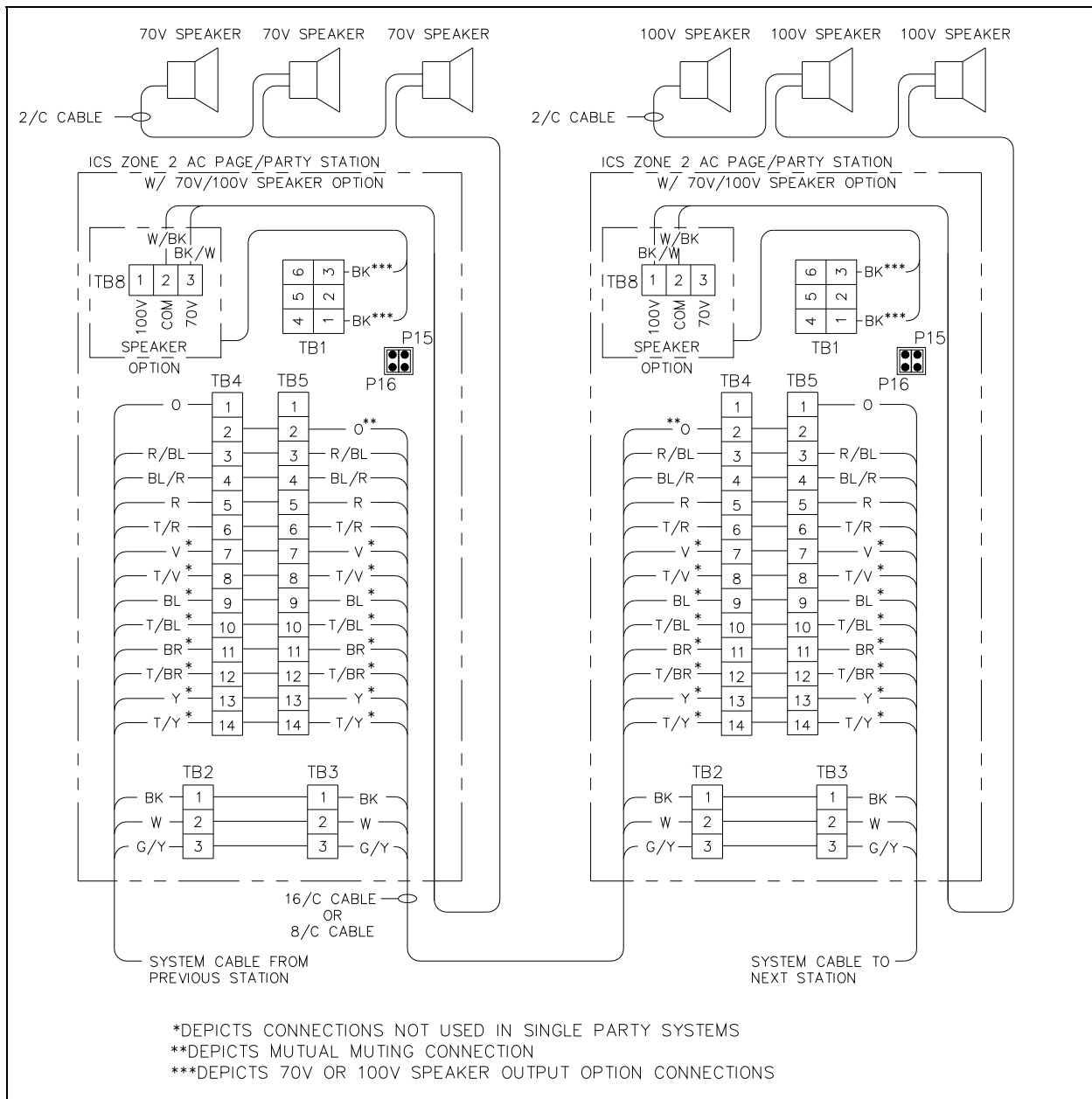
Figure 19. 70V / 100V Speaker Connections
