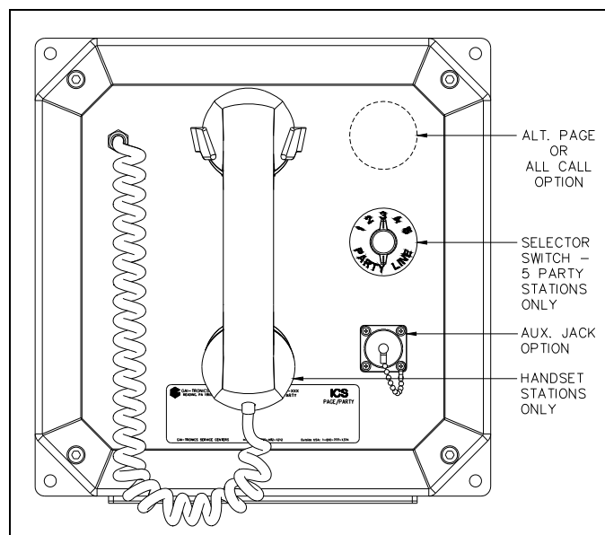
Figure 1. ICS Zone 2/22 Weatherproof Station Exterior Front Panel with all options
