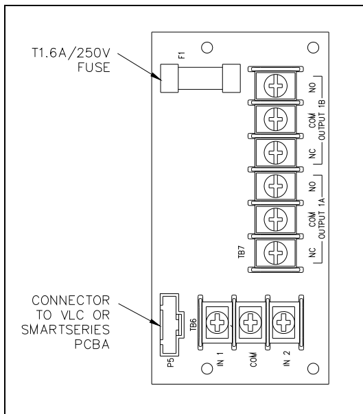
Figure 11. 69627 Series RTU PCBA
