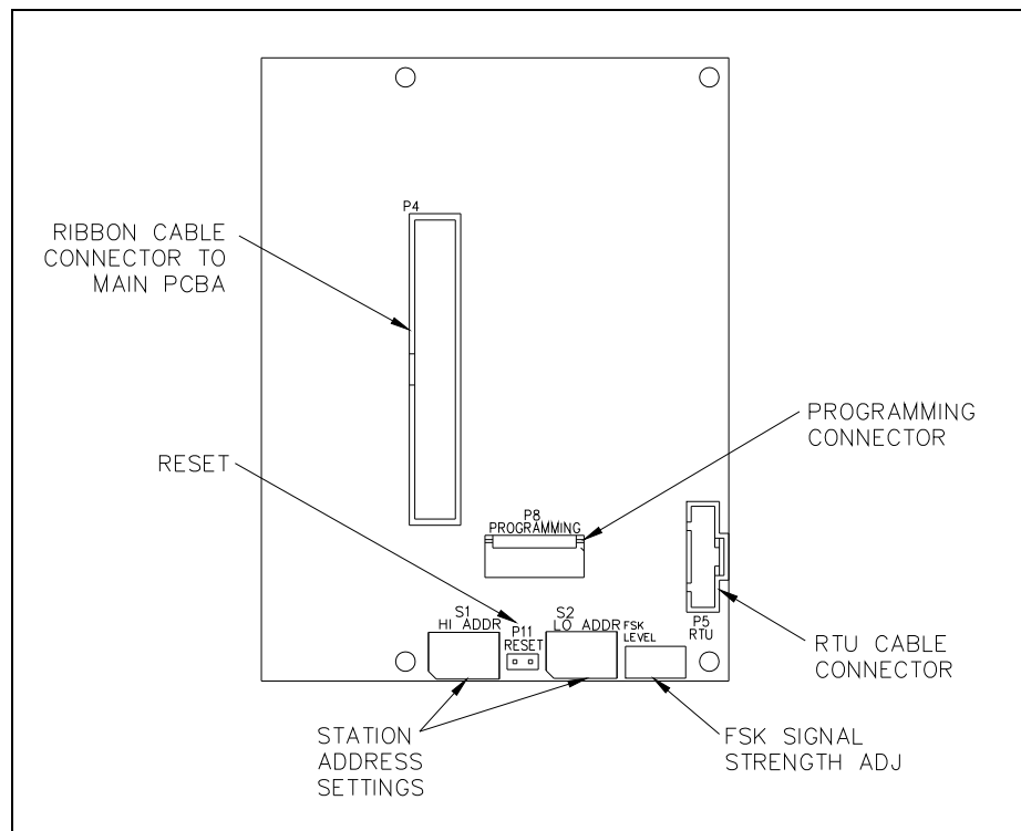
Figure 7. 69552 SmartSeries® PCBA
