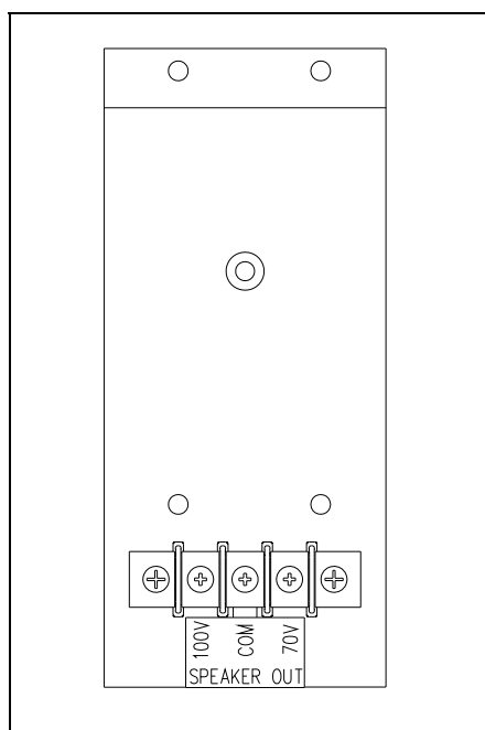
Figure 17. Standard Station 70V/100V Speaker Output Assembly
