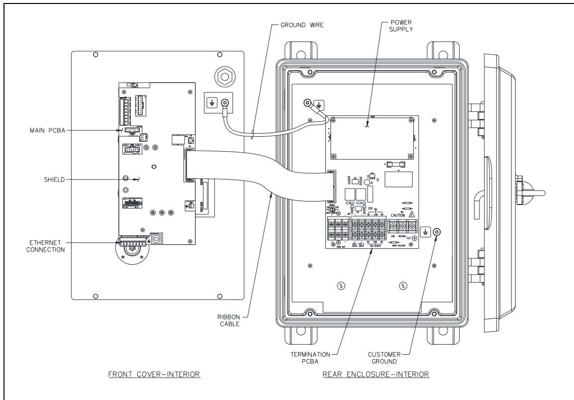
Figure 9. SP2 Weatherproof Class I Div. 2—Interior View
