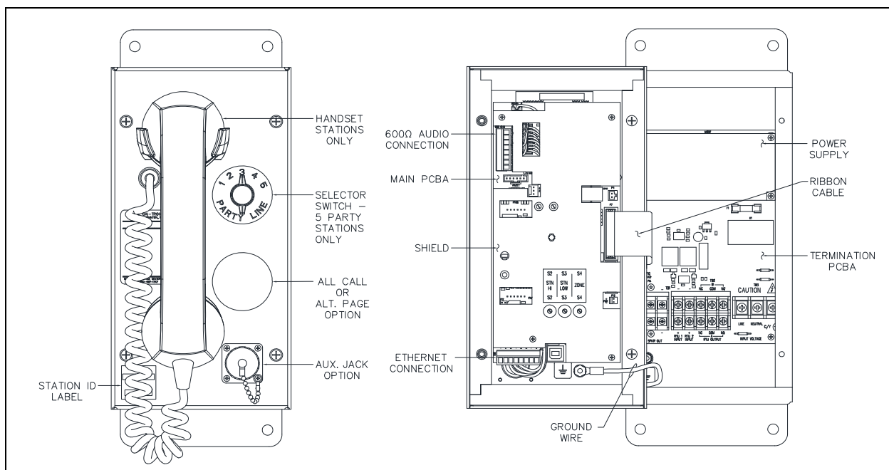
Figure 1. HUBBCOM Handset/Speaker Amplifier Station
