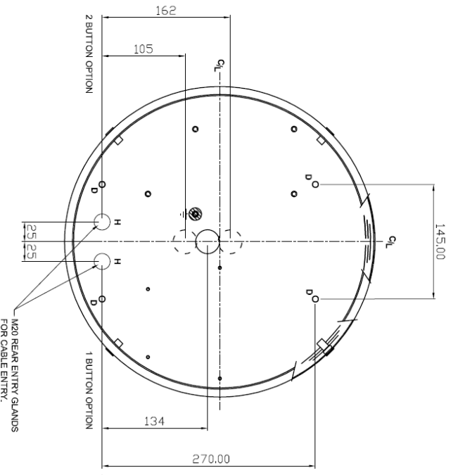
INTERNAL VIEW REAR CASE (COVER REMOVED)
