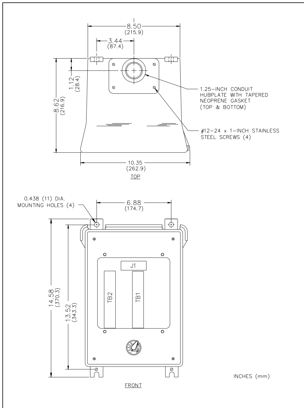
Figure 3. Model 7325-102 Weatherproof Aluminum Enclosure Mounting Details
