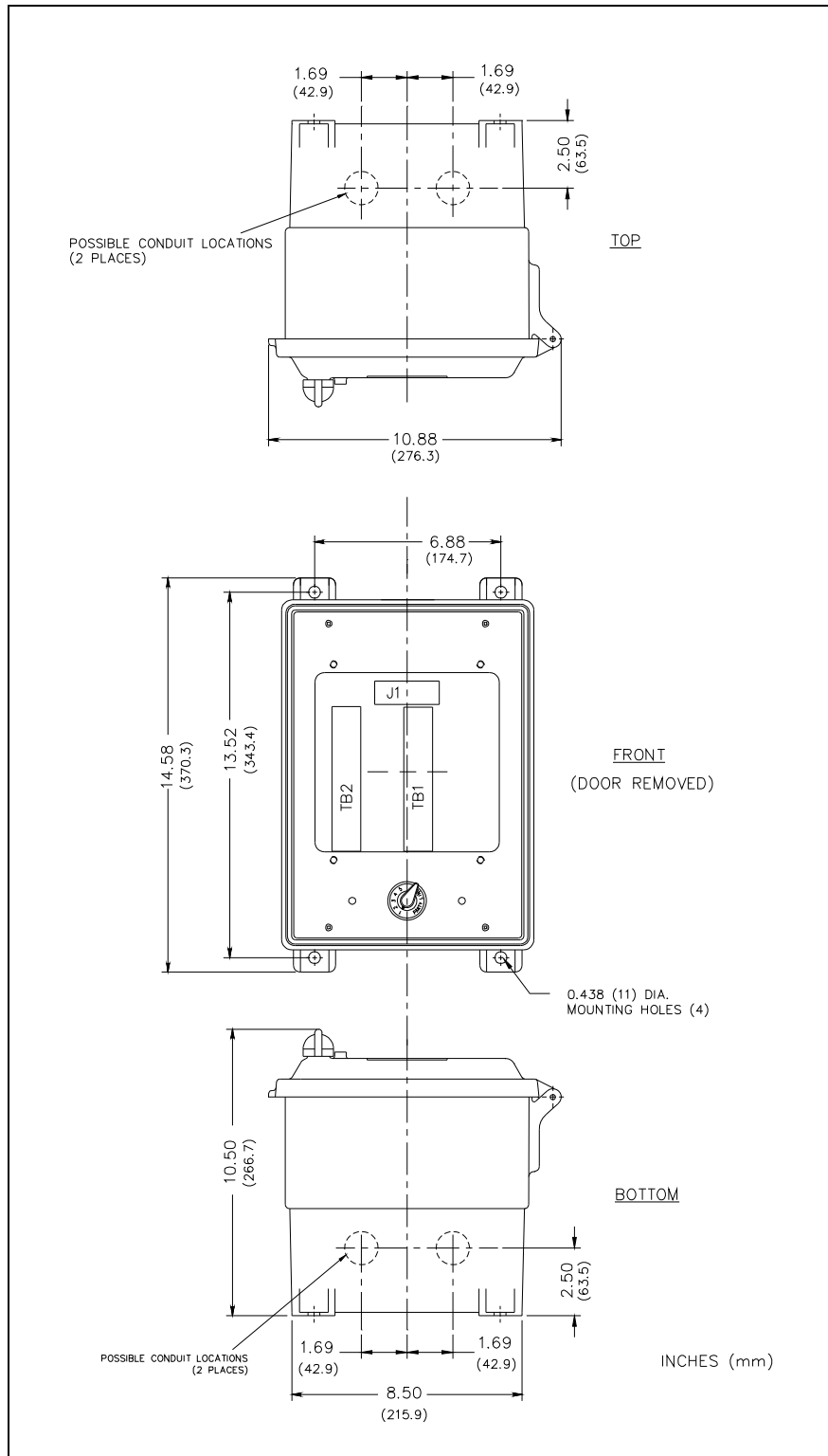
Figure 2. Model 7335-002 Outdoor Enclosure Mounting Details
