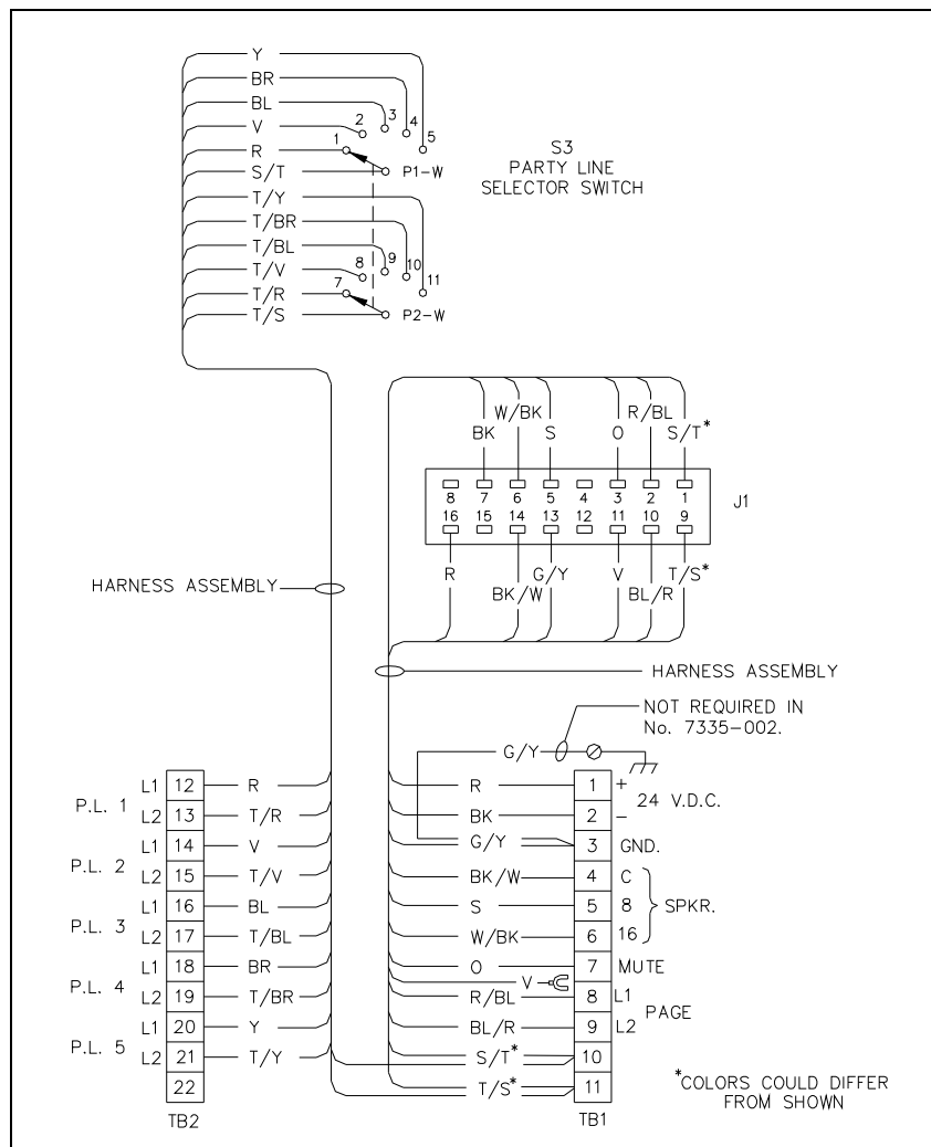
Figure 4. Wiring Diagram
