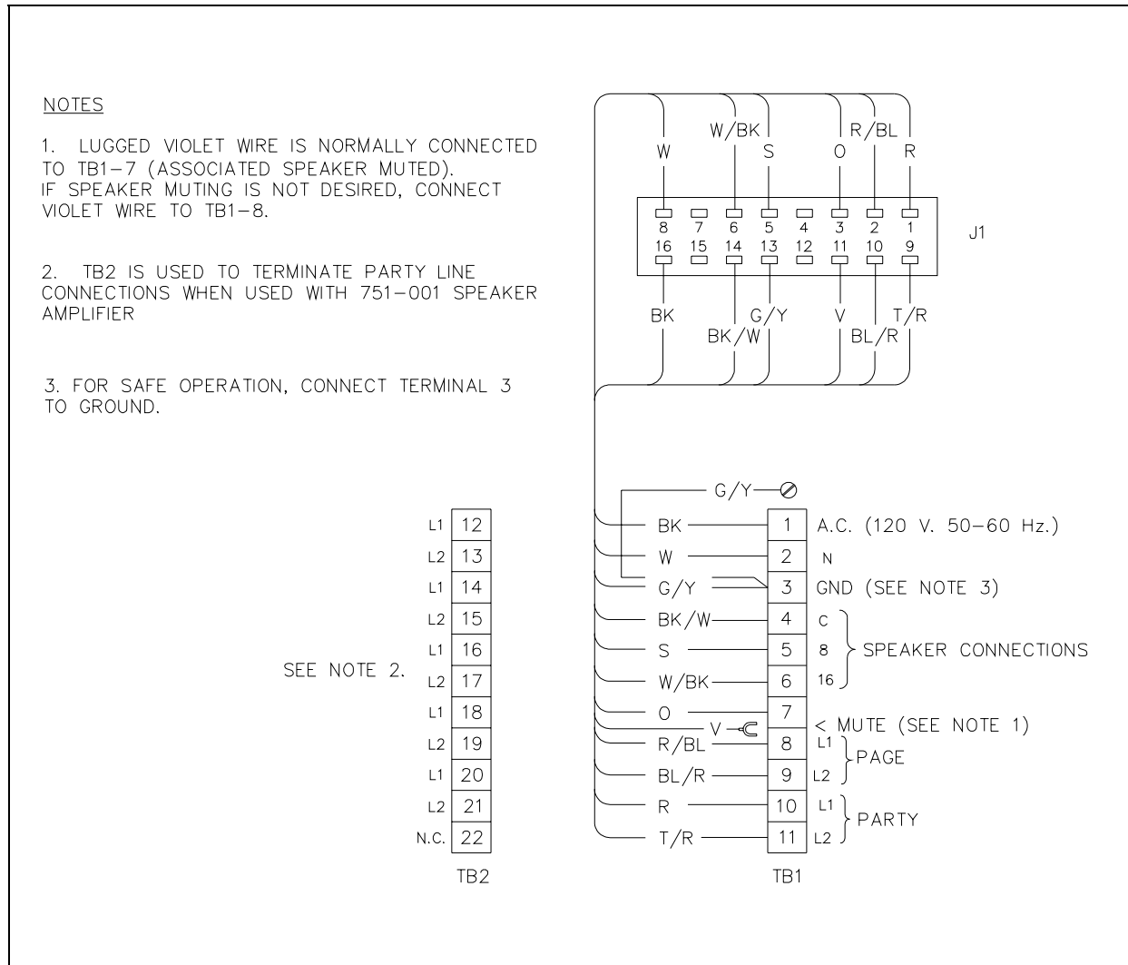
Figure 2. Wiring Diagram
