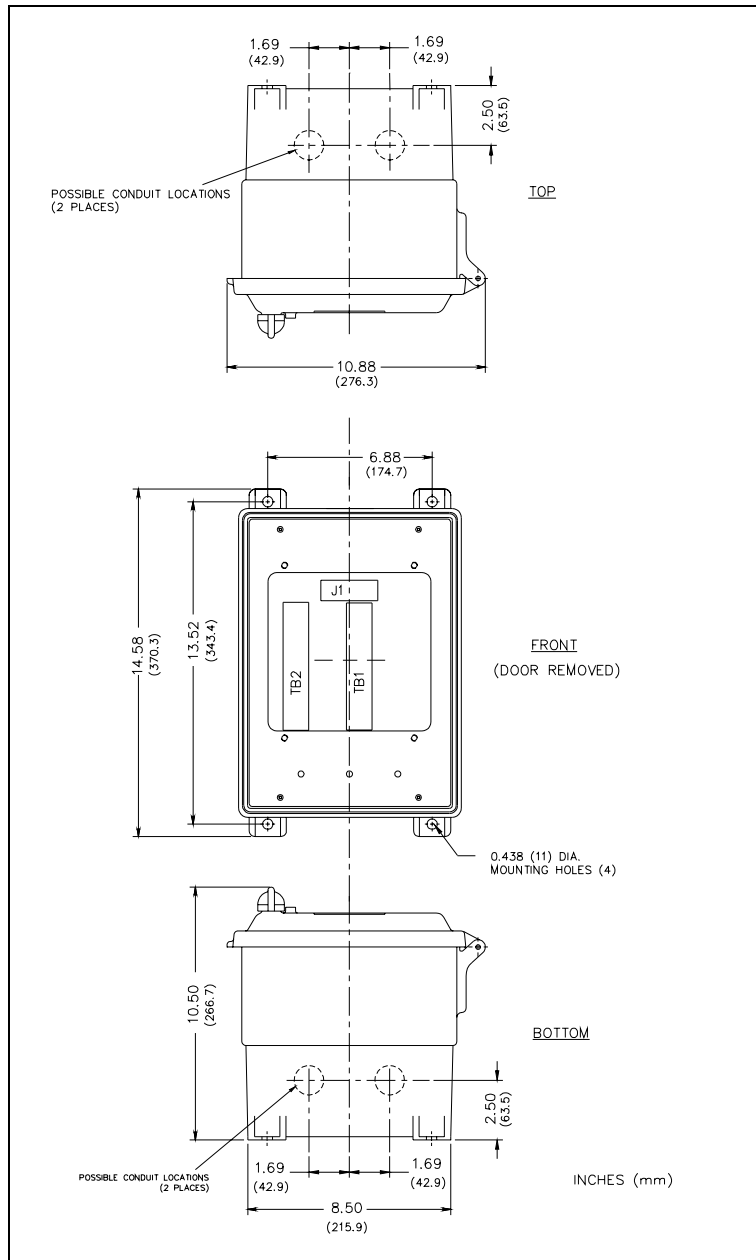
Figure 1. 733-001 Single-Party Weatherproof Non-Metallic Enclosure Mounting Details
