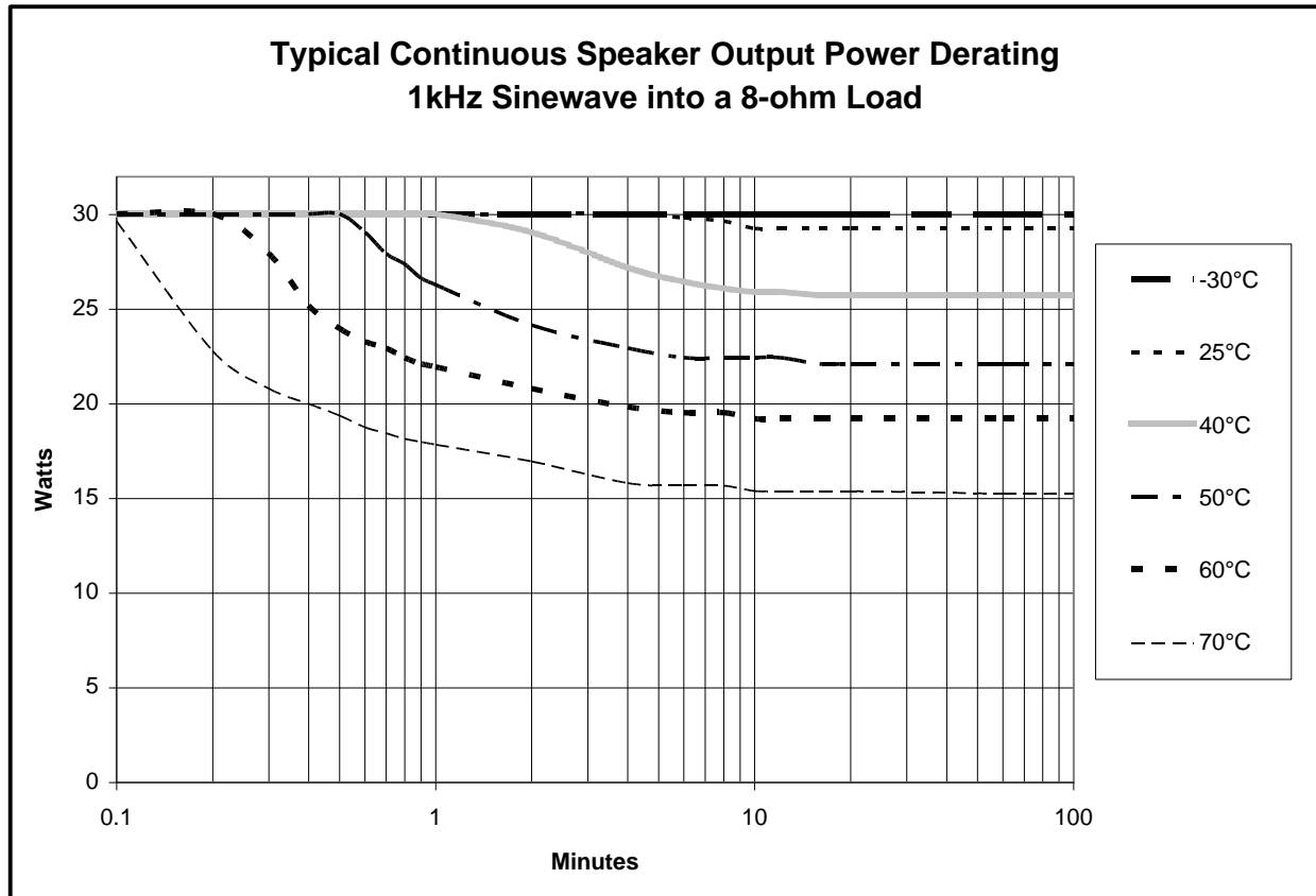
Figure 22. Typical Continuous Speaker Output Power Derating 1 kHz Sine Wave into an 8-ohm Load
