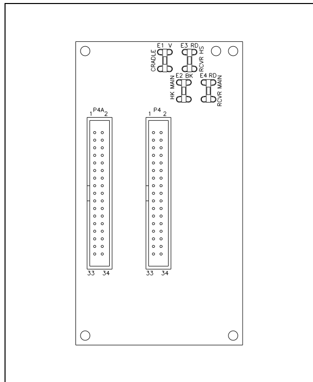
Figure 20. RF Hookswitch
