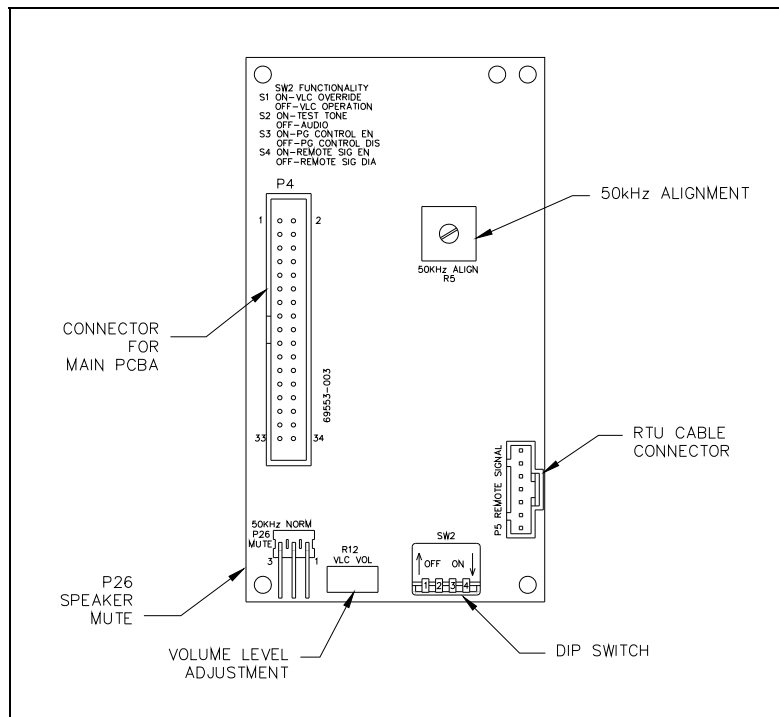
Figure 10. No. 69553 Series VLC PCBA
