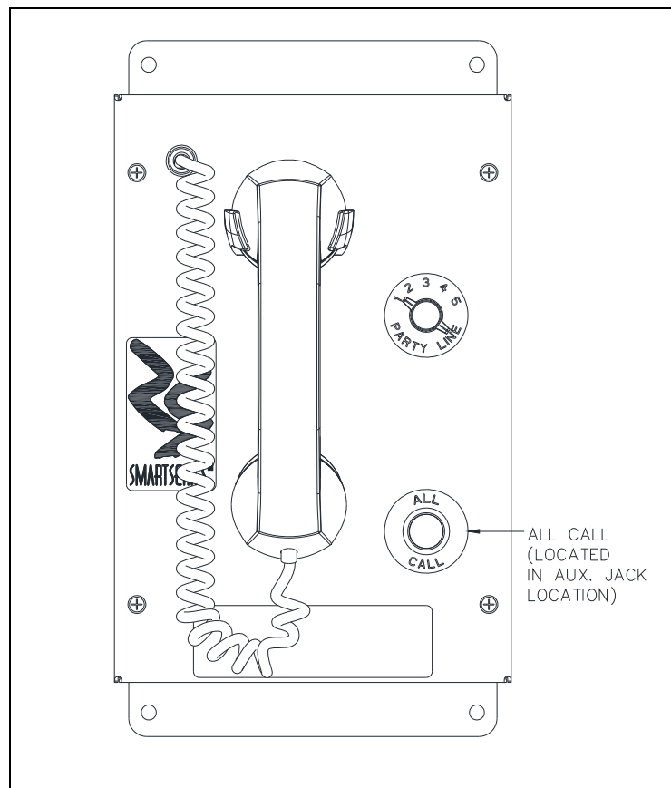
Figure 8. All-Call Selector Switch Location
