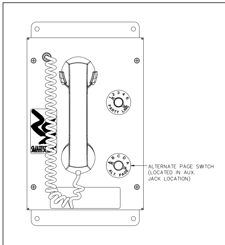
Figure 9. Alternate Page Selector Switch Location
