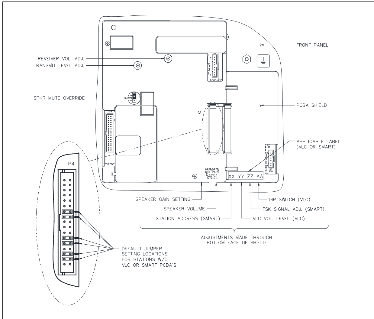
Figure 21. P4 Jumper Default Settings
