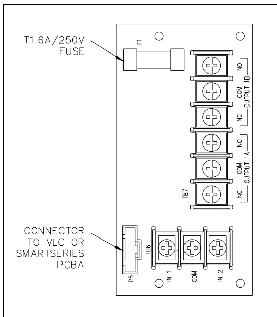
Figure 11. No. 69627 Series RTU PCBA
