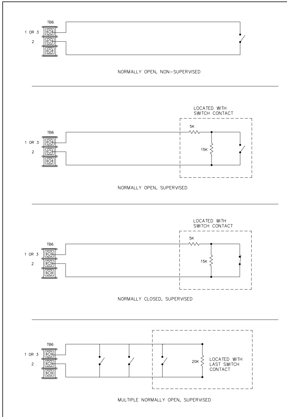
Figure 15. Input One or Two Wiring Configuration with the SmartSeries® Option
