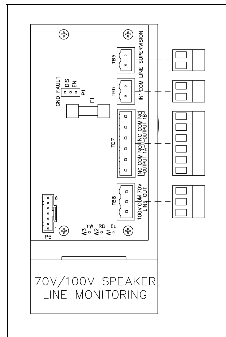
Figure 17. SmartSeries® Station 70V/100V Speaker Line Monitor Assembly
