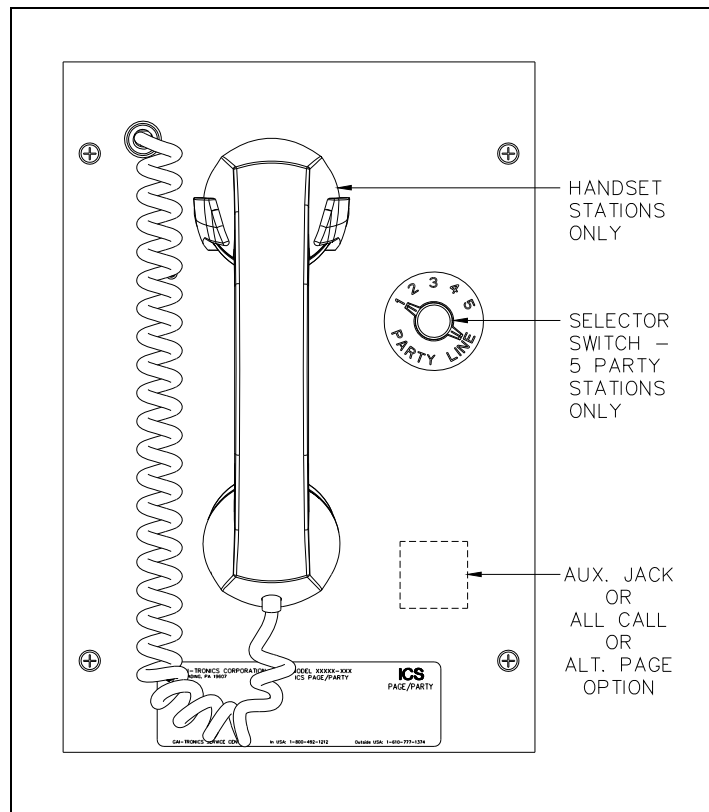
Figure 1. ICS Station Front Panel with all options
