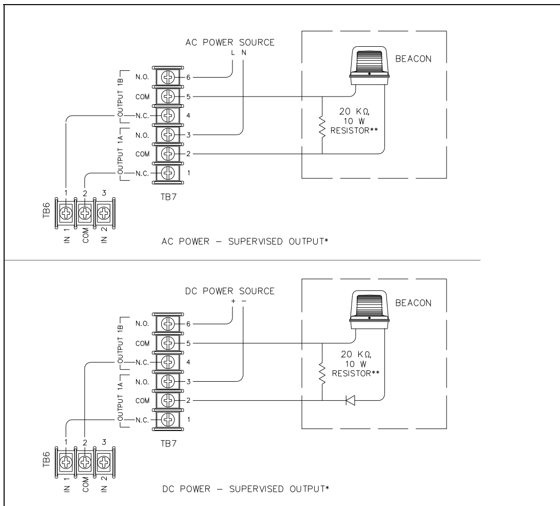
Figure 14. Supervised Output Wiring with SmartSeries® Option
