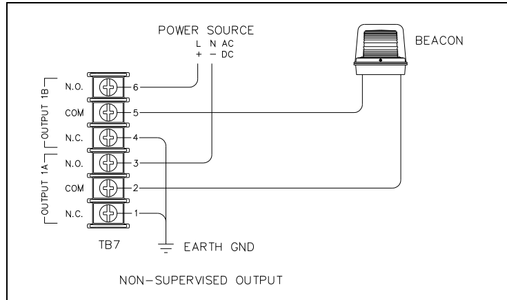
Figure 13. Non-supervised Output with the VLC or SmartSeries® Option
