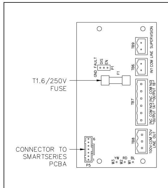
Figure 12. No. 69628 Series RTU & SmartSeries® 70V/100V Speaker Line Monitor PCBA
