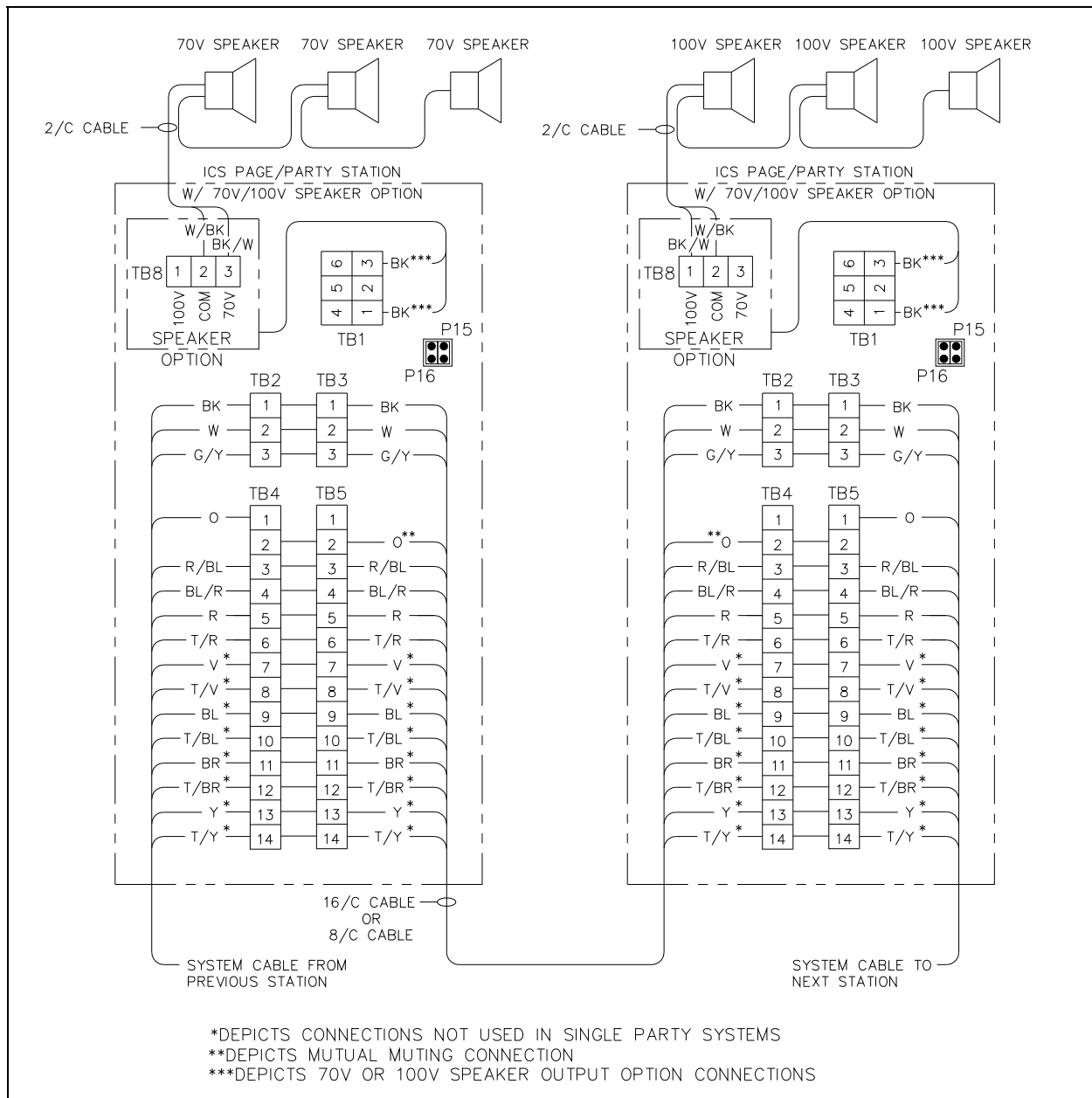
Figure 18. 70 V/100 V Speaker Connections
