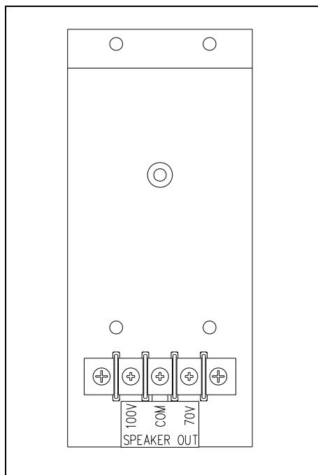
Figure 16. Standard Station 70V/100V Speaker Output Assembly
