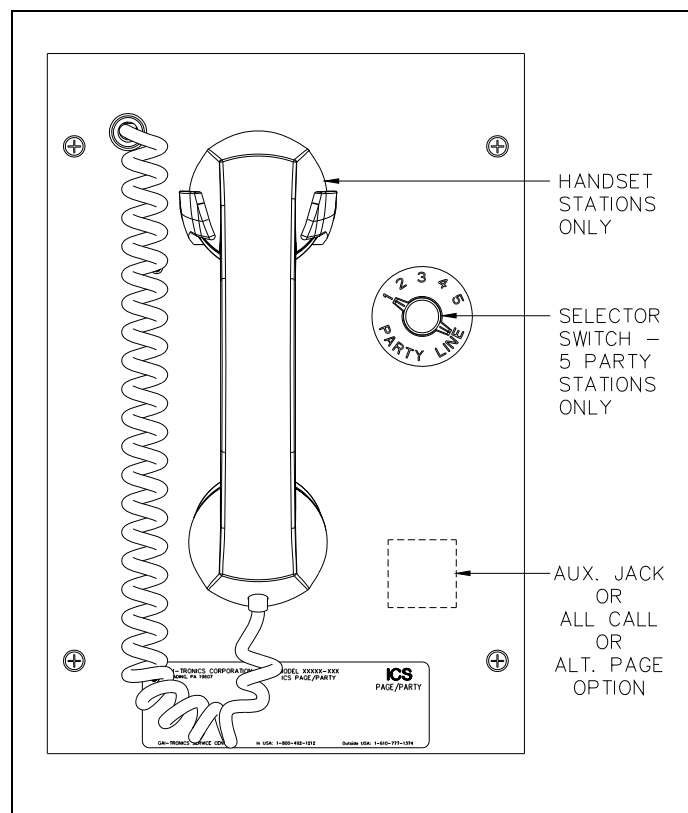
Figure 1. ICS Station Front Panel with all options
