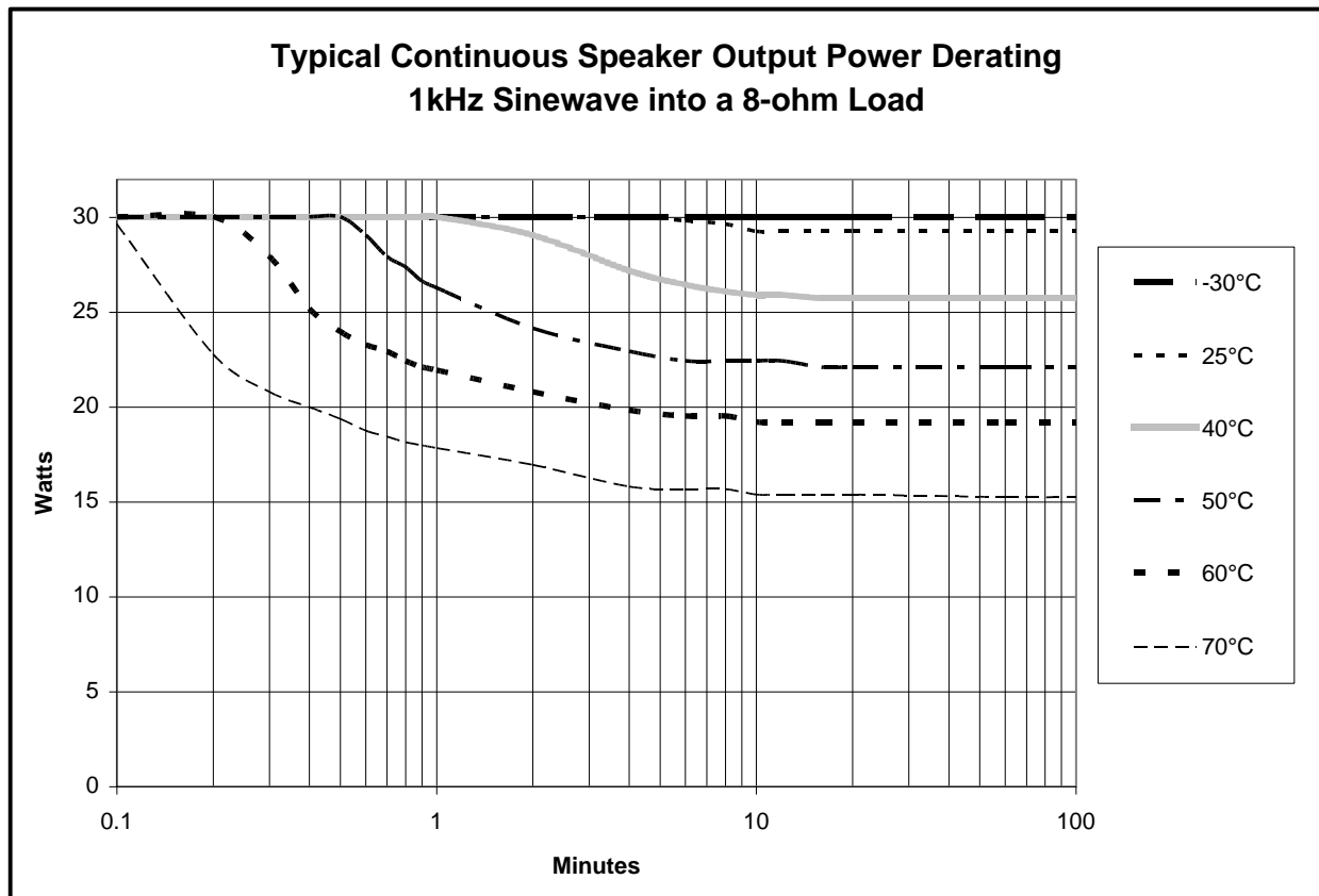
Figure 22. Typical Continuous Speaker Output Power Derating
