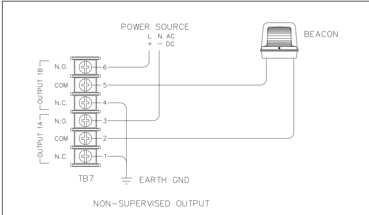
Figure 13. Non-supervised Output with the VLC or SmartSeries® Option
