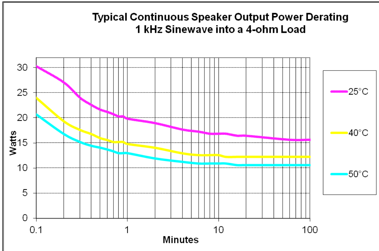
Figure 23. Typical Continuous Speaker Output Power Derating 1 kHz Sine Wave into a 4-ohm Load
