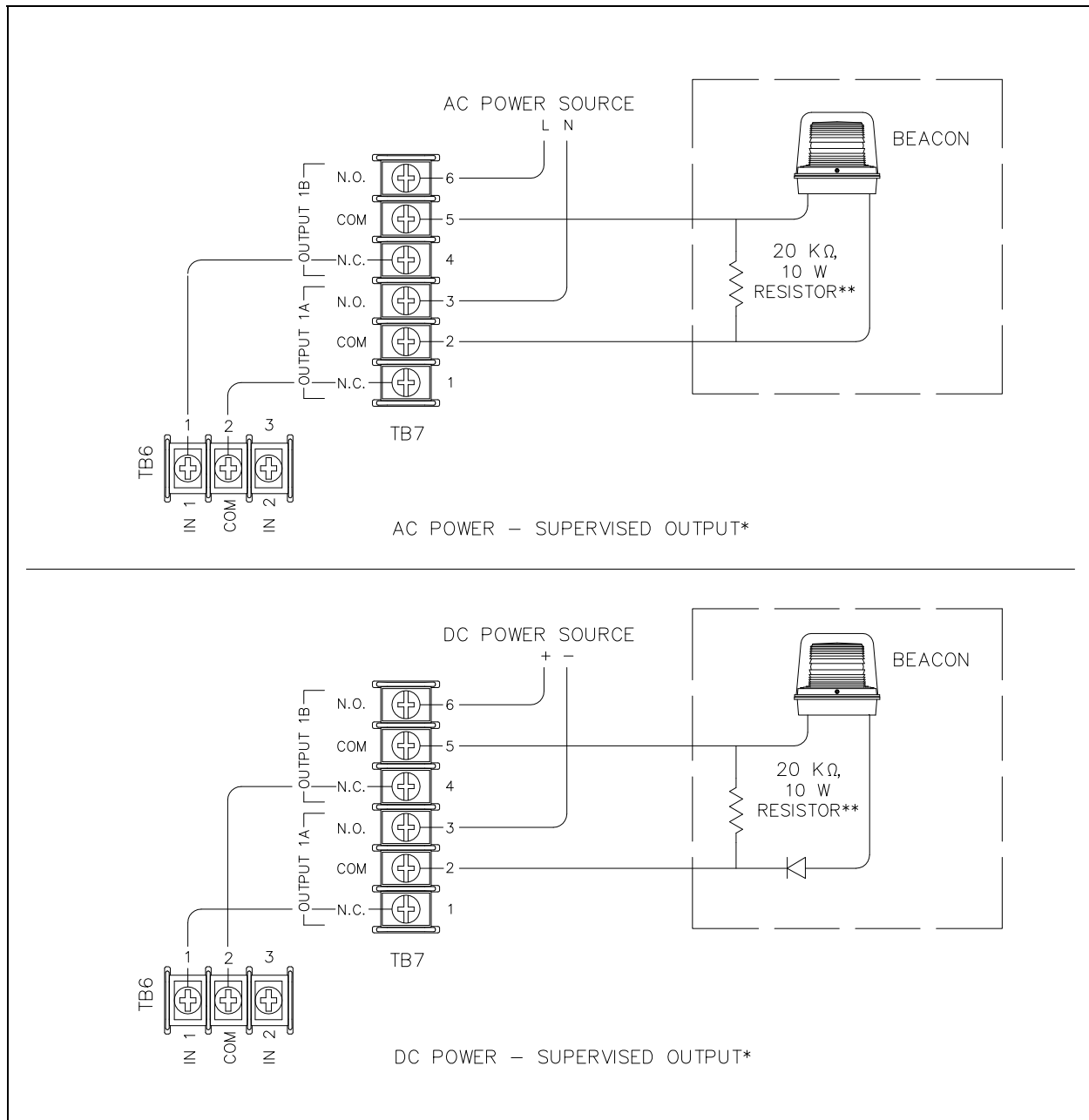
Figure 14. Supervised Output Wiring with SmartSeries® Option
