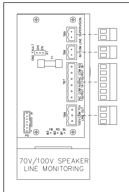
Figure 17. SmartSeries® Station 70V/100V Speaker Line Monitor Assembly
