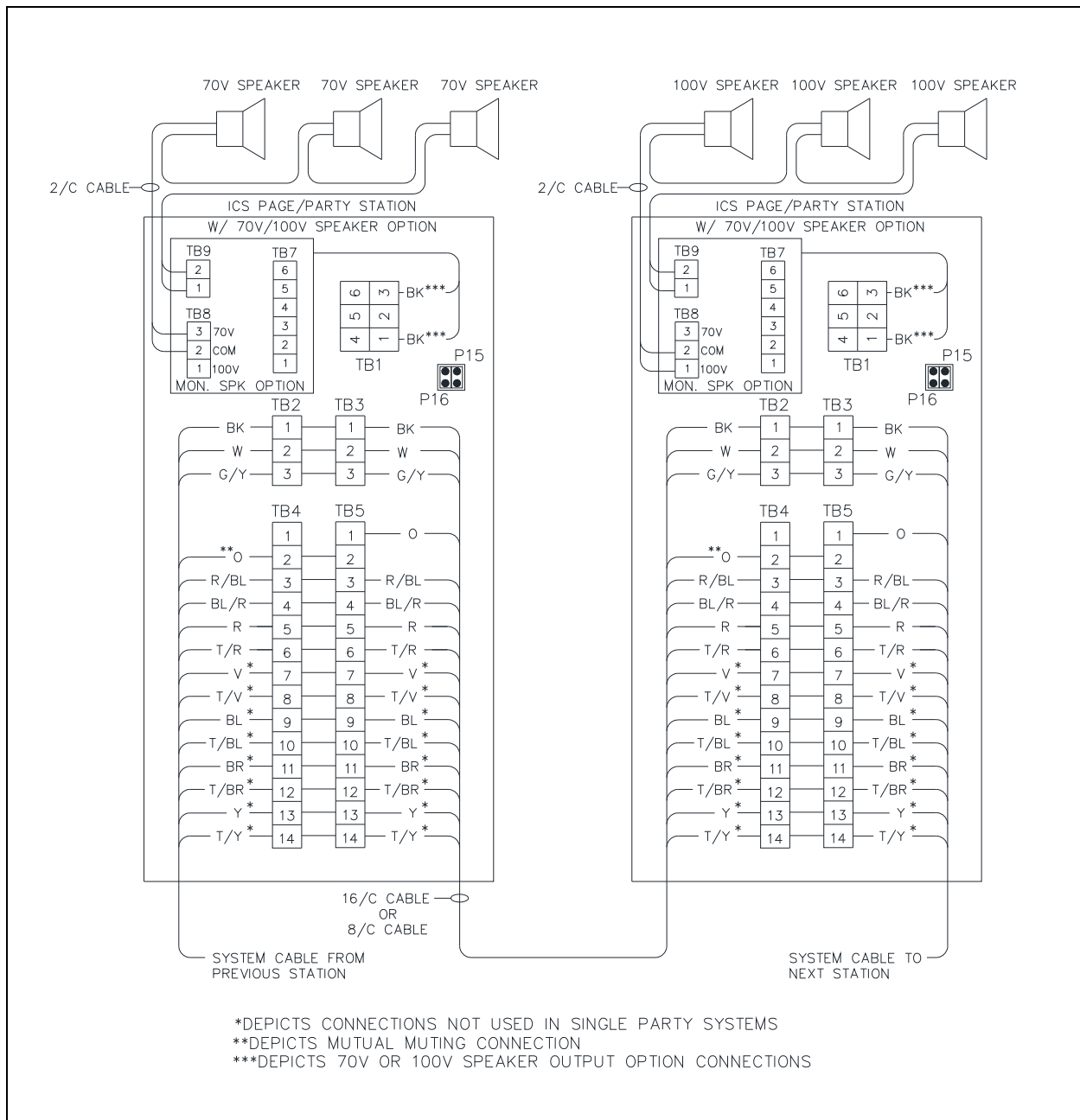
Figure 19. 70V/100V Monitored Speaker Connections
