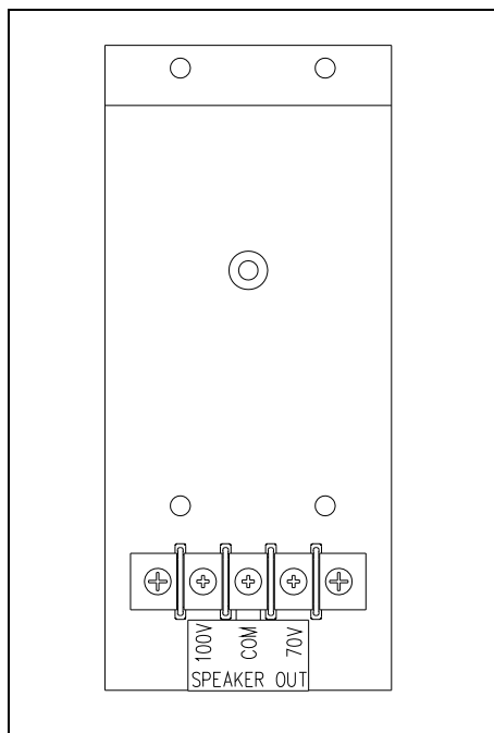
Figure 16. Standard Station 70V/100V Speaker Output Assembly
