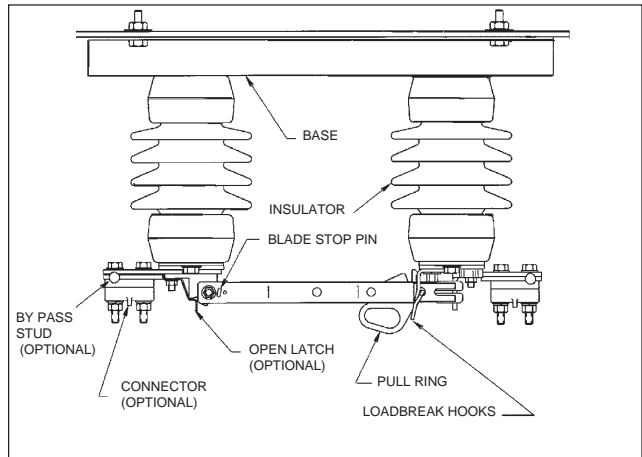
Figure 1 — Inverted-Underhung
