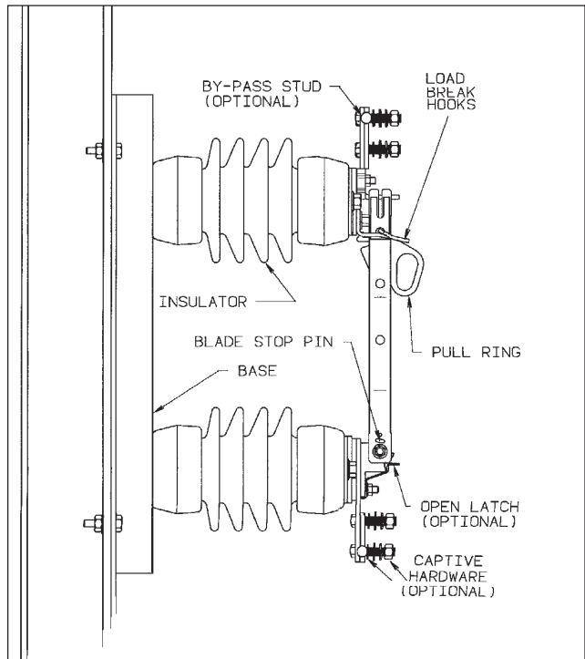
Figure 2 — Vertical Mount
