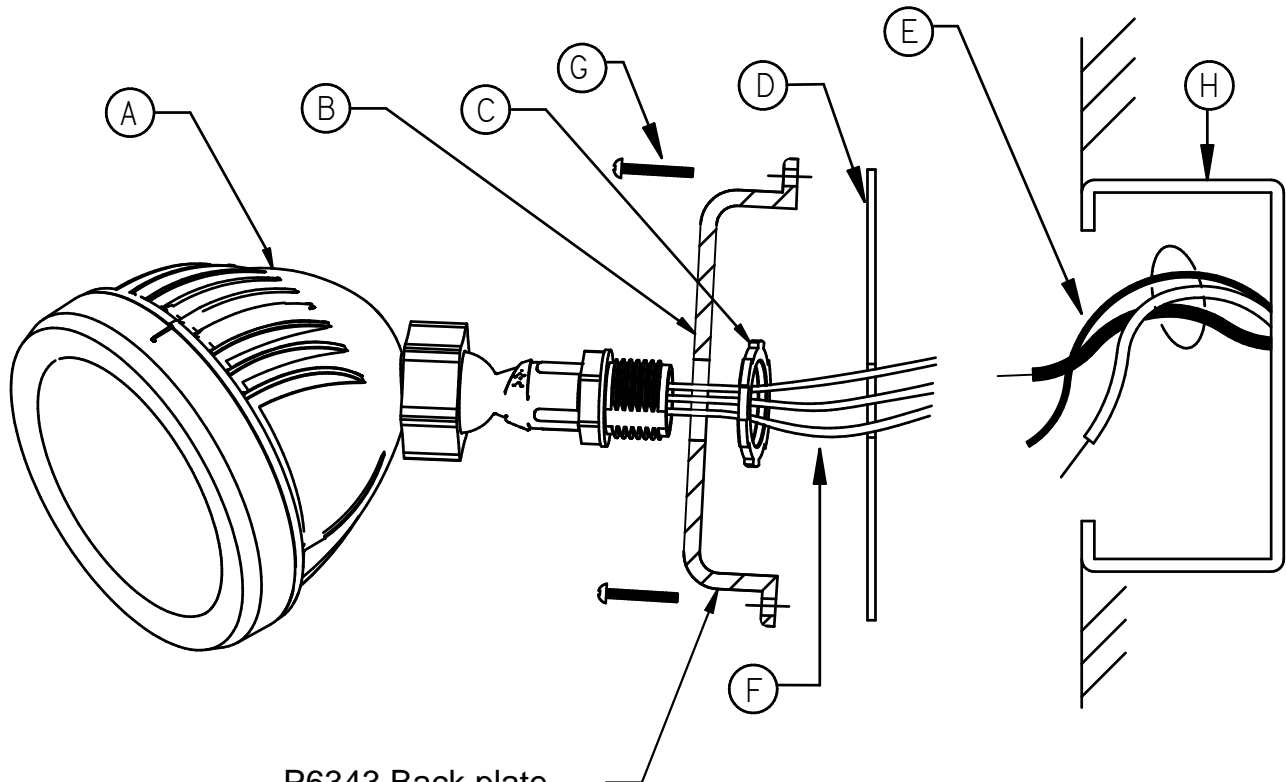
P6343 Back plate P6343 plaque arrière P6343 placa trasera
