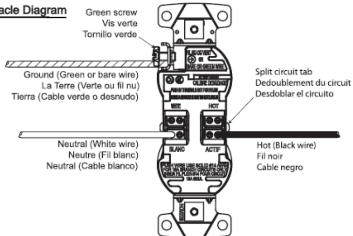
8-Hole Push Wire Receptacle Diagram
