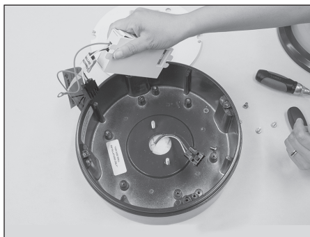
7. Remove ballast assembly and discard.
