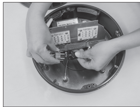
9. Connect LED upgrade driver to line voltage.
