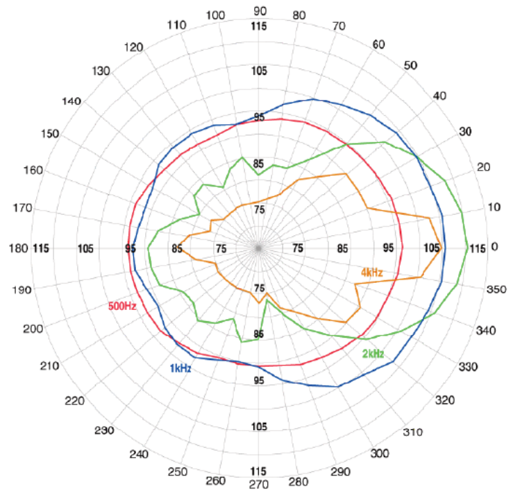
Polar Plot
