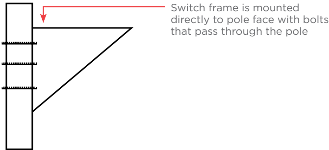
Detail F (Thru-Bolt)
