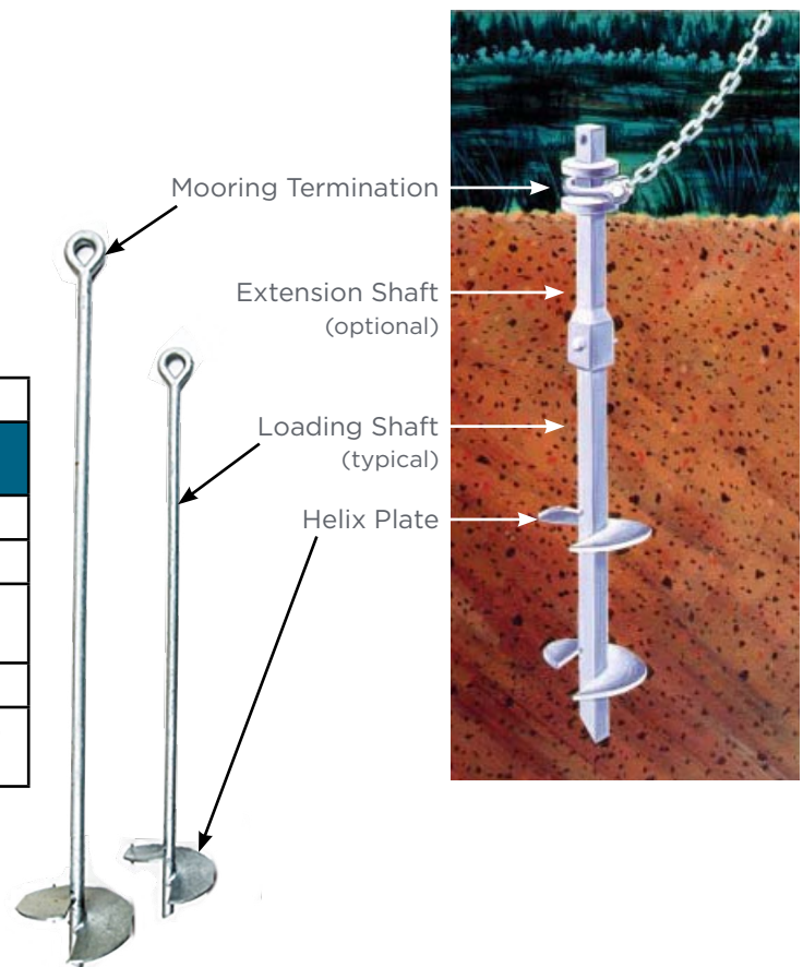
Square Shaft Anchor
